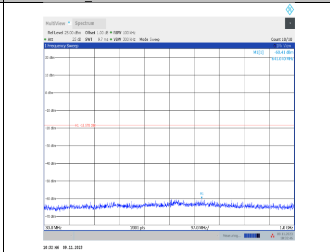
BLE_1M-Ant0-2480-30~1000-PASS
