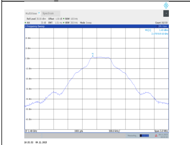
BLE_1M-Ant0-2480-0~Reference-PASS
