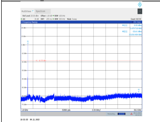
BLE_1M-Ant0-2480-1000~26500-PASS
