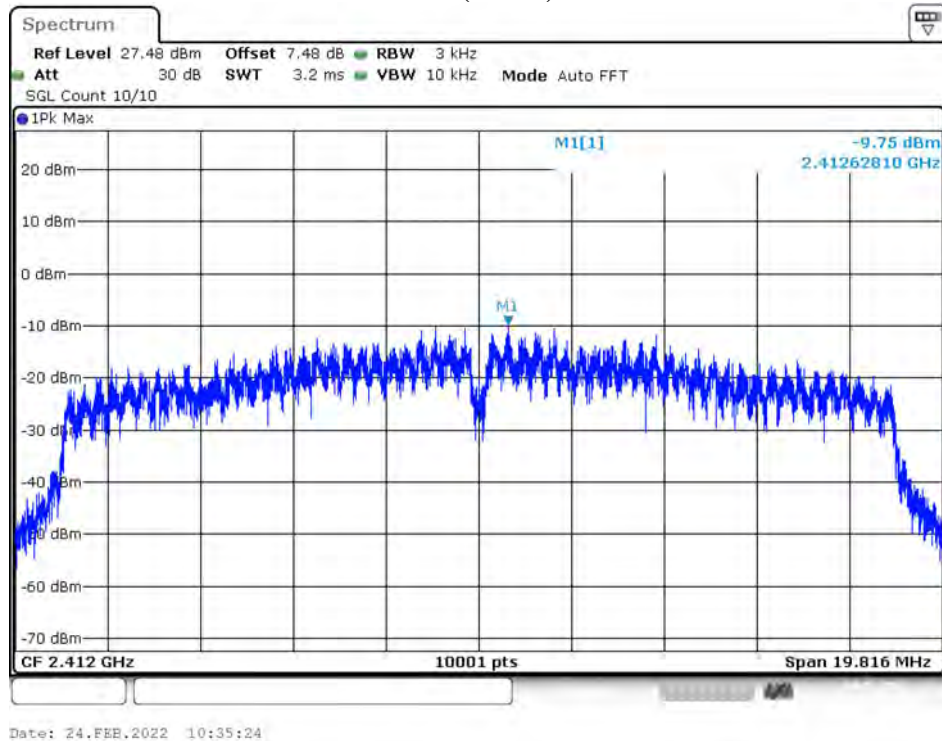
PSD NVNT 802.11n(HT20) 2412MHz Ant1
