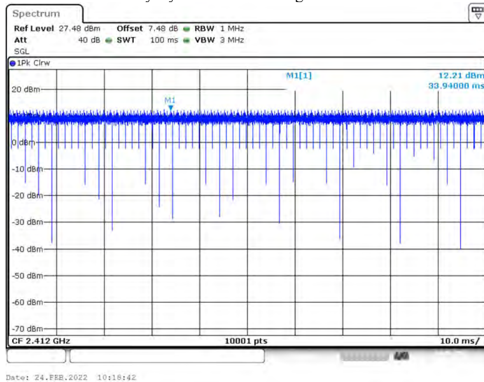
Duty Cycle NVNT 802.11g 2412MHz
