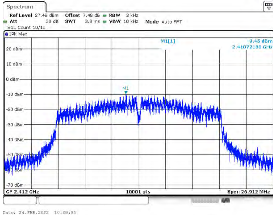
PSD NVNT 802.11g 2412MHz Ant1
