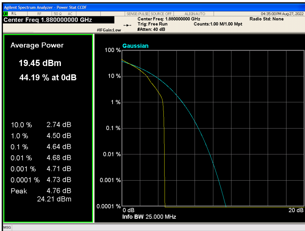
Band2 QAM16 BW=20MHz Channel=18900 RB Size=1 Position=#0
