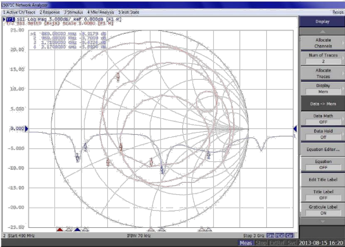
RF1: Main circuit matching - 10nH
