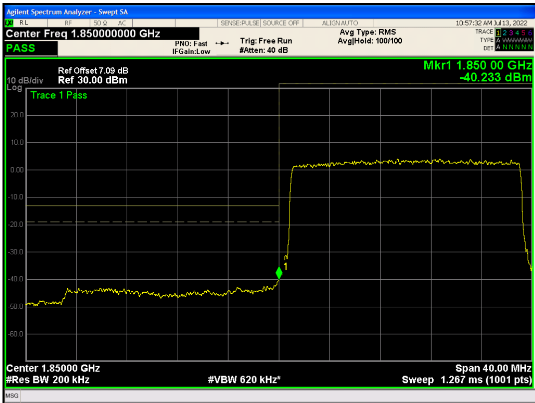
Band2 QAM16 BW=20MHz Channel=18700 RB Size=100 Position=#0
