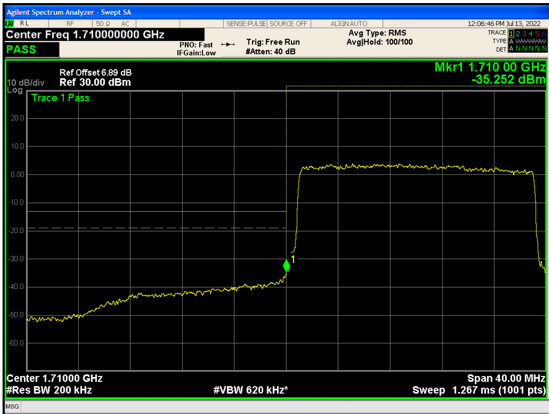
Band4 QAM16 BW=20MHz Channel=20050 RB Size=100 Position=#0
