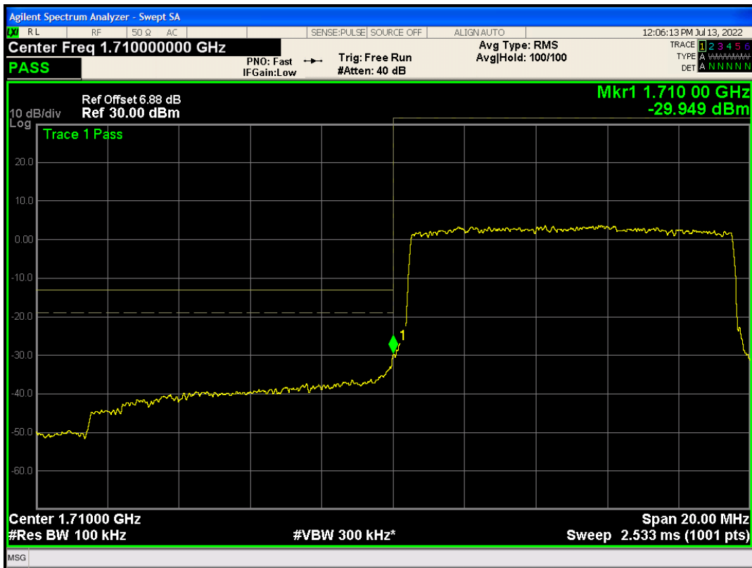
Band4 QAM16 BW=10MHz Channel=20000 RB Size=50 Position=#0
