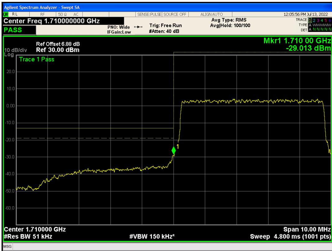
Band4 QAM16 BW=5MHz Channel=19975 RB Size=25 Position=#0
