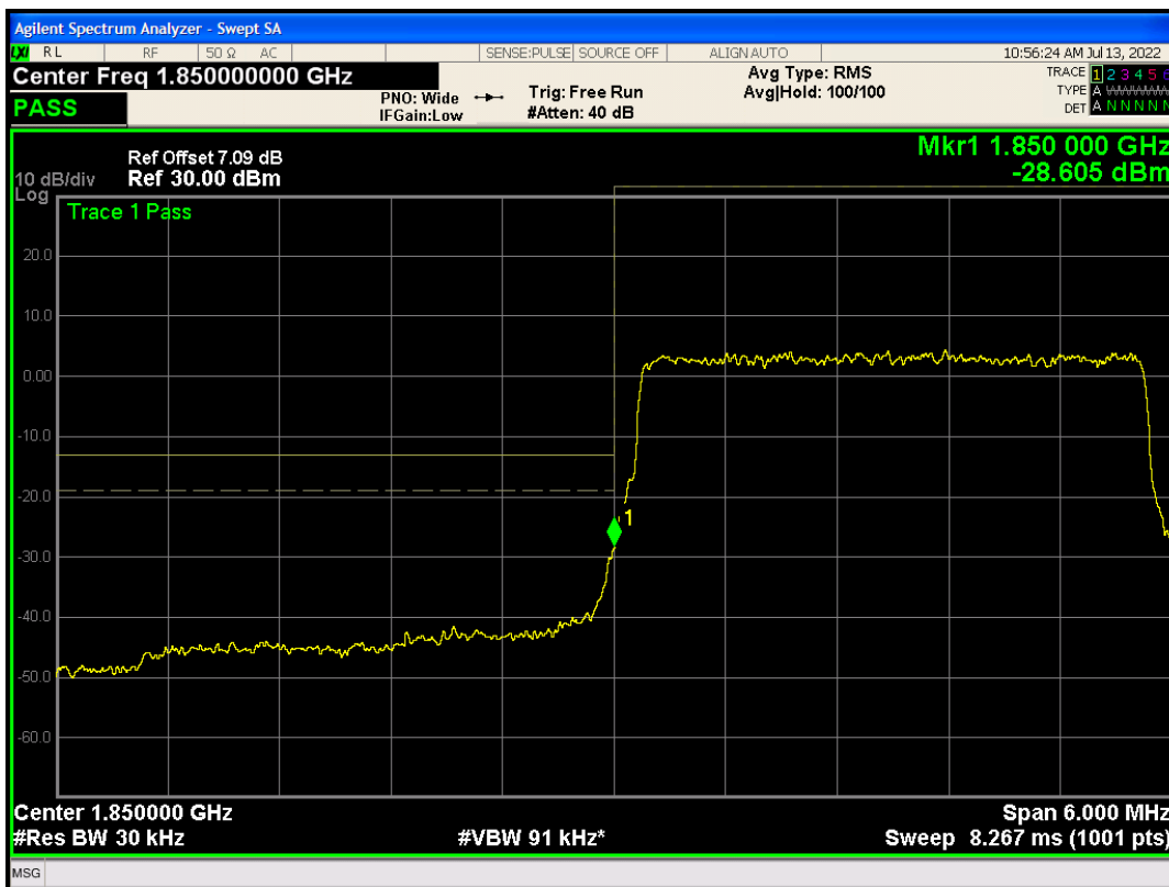
Band2 QAM16 BW=3MHz Channel=18615 RB Size=15 Position=#0
