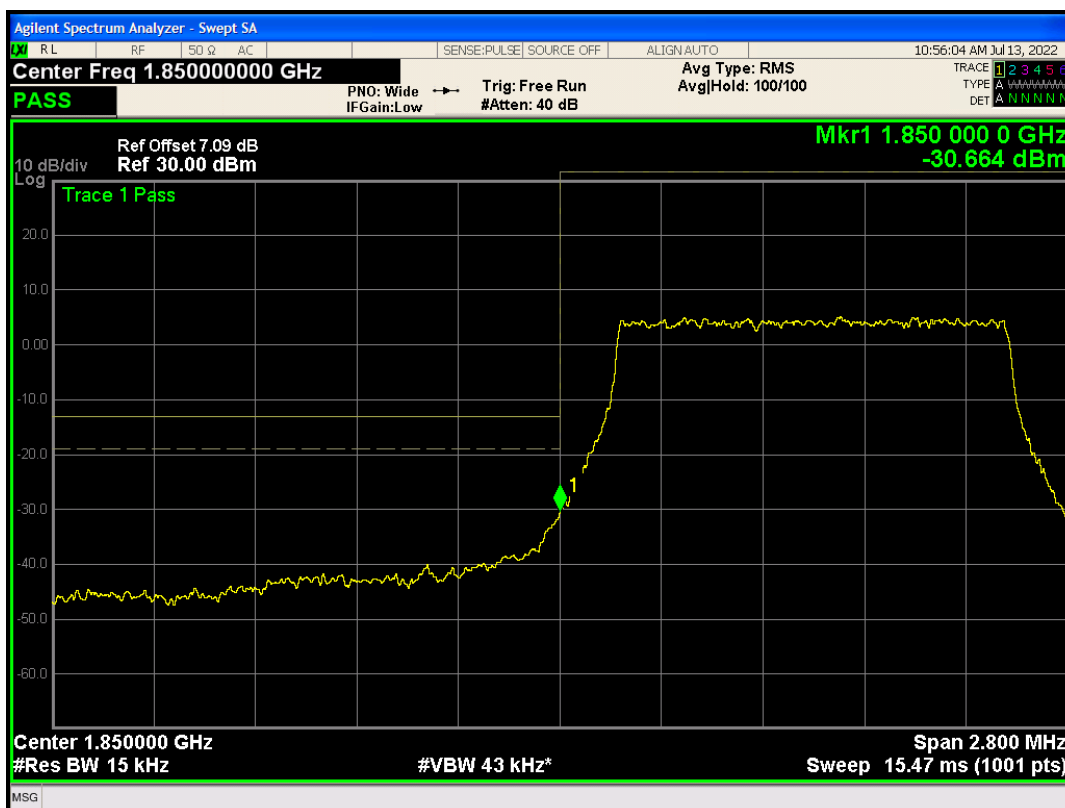
Band2 QAM16 BW=1.4MHz Channel=18607 RB Size=6 Position=#0
