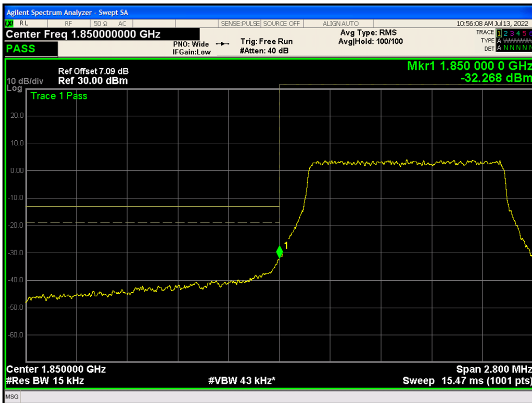
Band2 QPSK BW=1.4MHz Channel=19193 RB Size=6 Position=#0
