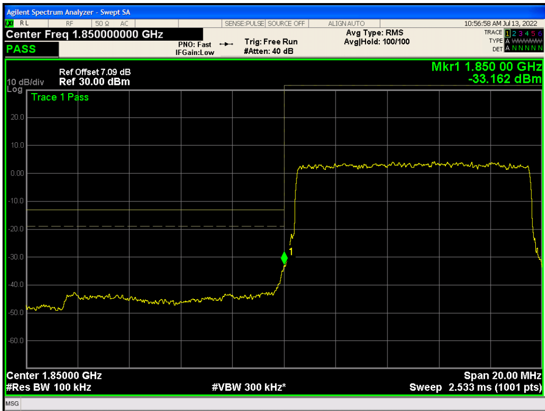
Band2 QAM16 BW=10MHz Channel=18650 RB Size=50 Position=#0
