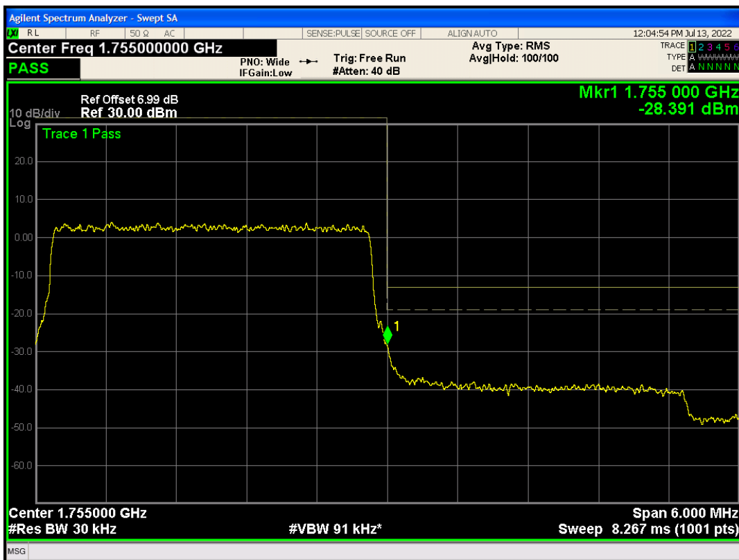
Band4 QAM16 BW=3MHz Channel=20385 RB Size=15 Position=#0
