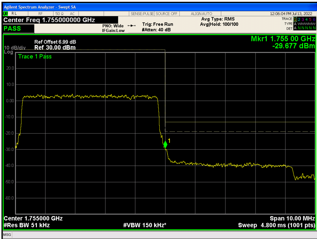
Band4 QAM16 BW=5MHz Channel=20375 RB Size=25 Position=#0
