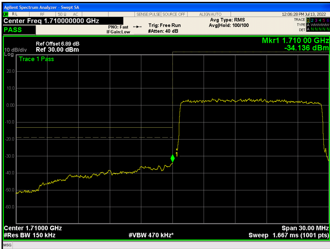
Band4 QAM16 BW=15MHz Channel=20025 RB Size=75 Position=#0
