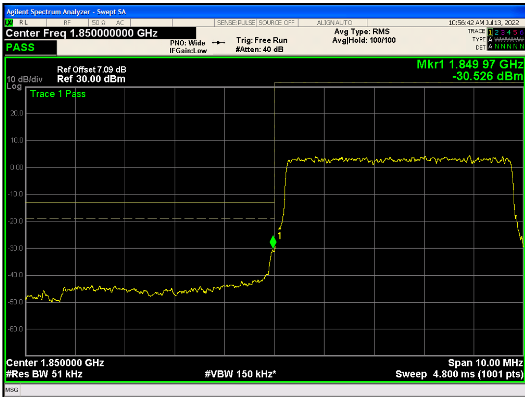
Band2 QAM16 BW=5MHz Channel=18625 RB Size=25 Position=#0
