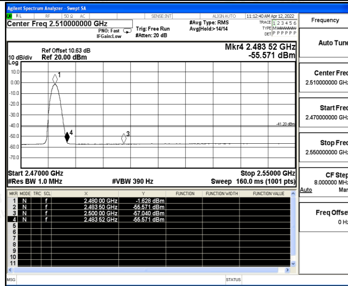
2DH5_Ant_High_2480_Peak
