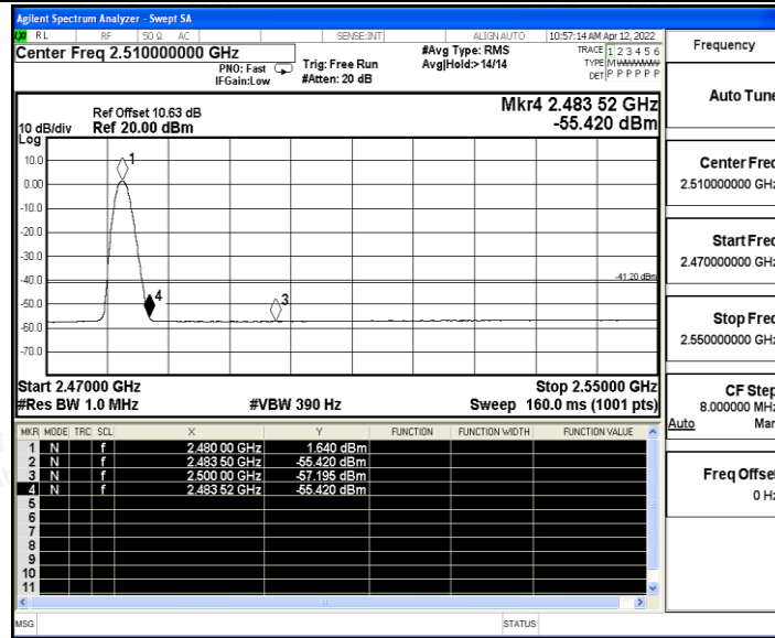
DH5_Ant_High_2480_Peak
