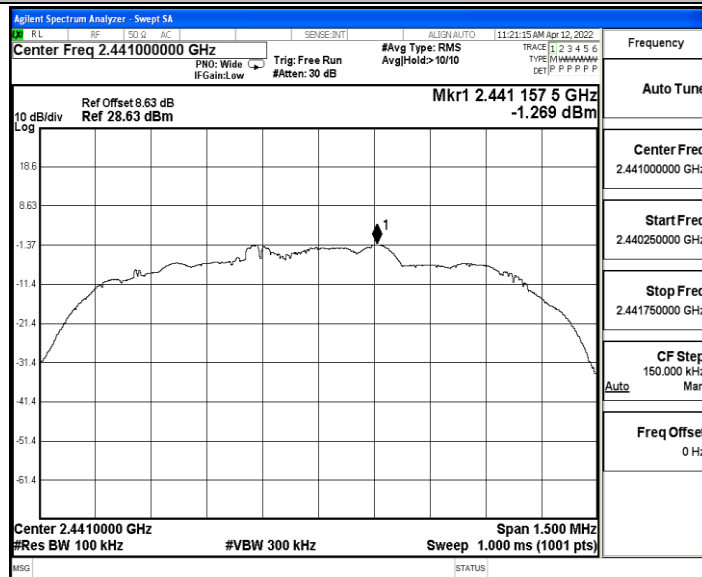
3DH5_Ant_2441_30~1000
