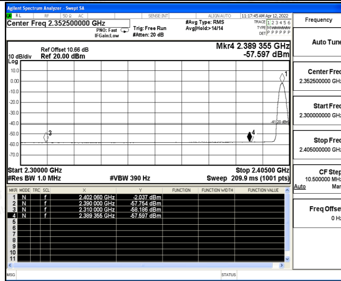
3DH5_Ant_Low_2402_Peak
