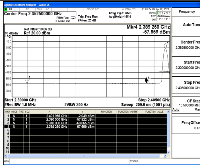
2DH5_Ant_Low_2402_Peak
