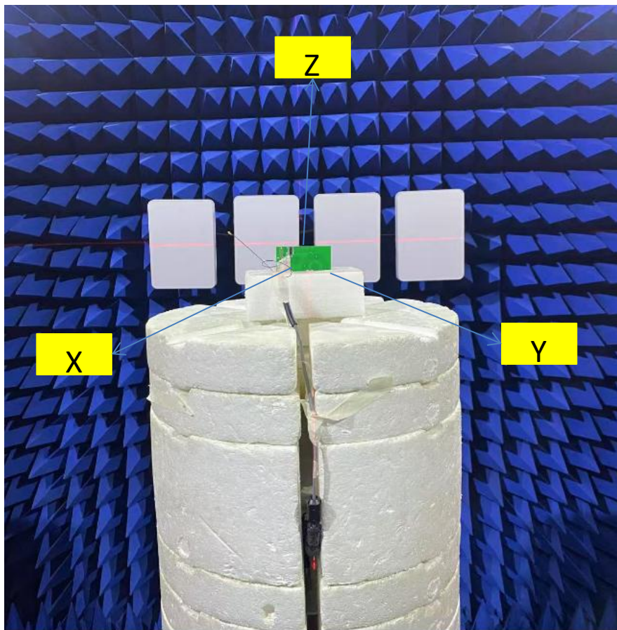
Testing environment
