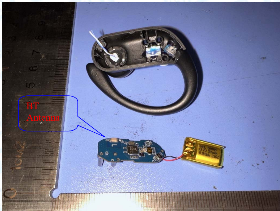
Photo 12 Internal EUT
