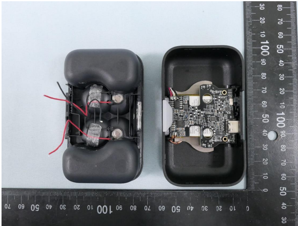
(20) EUT Photo (Charging box)
