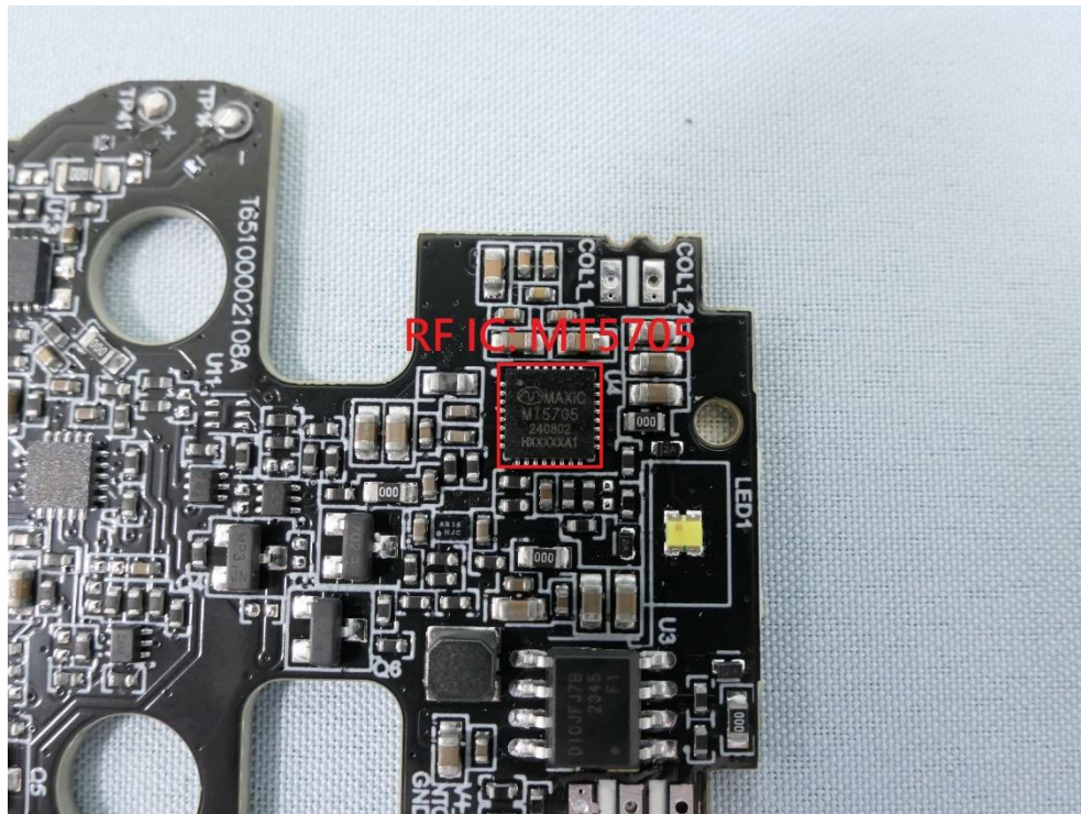
(27) EUT Photo (Charging box)
