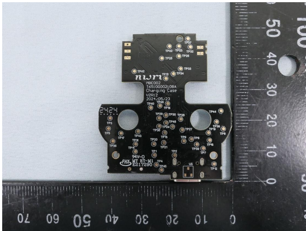
(25) EUT Photo (Charging box)
