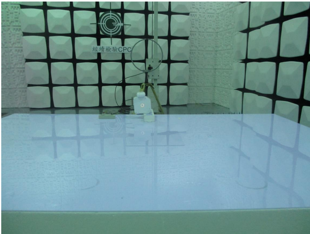
Setup Photo FCC ID: 2A57Q-RN01
