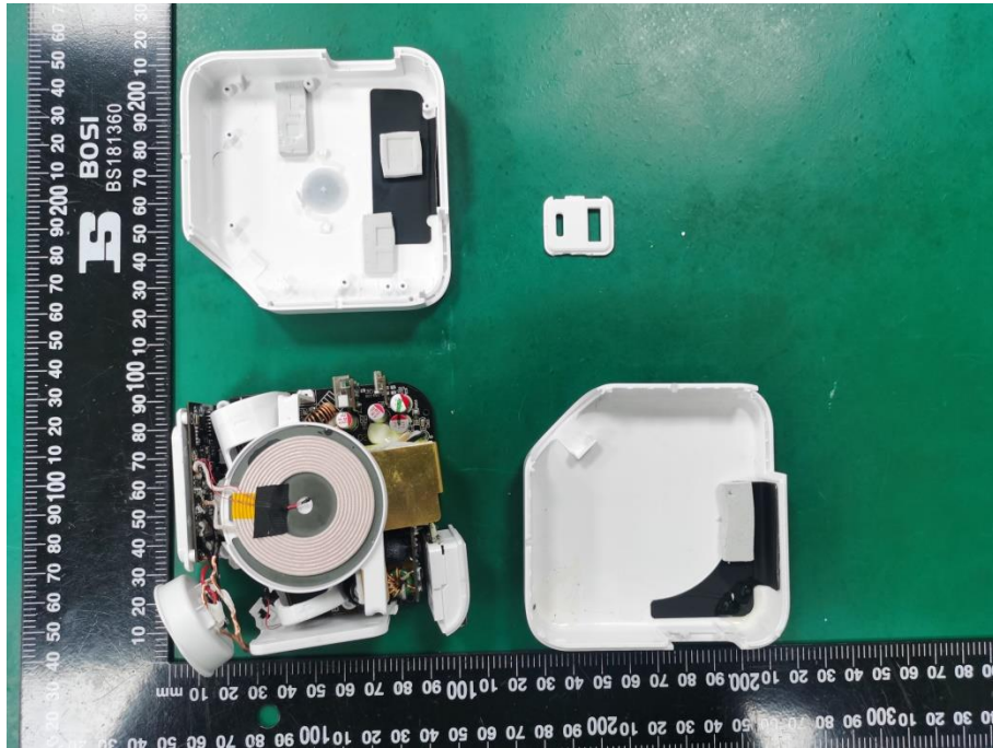
Internal Photo FCC ID: 2A57Q-RN01
