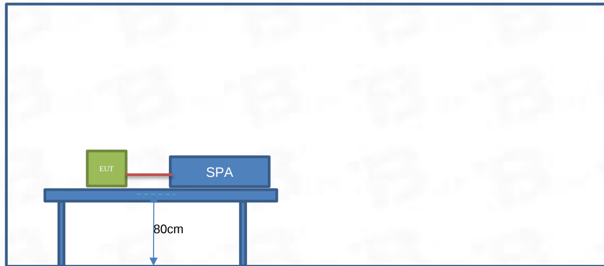
Radiation Test (9k - 30MHz)
