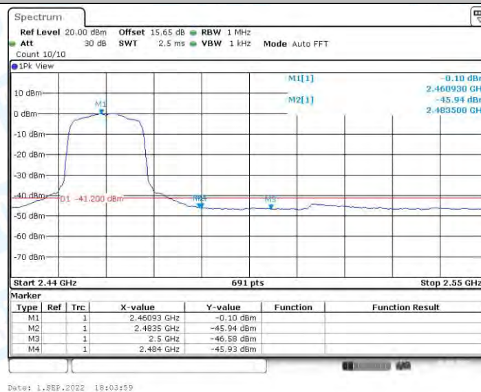
11G-CDD_Ant2_High_2462_Peak
