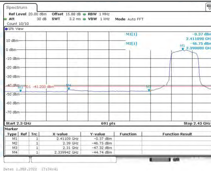
11G-CDD_Ant1_Low_2412_Peak
