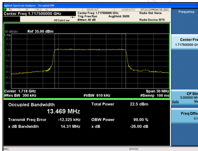
Band4-15MHz-QPSK-20175-75RB#0
