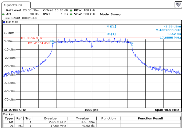
n20_2462MHz_Chain 0 17.680MHz
