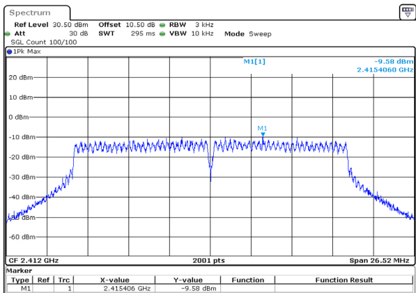
n20_2412MHz_Chain 0 -9.58dBm/3kHz
