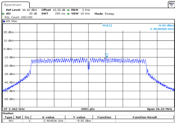
n20_2462MHz_Chain 0 -9.95dBm/3kHz
