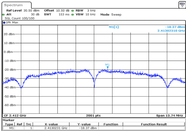
b_2412MHz_Chain 0 -18.37dBm/3kHz
