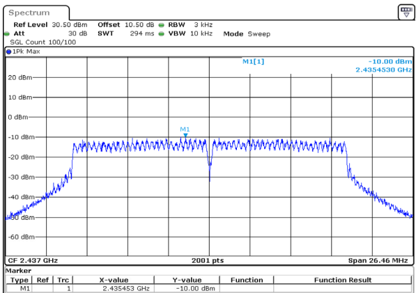
n20_2437MHz_Chain 0 -10.00dBm/3kHz
