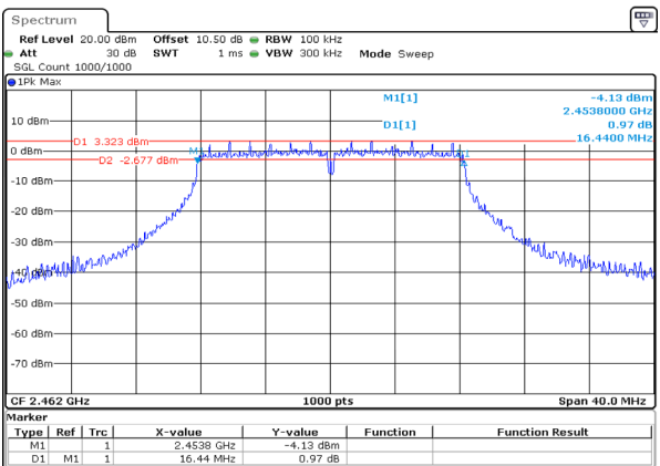
g_2462MHz_Chain 0 16.440MHz
