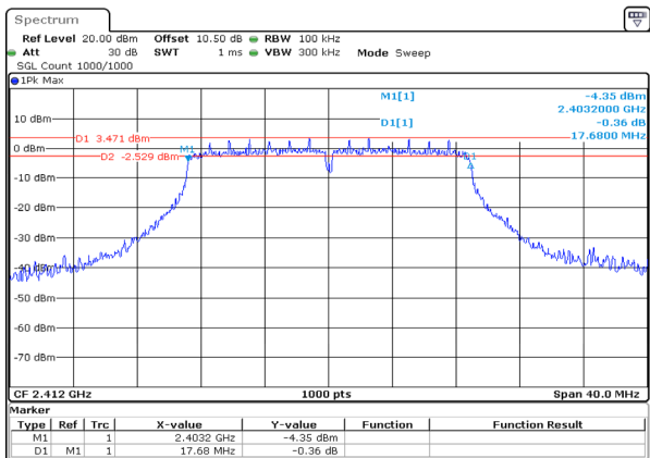
n20_2412MHz_Chain 0 17.680MHz
