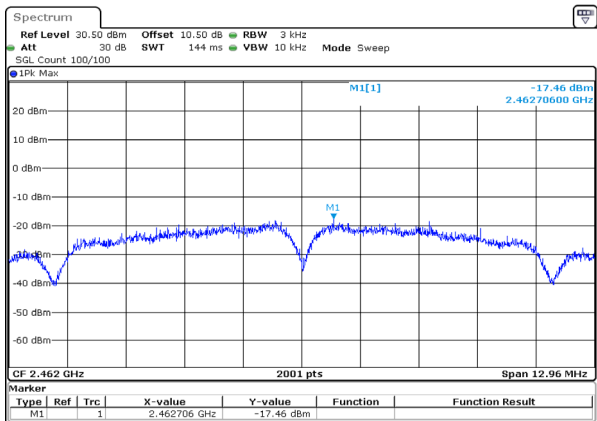
b_2462MHz_Chain 0 -17.46dBm/3kHz
