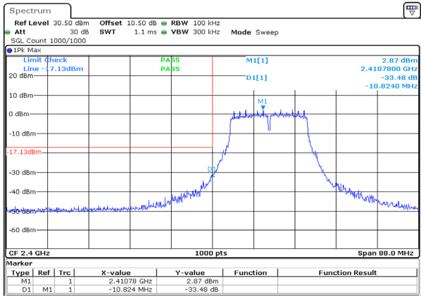
g_2412MHz_Chain 0
