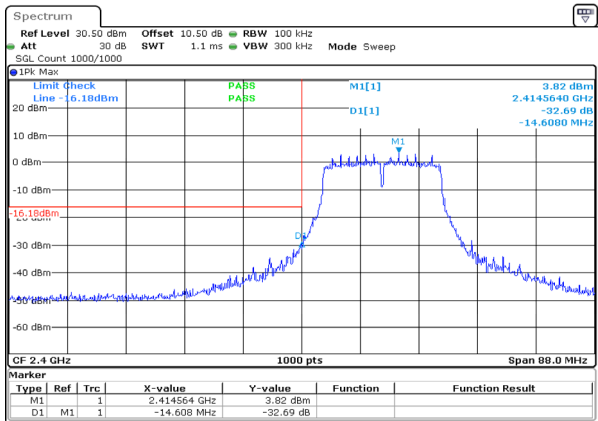
n20_2412MHz_Chain 0
