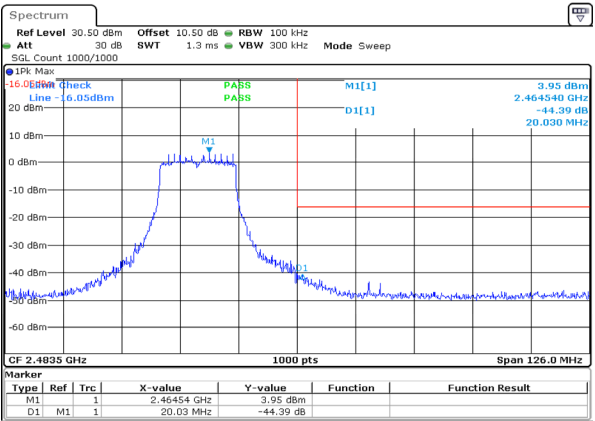
g_2462MHz_Chain 0
