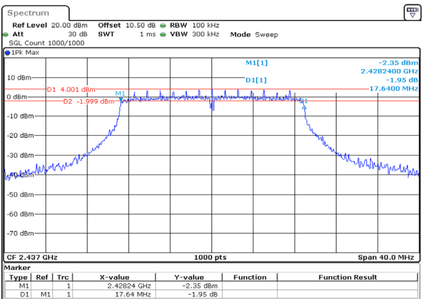
n20_2437MHz_Chain 0 17.640MHz
