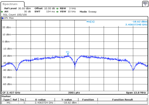
b_2437MHz_Chain 0 -18.62dBm/3kHz
