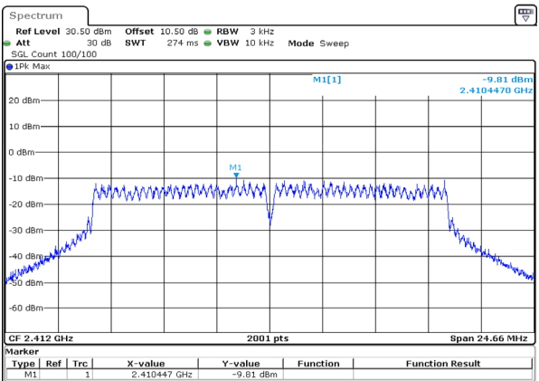
g_2412MHz_Chain 0 -9.81dBm/3kHz
