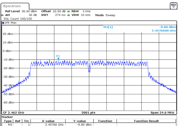
g_2462MHz_Chain 0 -9.80dBm/3kHz
