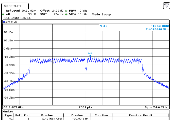
g_2437MHz_Chain 0 -10.03dBm/3kHz
