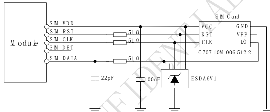
Figure 31: Reference circuit of the 6-pin SIM card holder
