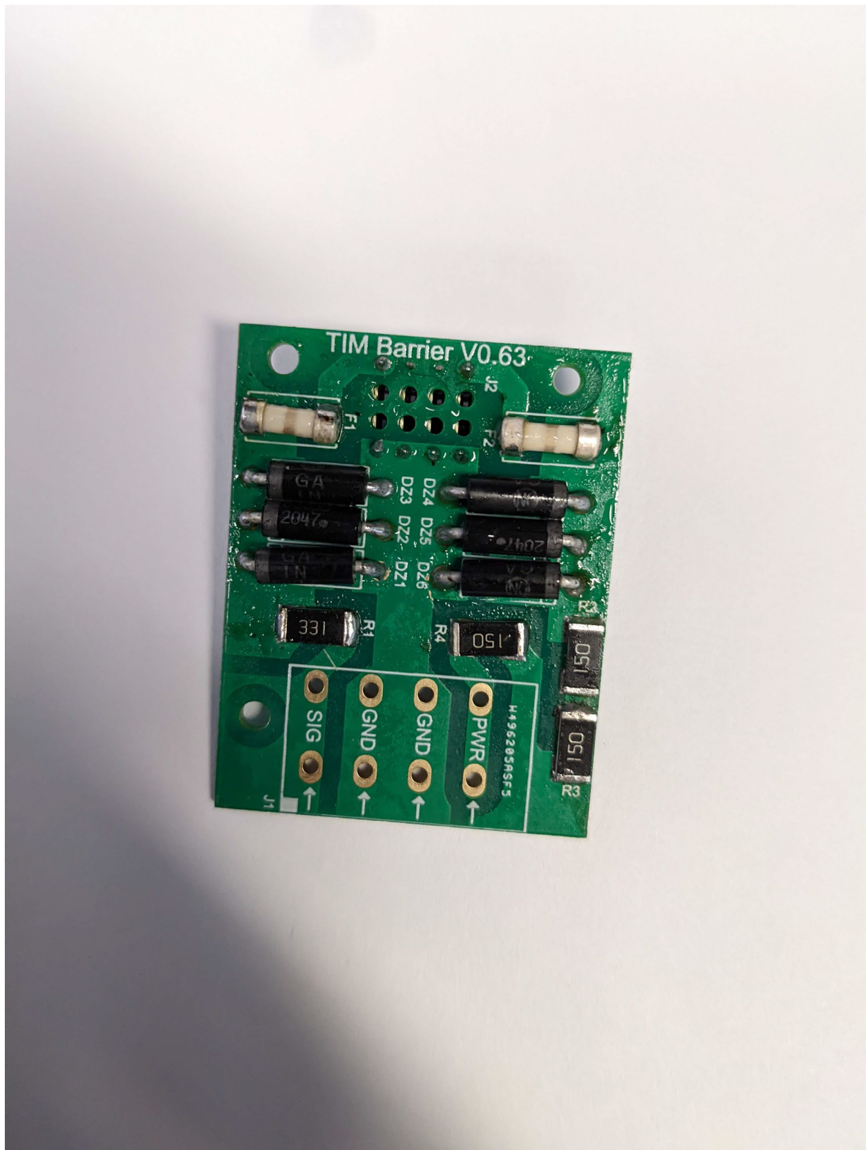
TIM PLUS BARRIER BOARD – TOP VIEW
