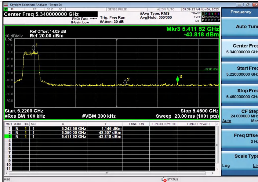
11N20SISO-Ant2-5240-PASS
