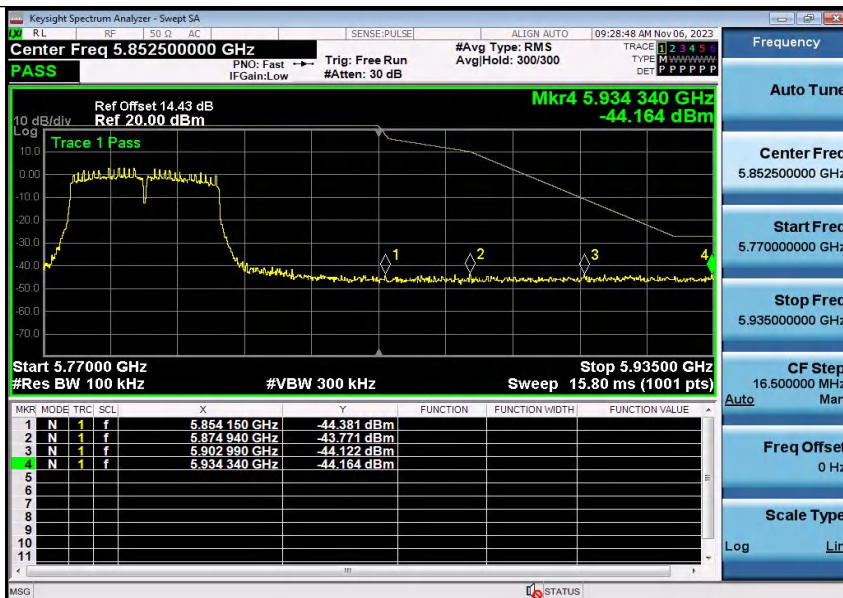
11AC40SISO-Ant1-5795-PASS
