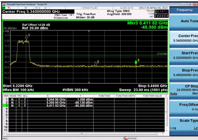
11N20SISO-Ant1-5240-PASS
