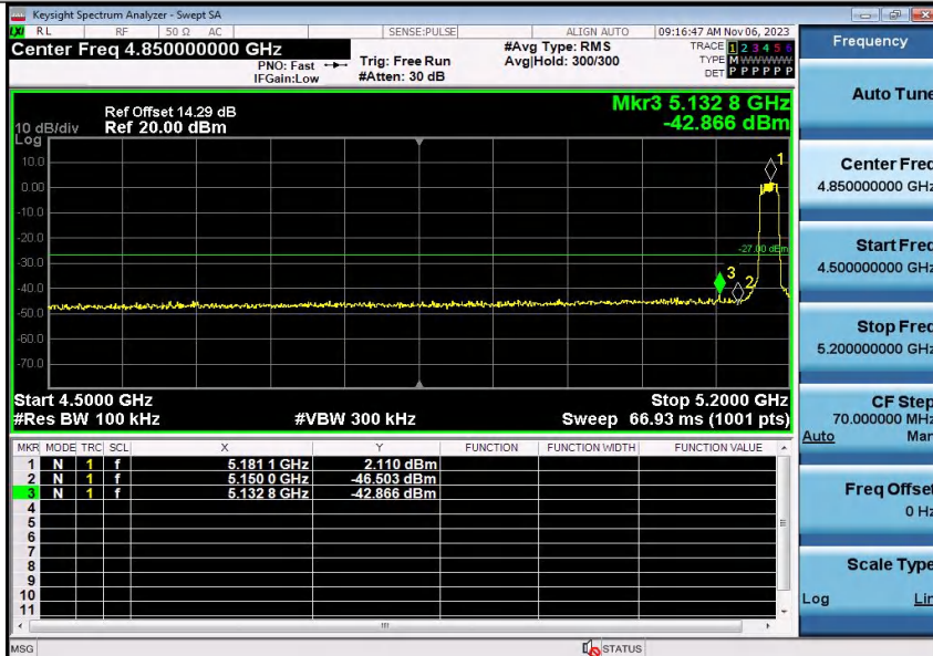
11N20SISO-Ant1-5180-PASS
