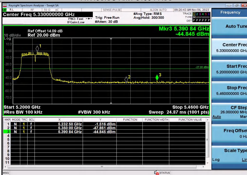
11N40SISO-Ant1-5230-PASS
