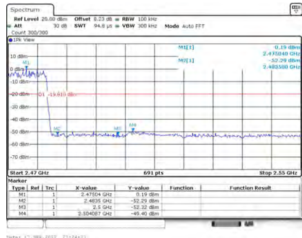
3DH5(2480)-Hopping on
