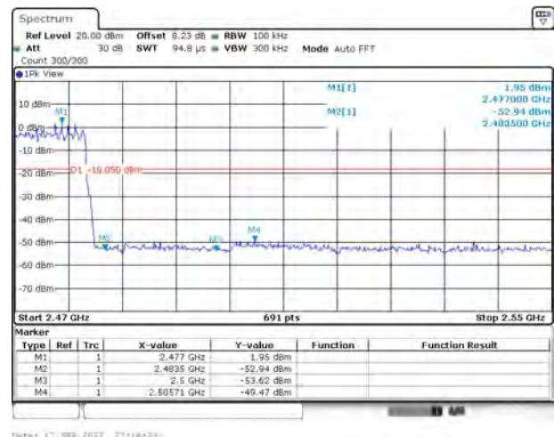
3DH5(2480)-Hopping on
