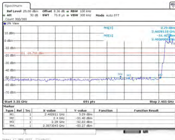
3DH5(2402)-Hopping on
