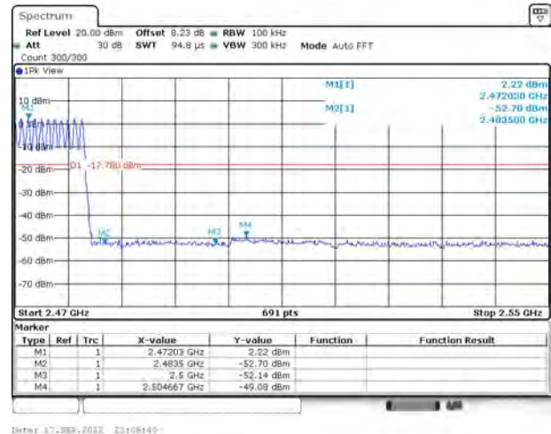
2DH5(2480)-Hopping on
