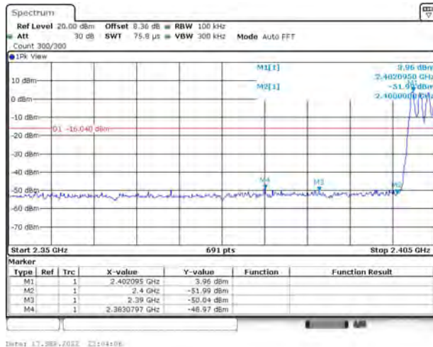
2DH5(2402)-Hopping on
