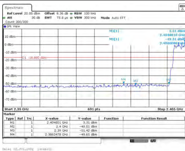
3DH5(2402)-Hopping on
