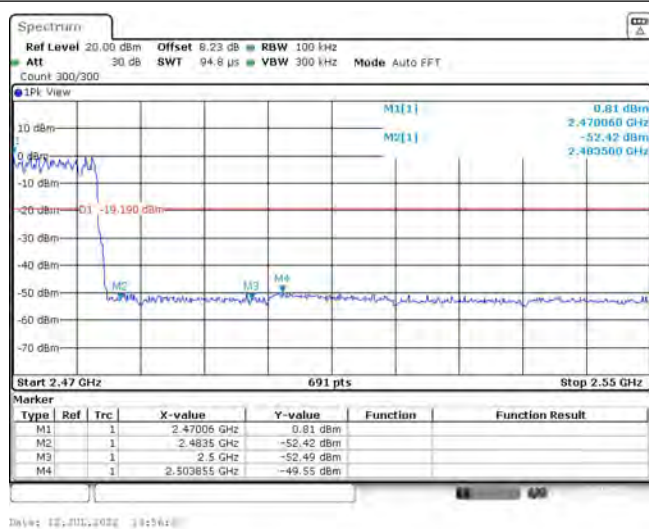
3DH5(2480)-Hopping on
