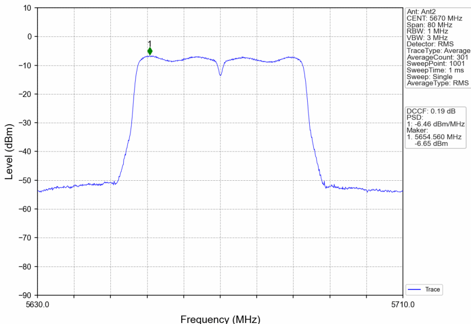
802.11n(HT40)_HCH_5670MHz_MIMO_NTNV
