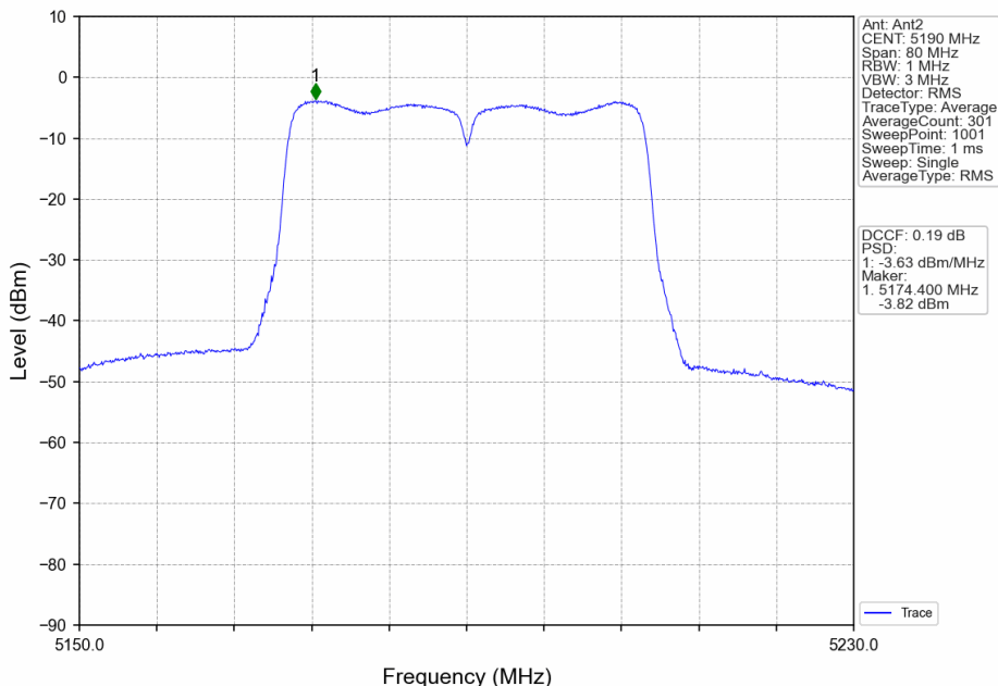
802.11n(HT40)_LCH_5190MHz_MIMO_NTNV
