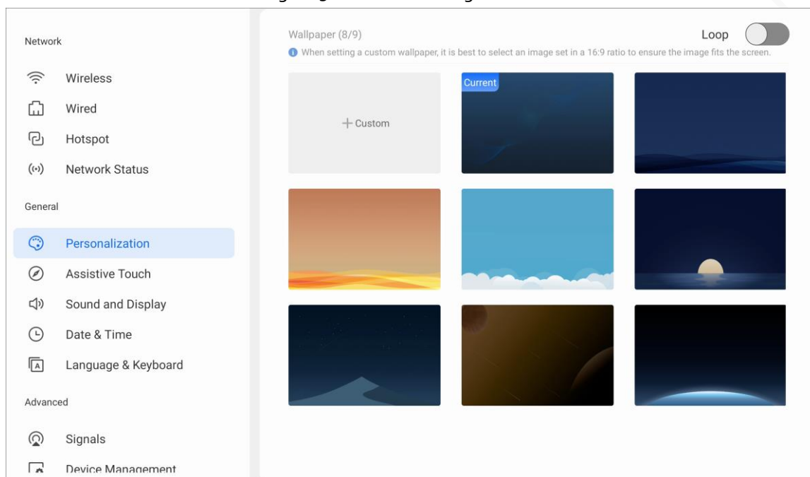
Figure 3-8 General settings
