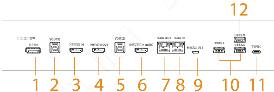
Figure 1-10 Ports on the side of the rear panel
