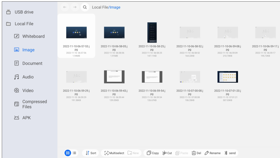
Figure 3-5 File management
