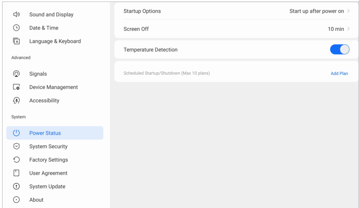
Figure 3-10 System parameters
