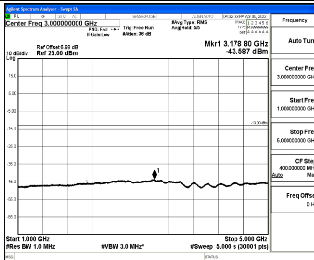
Band12-10MHz-16QAM-23095-1-0-Low-1000-5000--43.59-PASS
