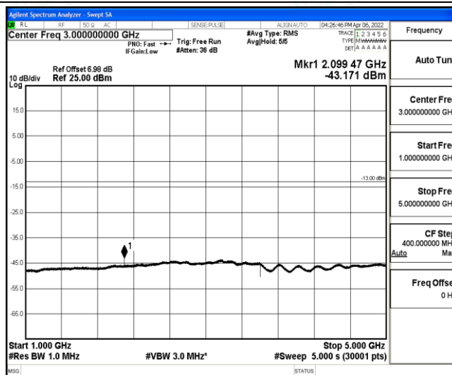
Band12-10MHz-QPSK-23060-1-0-Low-1000-5000--43.17-PASS
