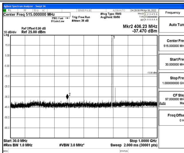
Band12-10MHz-16QAM-23060-1-0-Low-30-1000--37.47-PASS
