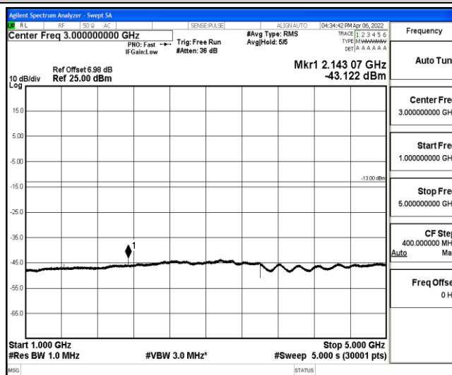
Band12-10MHz-QPSK-23130-1-0-High-1000-5000--43.12-PASS
