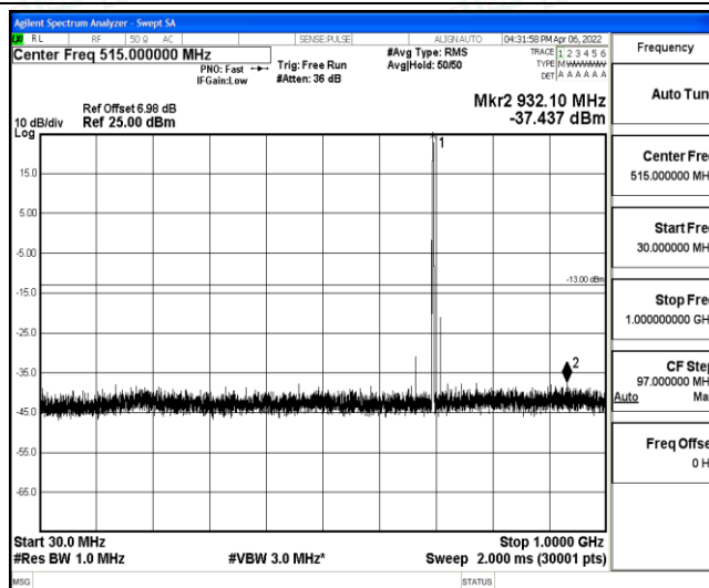
Band12-10MHz-16QAM-23095-1-0-Low-30-1000--37.44-PASS
