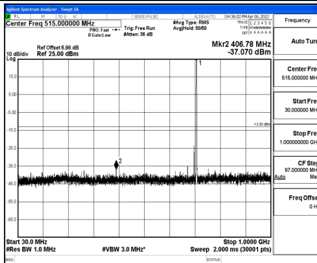
Band12-10MHz-16QAM-23130-1-0-High-30-1000--37.07-PASS
