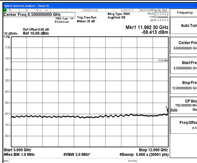
Band12-10MHz-QPSK-23060-1-0-Low-5000-12000--59.41-PASS
