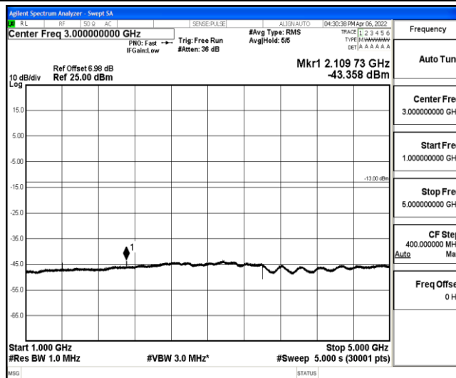
Band12-10MHz-QPSK-23095-1-0-Low-1000-5000--43.36-PASS
