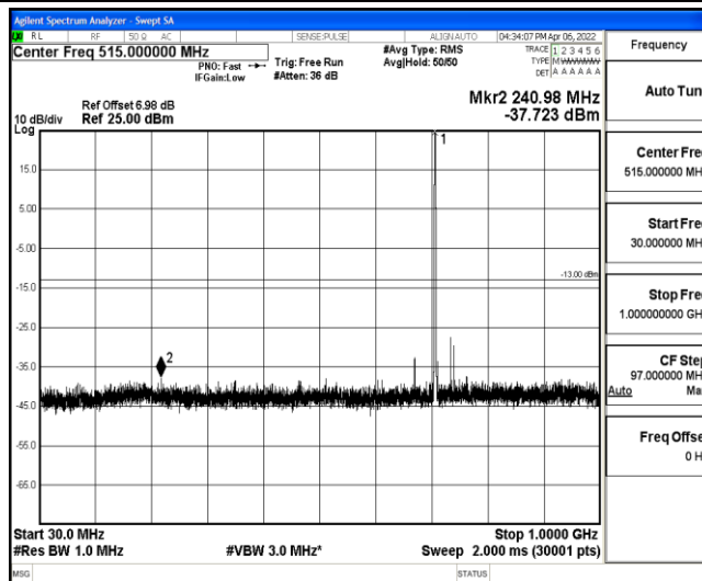
Band12-10MHz-QPSK-23130-1-0-High-30-1000--37.72-PASS
