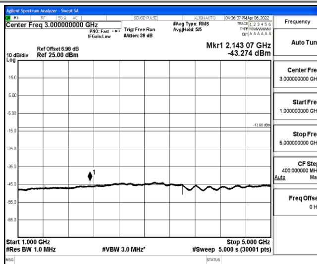
Band12-10MHz-16QAM-23130-1-0-High-1000-5000--43.27-PASS
