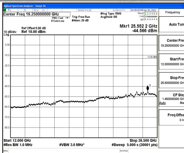
Band12-5MHz-16QAM-23095-1-0-Low-12000-26500--44.57-PASS
