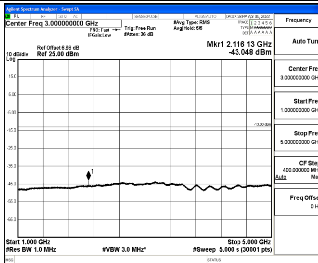
Band12-5MHz-16QAM-23095-1-0-Low-1000-5000--43.05-PASS
