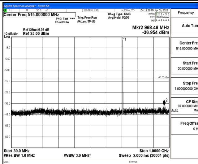
Band12-5MHz-16QAM-23155-1-0-High-30-1000--36.95-PASS
