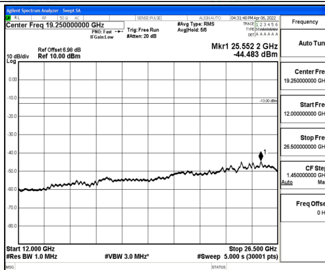
Band12-10MHz-QPSK-23095-1-0-Low-12000-26500--44.48-PASS
