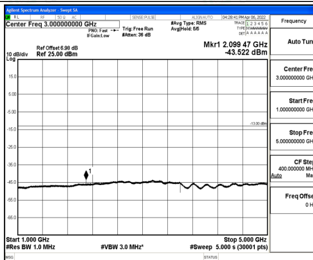
Band12-10MHz-16QAM-23060-1-0-Low-1000-5000--43.52-PASS
