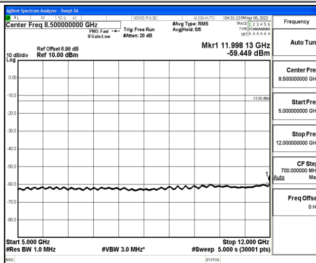
Band12-10MHz-QPSK-23095-1-0-Low-5000-12000--59.45-PASS
