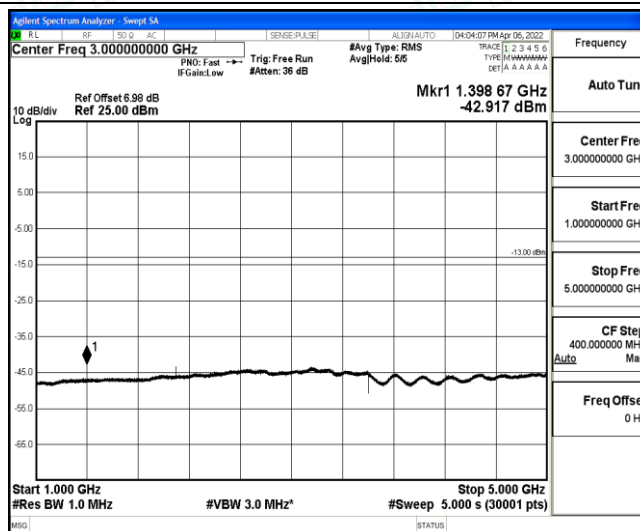
Band12-5MHz-16QAM-23035-1-0-Low-1000-5000--42.92-PASS
