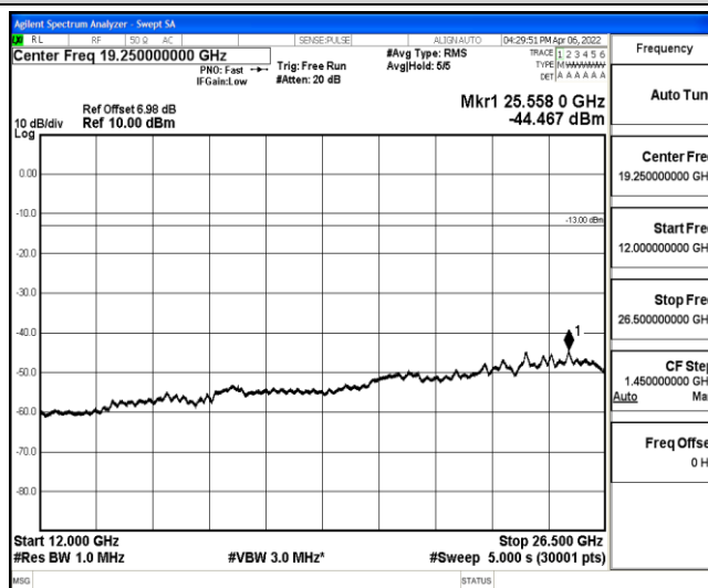
Band12-10MHz-16QAM-23060-1-0-Low-12000-26500--44.47-PASS
