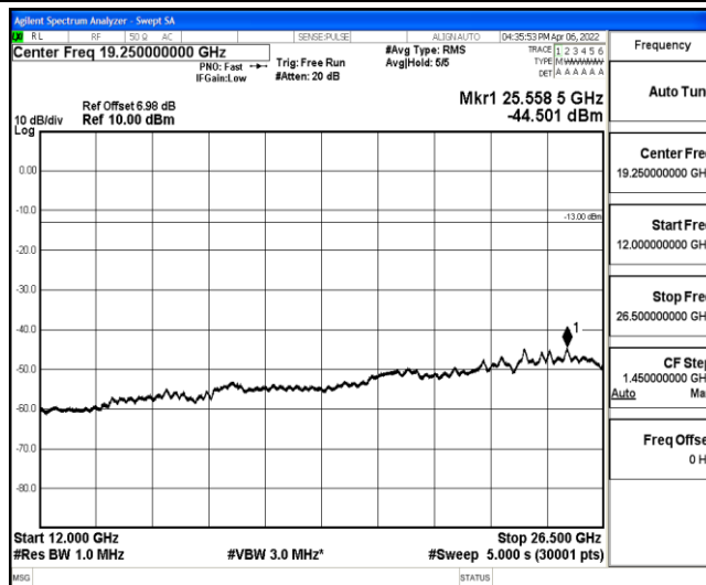
Band12-10MHz-QPSK-23130-1-0-High-12000-26500--44.5-PASS
