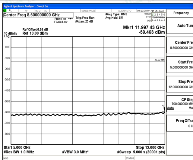
Band12-5MHz-16QAM-23155-1-0-High-5000-12000--59.46-PASS
