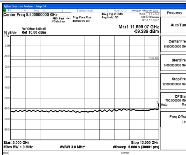
Band12-5MHz-16QAM-23095-1-0-Low-5000-12000--59.29-PASS
