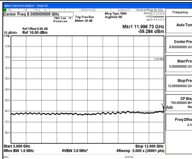
Band12-10MHz-16QAM-23060-1-0-Low-5000-12000--59.28-PASS
