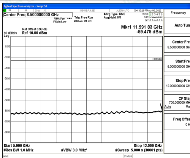
Band12-10MHz-QPSK-23130-1-0-High-5000-12000--59.48-PASS
