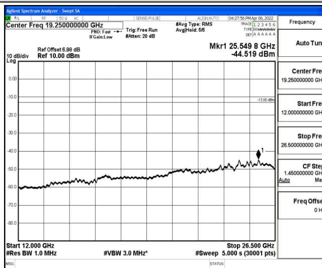
Band12-10MHz-QPSK-23060-1-0-Low-12000-26500--44.52-PASS
