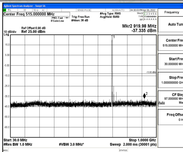
Band12-10MHz-QPSK-23095-1-0-Low-30-1000--37.34-PASS
