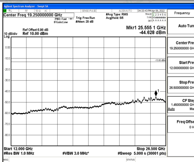
Band12-10MHz-16QAM-23095-1-0-Low-12000-26500--44.63-PASS
