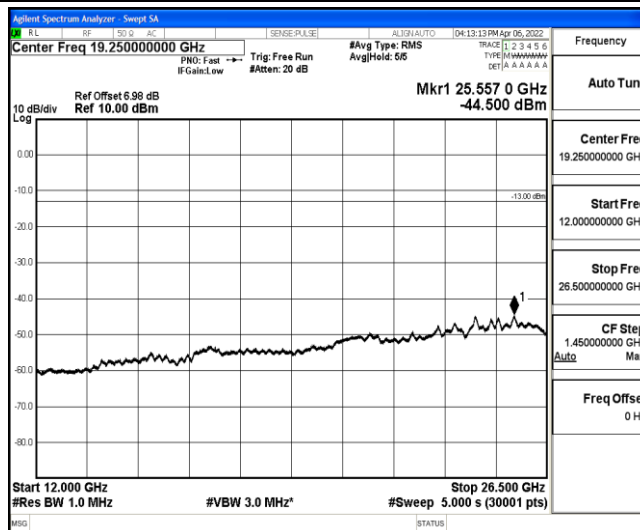
Band12-5MHz-16QAM-23155-1-0-High-12000-26500--44.5-PASS
