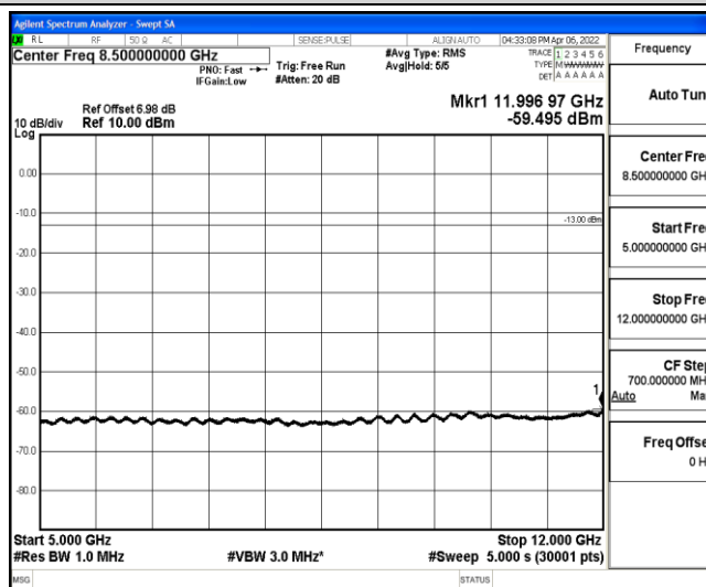
Band12-10MHz-16QAM-23095-1-0-Low-5000-12000--59.5-PASS
