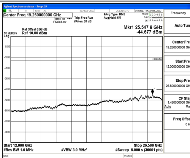
Band12-5MHz-16QAM-23035-1-0-Low-12000-26500--44.68-PASS
