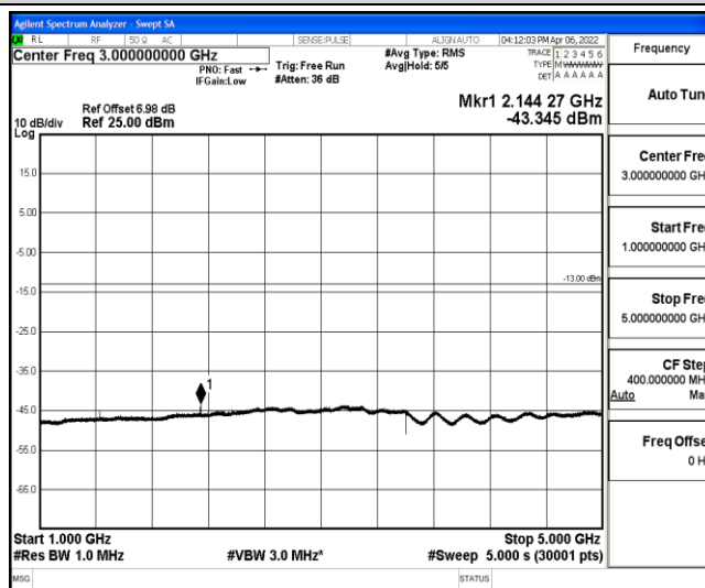
Band12-5MHz-16QAM-23155-1-0-High-1000-5000--43.35-PASS
