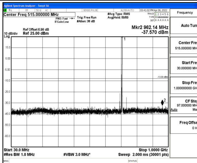
Band12-3MHz-QPSK-23165-1-0-High-30-1000--37.57-PASS
