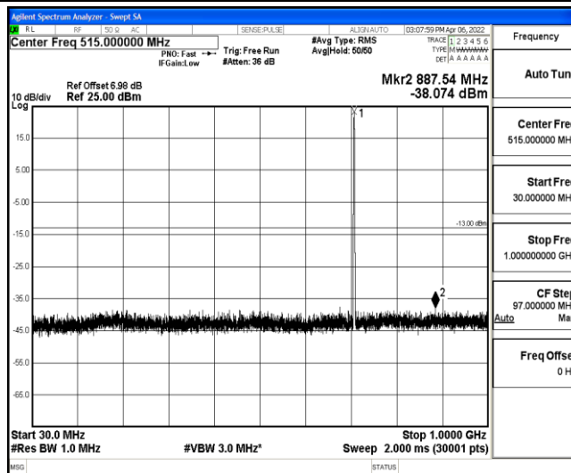
Band12-1.4MHz-QPSK-23173-1-0-High-30-1000--38.07-PASS
