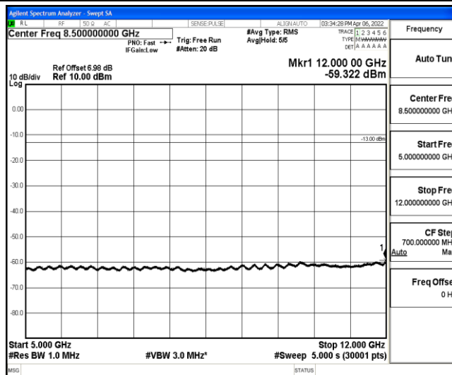
Band12-3MHz-QPSK-23025-1-0-Low-5000-12000--59.32-PASS
