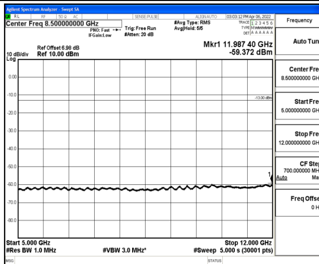
Band12-1.4MHz-16QAM-23017-1-0-Low-5000-12000--59.37-PASS
