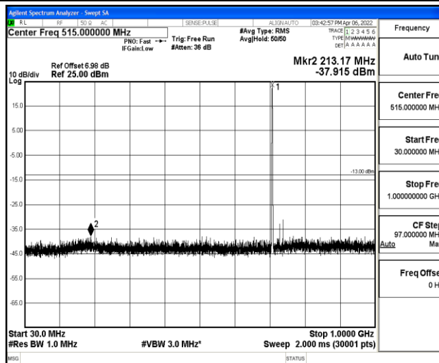
Band12-3MHz-16QAM-23165-1-0-High-30-1000--37.92-PASS
