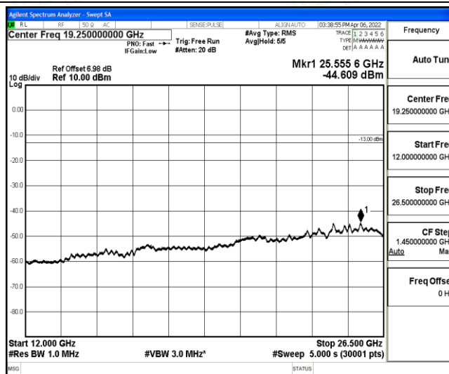
Band12-3MHz-QPSK-23095-1-0-Low-12000-26500--44.61-PASS
