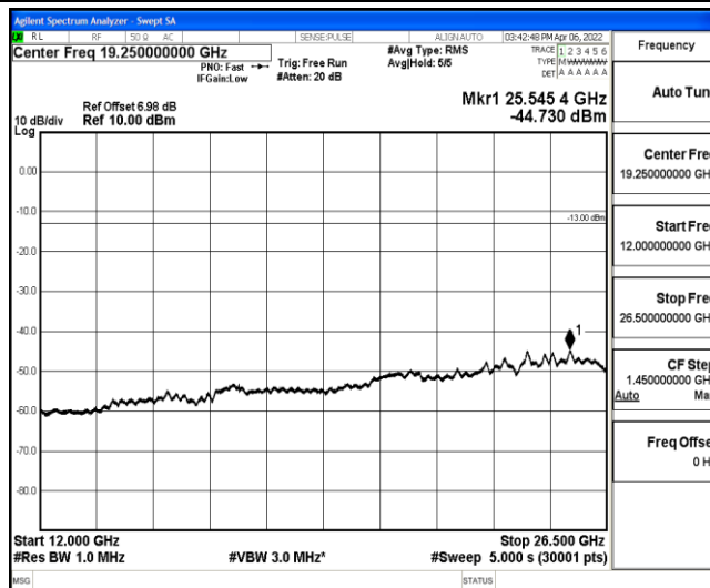
Band12-3MHz-QPSK-23165-1-0-High-12000-26500--44.73-PASS
