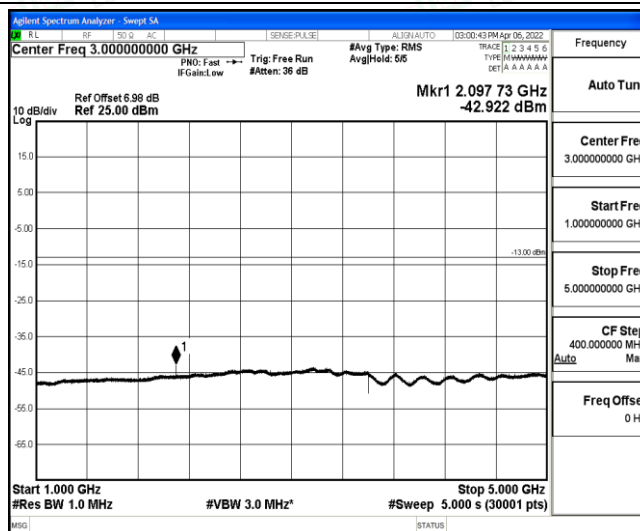
Band12-1.4MHz-QPSK-23017-1-0-Low-1000-5000--42.92-PASS
