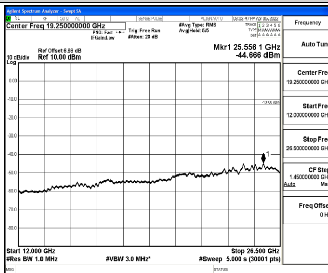
Band12-1.4MHz-16QAM-23017-1-0-Low-12000-26500--44.67-PASS
