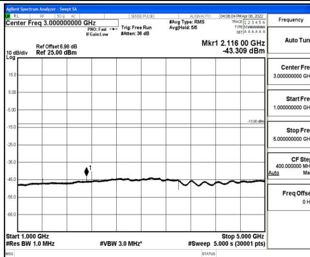
Band12-5MHz-QPSK-23095-1-0-Low-1000-5000--43.31-PASS
