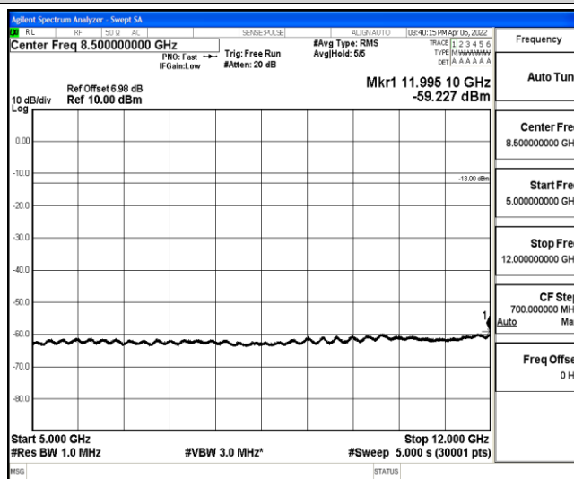
Band12-3MHz-16QAM-23095-1-0-Low-5000-12000--59.23-PASS
