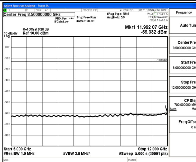
Band12-1.4MHz-QPSK-23017-1-0-Low-5000-12000--59.33-PASS
