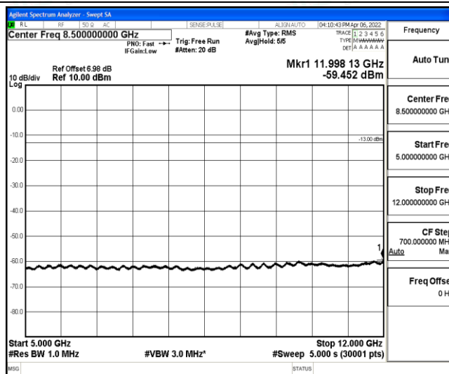
Band12-5MHz-QPSK-23155-1-0-High-5000-12000--59.45-PASS
