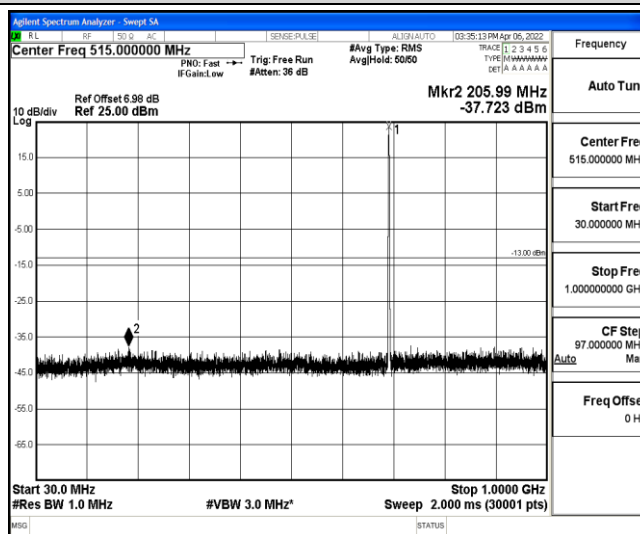
Band12-3MHz-16QAM-23025-1-0-Low-30-1000--37.72-PASS
