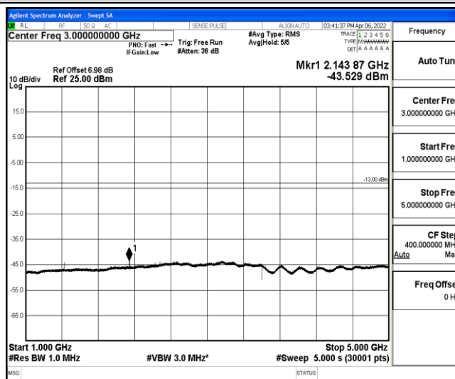
Band12-3MHz-QPSK-23165-1-0-High-1000-5000--43.53-PASS
