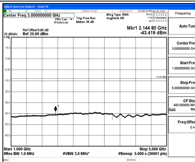
Band12-1.4MHz-QPSK-23173-1-0-High-1000-5000--43.42-PASS
