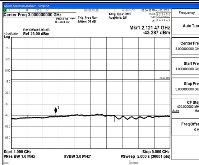
Band12-1.4MHz-16QAM-23095-1-0-Low-1000-5000--43.29-PASS
