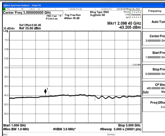
Band12-3MHz-16QAM-23025-1-0-Low-1000-5000--43.21-PASS
