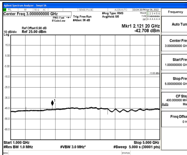
Band12-1.4MHz-QPSK-23095-1-0-Low-1000-5000--42.71-PASS
