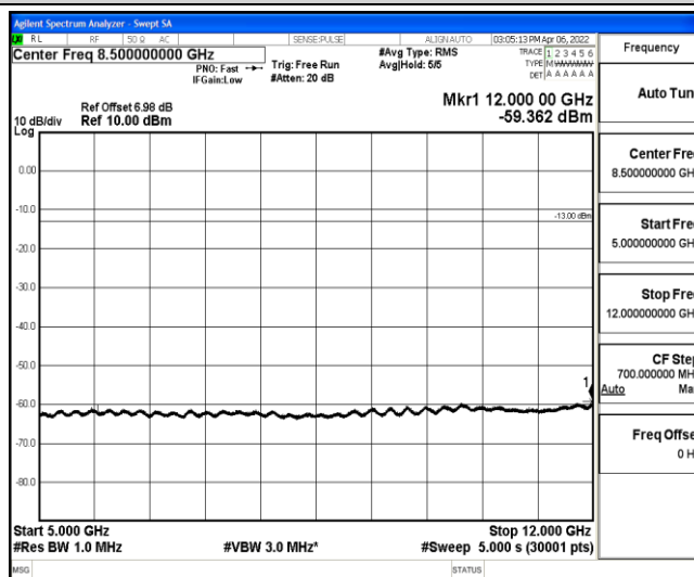
Band12-1.4MHz-QPSK-23095-1-0-Low-5000-12000--59.36-PASS
