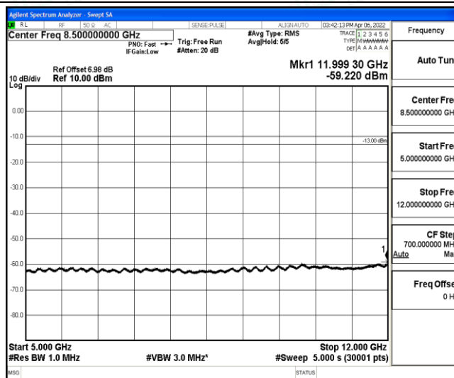
Band12-3MHz-QPSK-23165-1-0-High-5000-12000--59.22-PASS
