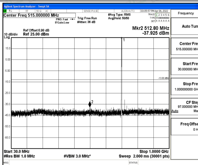
Band12-1.4MHz-16QAM-23095-1-0-Low-30-1000--37.93-PASS
