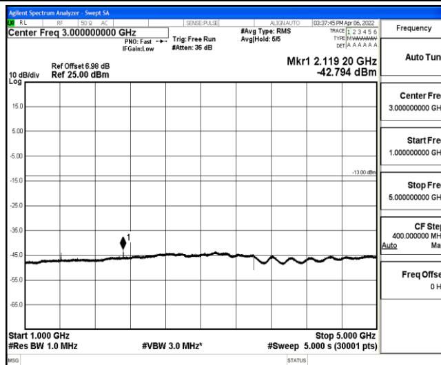
Band12-3MHz-QPSK-23095-1-0-Low-1000-5000--42.79-PASS
