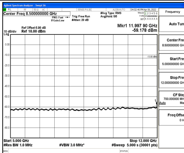
Band12-5MHz-QPSK-23035-1-0-Low-5000-12000--59.18-PASS
