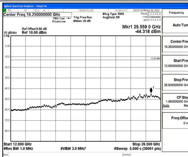
Band12-1.4MHz-16QAM-23095-1-0-Low-12000-26500--44.32-PASS
