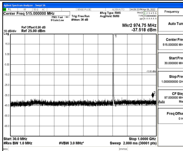
Band12-5MHz-QPSK-23155-1-0-High-30-1000--37.52-PASS
