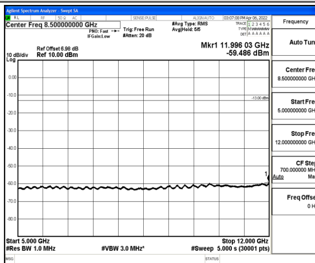
Band12-1.4MHz-16QAM-23095-1-0-Low-5000-12000--59.49-PASS
