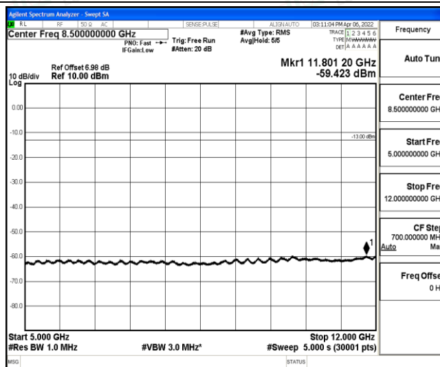
Band12-1.4MHz-16QAM-23173-1-0-High-5000-12000--59.42-PASS
