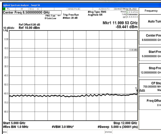
Band12-3MHz-16QAM-23165-1-0-High-5000-12000--59.44-PASS
