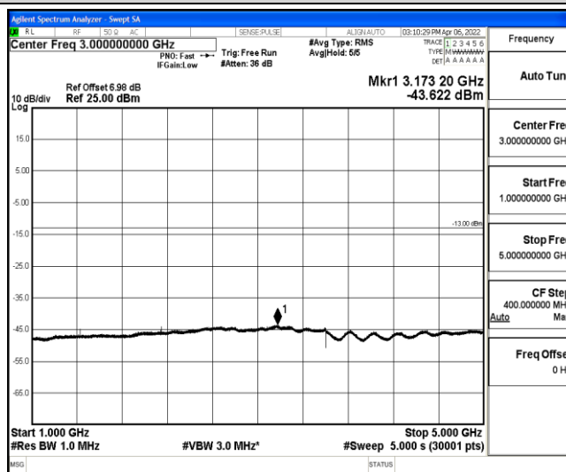
Band12-1.4MHz-16QAM-23173-1-0-High-1000-5000--43.62-PASS
