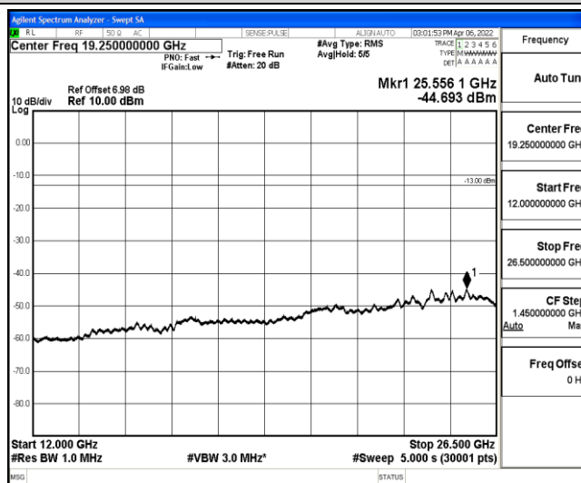
Band12-1.4MHz-QPSK-23017-1-0-Low-12000-26500--44.69-PASS
