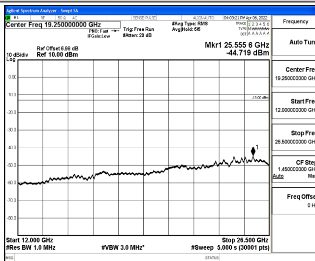
Band12-5MHz-QPSK-23035-1-0-Low-12000-26500--44.72-PASS
