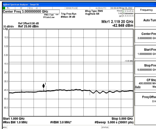
Band12-3MHz-16QAM-23095-1-0-Low-1000-5000--42.85-PASS
