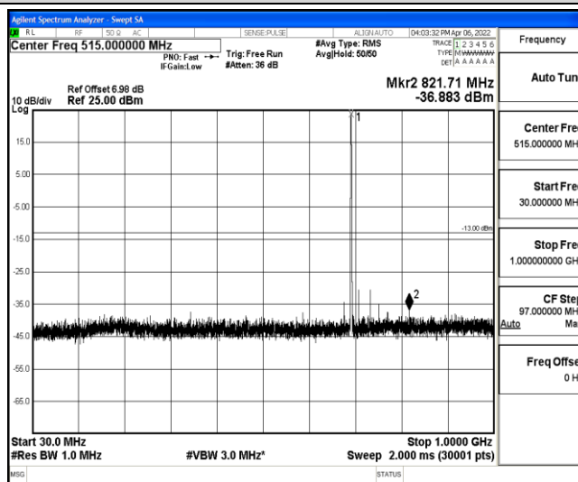
Band12-5MHz-16QAM-23035-1-0-Low-30-1000--36.88-PASS
