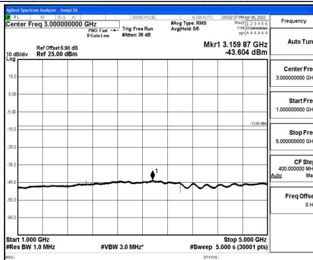
Band12-1.4MHz-16QAM-23017-1-0-Low-1000-5000--43.6-PASS
