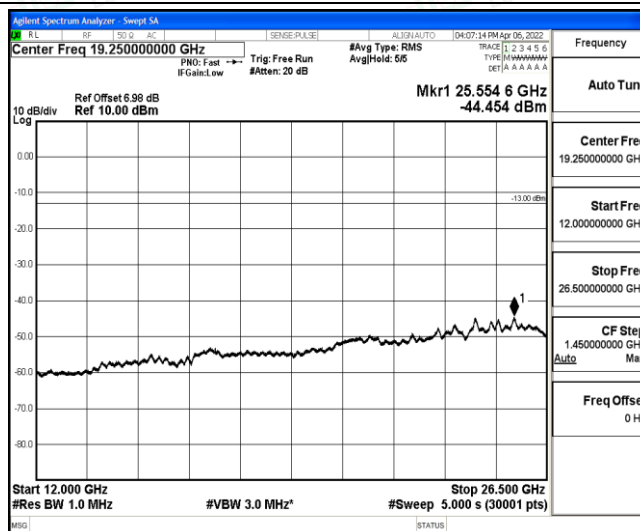
Band12-5MHz-QPSK-23095-1-0-Low-12000-26500--44.45-PASS
