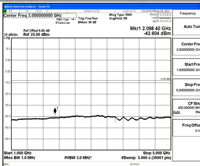
Band12-3MHz-QPSK-23025-1-0-Low-1000-5000--42.6-PASS
