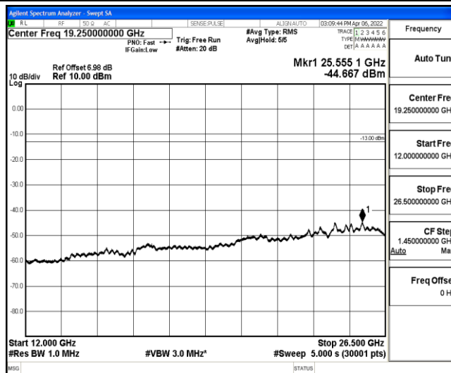
Band12-1.4MHz-QPSK-23173-1-0-High-12000-26500--44.67-PASS
