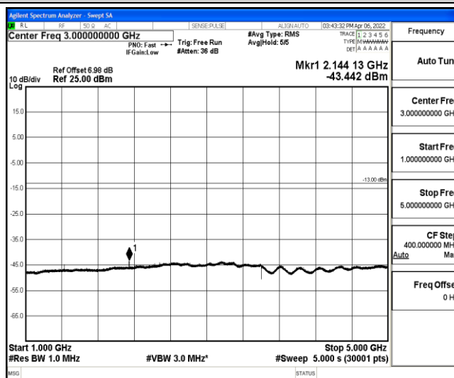
Band12-3MHz-16QAM-23165-1-0-High-1000-5000--43.44-PASS
