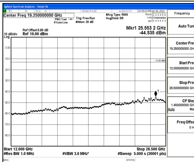
Band12-3MHz-QPSK-23025-1-0-Low-12000-26500--44.54-PASS
