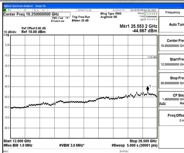
Band12-3MHz-16QAM-23095-1-0-Low-12000-26500--44.67-PASS
