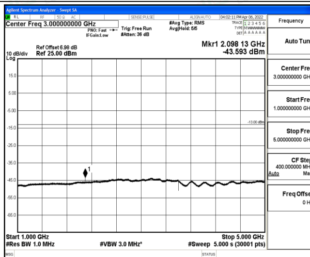
Band12-5MHz-QPSK-23035-1-0-Low-1000-5000--43.59-PASS
