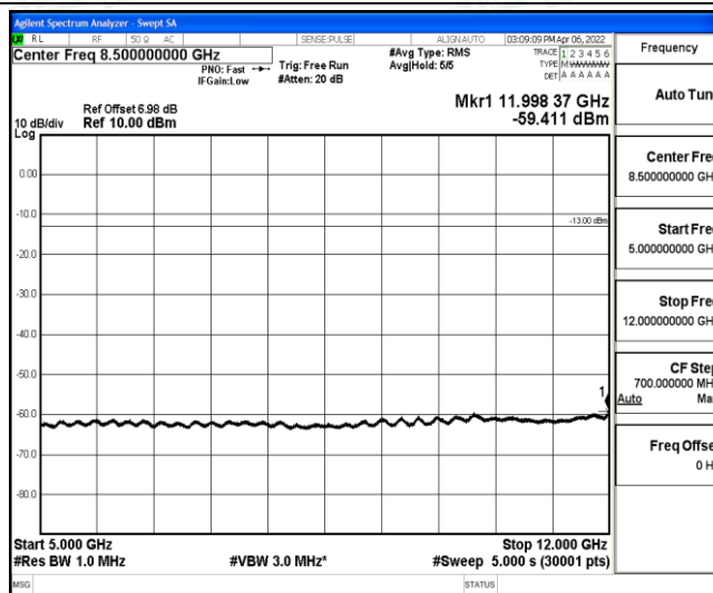
Band12-1.4MHz-QPSK-23173-1-0-High-5000-12000--59.41-PASS
