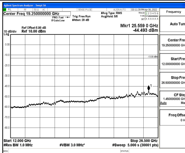
Band12-1.4MHz-16QAM-23173-1-0-High-12000-26500--44.49-PASS
