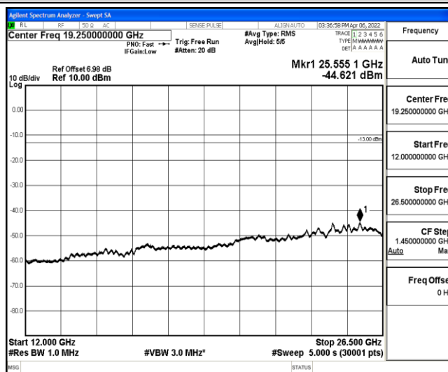
Band12-3MHz-16QAM-23025-1-0-Low-12000-26500--44.62-PASS
