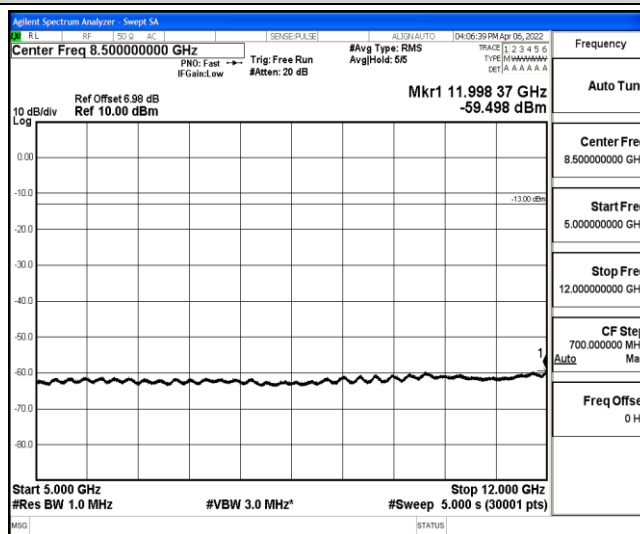
Band12-5MHz-QPSK-23095-1-0-Low-5000-12000--59.5-PASS
