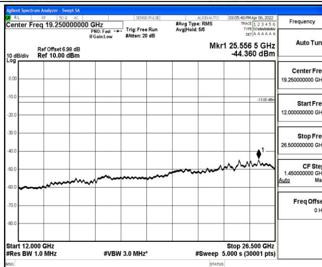
Band12-1.4MHz-QPSK-23095-1-0-Low-12000-26500--44.36-PASS
