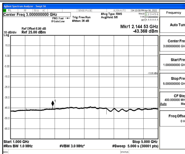
Band12-5MHz-QPSK-23155-1-0-High-1000-5000--43.37-PASS
