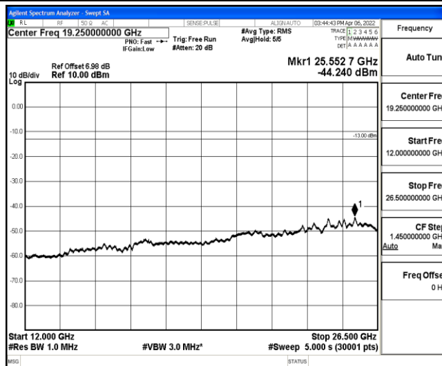
Band12-3MHz-16QAM-23165-1-0-High-12000-26500--44.24-PASS
