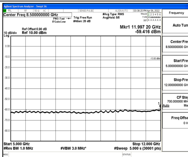
Band12-3MHz-QPSK-23095-1-0-Low-5000-12000--59.42-PASS
