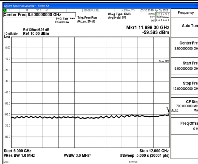
Band12-3MHz-16QAM-23025-1-0-Low-5000-12000--59.39-PASS
