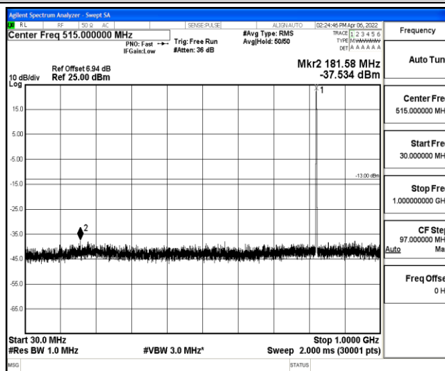
Band5-10MHz-16QAM-20450-1-0-Low-30-1000--37.53-PASS
