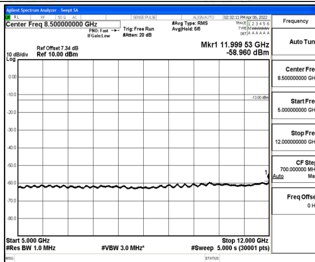
Band5-10MHz-QPSK-20600-1-0-High-5000-12000--58.96-PASS
