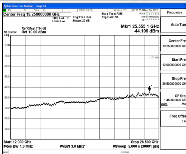
Band5-10MHz-16QAM-20525-1-0-Low-12000-26500--44.2-PASS
