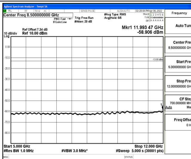
Band5-10MHz-QPSK-20525-1-0-Low-5000-12000--58.91-PASS
