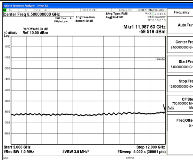
Band5-5MHz-16QAM-20425-1-0-Low-5000-12000--59.52-PASS
