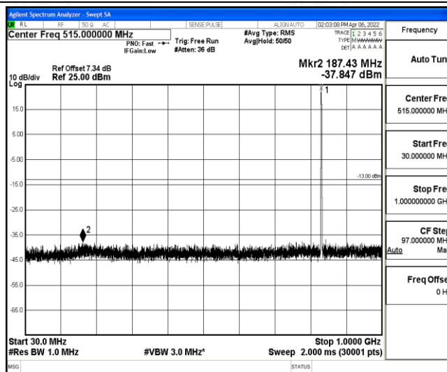
Band5-5MHz-16QAM-20525-1-0-Low-30-1000--37.85-PASS
