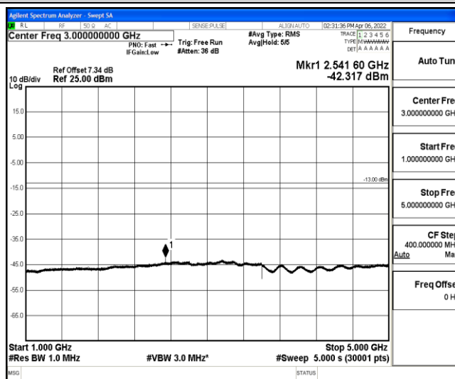
Band5-10MHz-QPSK-20600-1-0-High-1000-5000--42.32-PASS
