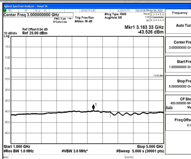
Band5-10MHz-QPSK-20450-1-0-Low-1000-5000--43.53-PASS
