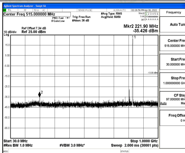
Band5-10MHz-QPSK-20525-1-0-Low-30-1000--35.43-PASS
