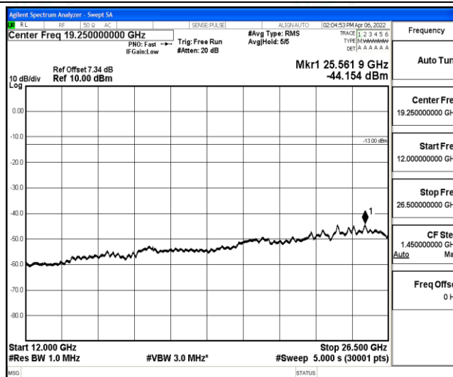
Band5-5MHz-16QAM-20525-1-0-Low-12000-26500--44.15-PASS
