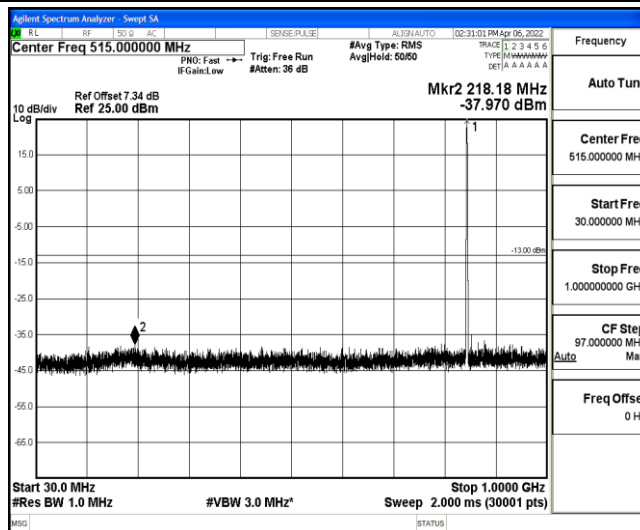
Band5-10MHz-QPSK-20600-1-0-High-30-1000--37.97-PASS
