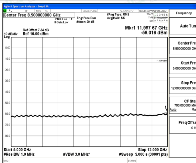
Band5-5MHz-16QAM-20625-1-0-High-5000-12000--59.02-PASS
