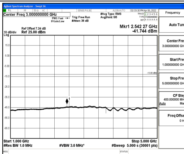
Band5-10MHz-16QAM-20600-1-0-High-1000-5000--41.74-PASS
