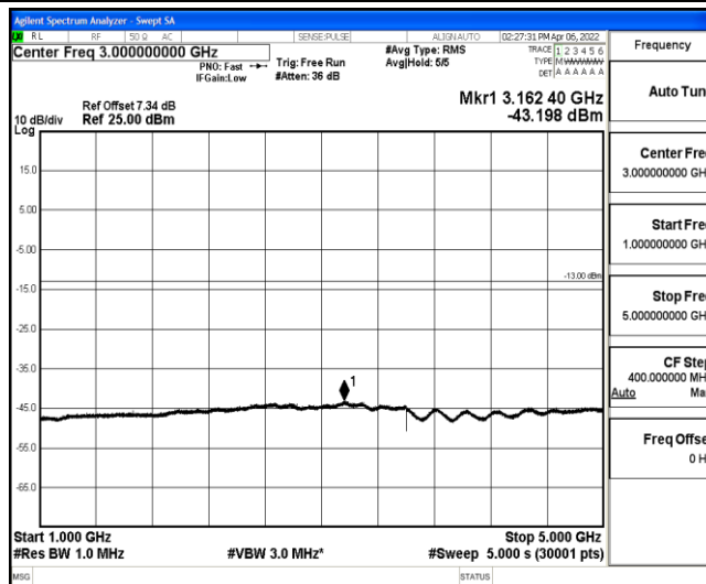
Band5-10MHz-QPSK-20525-1-0-Low-1000-5000--43.2-PASS
