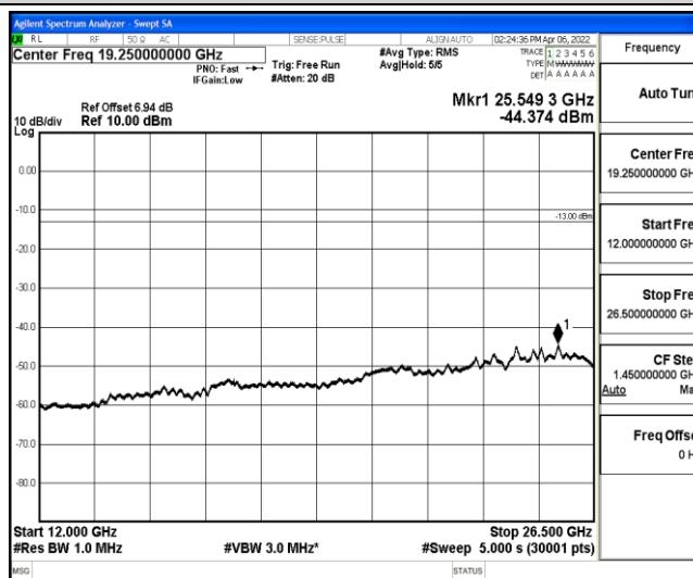
Band5-10MHz-QPSK-20450-1-0-Low-12000-26500--44.37-PASS
