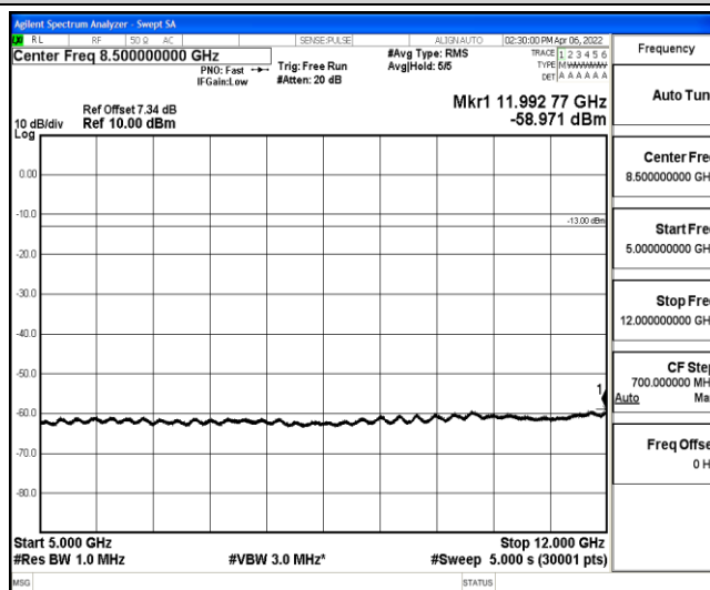
Band5-10MHz-16QAM-20525-1-0-Low-5000-12000--58.97-PASS
