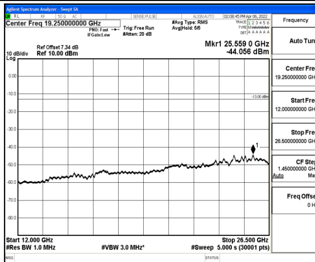
Band5-5MHz-16QAM-20625-1-0-High-12000-26500--44.06-PASS
