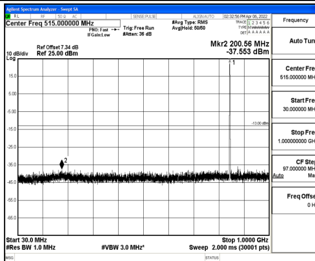
Band5-10MHz-16QAM-20600-1-0-High-30-1000--37.55-PASS
