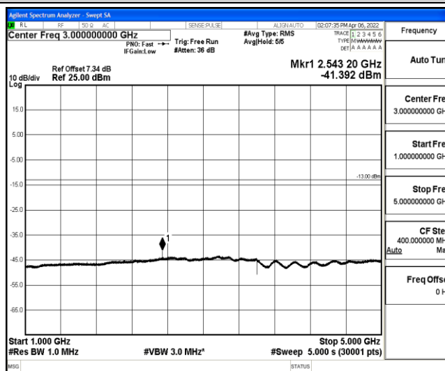
Band5-5MHz-16QAM-20625-1-0-High-1000-5000--41.39-PASS
