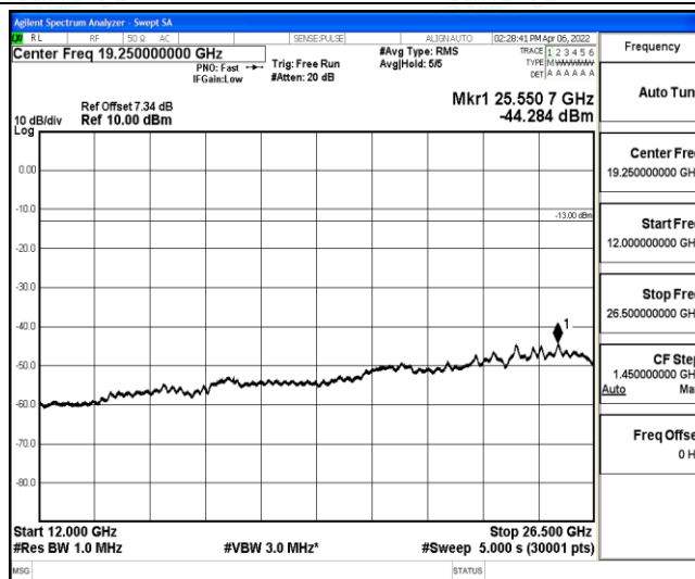
Band5-10MHz-QPSK-20525-1-0-Low-12000-26500--44.28-PASS
