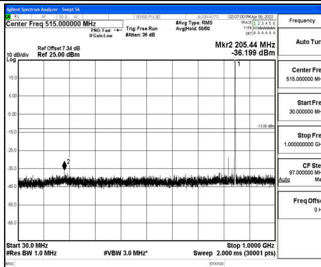
Band5-5MHz-16QAM-20625-1-0-High-30-1000--36.2-PASS
