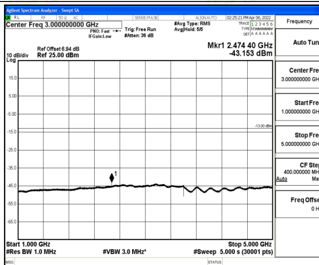
Band5-10MHz-16QAM-20450-1-0-Low-1000-5000--43.15-PASS
