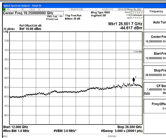
Band5-5MHz-16QAM-20425-1-0-Low-12000-26500--44.62-PASS
