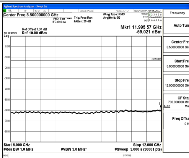
Band5-5MHz-16QAM-20525-1-0-Low-5000-12000--59.02-PASS
