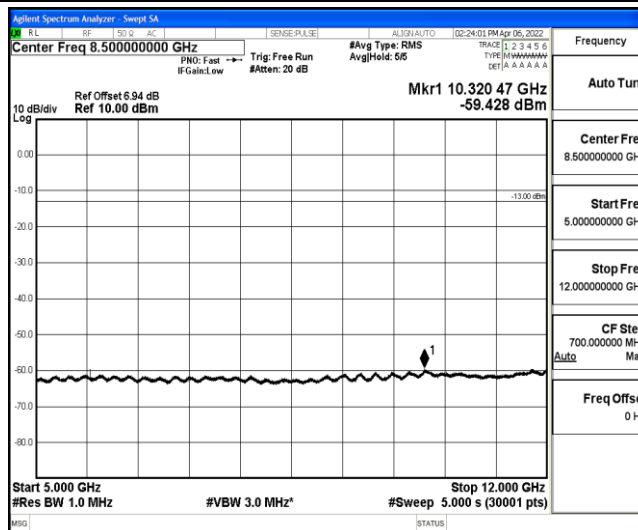
Band5-10MHz-QPSK-20450-1-0-Low-5000-12000--59.43-PASS
