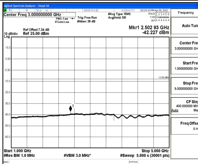
Band5-5MHz-16QAM-20525-1-0-Low-1000-5000--42.23-PASS
