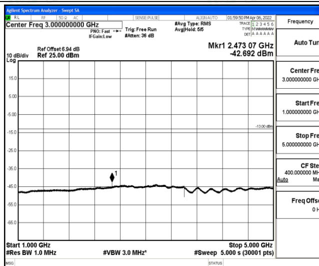
Band5-5MHz-16QAM-20425-1-0-Low-1000-5000--42.69-PASS
