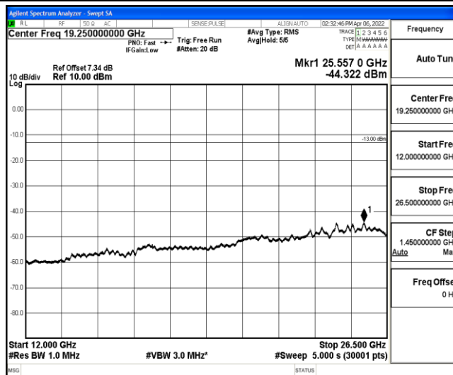
Band5-10MHz-QPSK-20600-1-0-High-12000-26500--44.32-PASS
