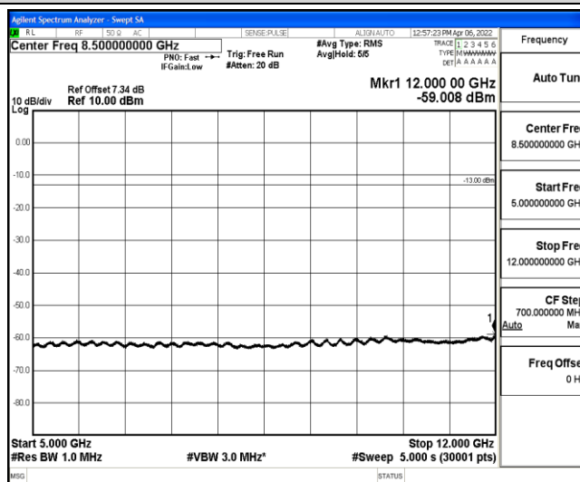
Band5-1.4MHz-QPSK-20525-1-0-Low-5000-12000--59.01-PASS
