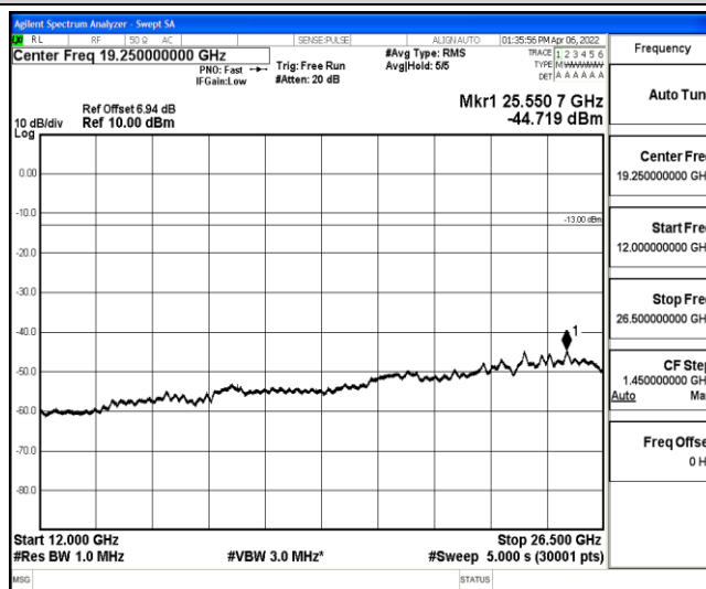
Band5-3MHz-16QAM-20415-1-0-Low-12000-26500--44.72-PASS
