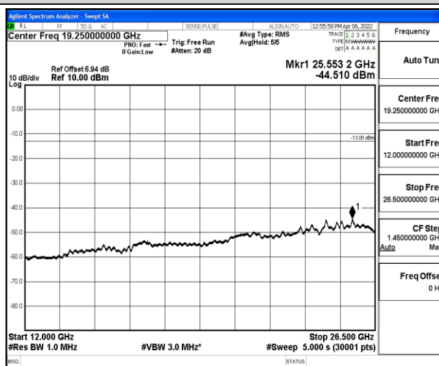
Band5-1.4MHz-16QAM-20407-1-0-Low-12000-26500--44.51-PASS
