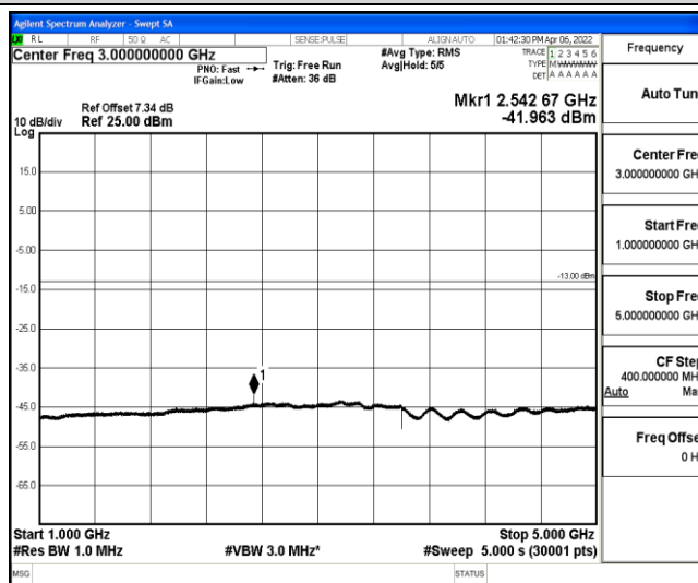
Band5-3MHz-16QAM-20635-1-0-High-1000-5000--41.96-PASS
