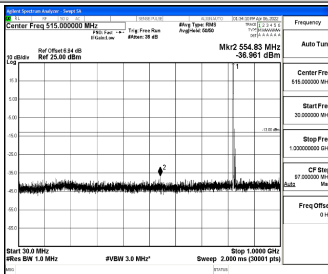
Band5-3MHz-16QAM-20415-1-0-Low-30-1000--36.96-PASS
