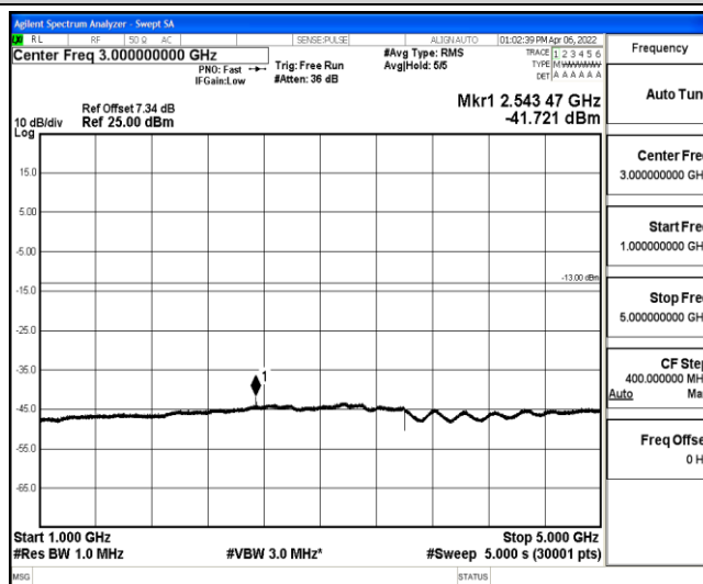
Band5-1.4MHz-16QAM-20643-1-0-High-1000-5000--41.72-PASS
