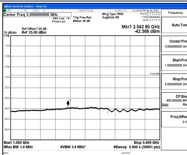
Band5-3MHz-QPSK-20635-1-0-High-1000-5000--42.37-PASS
