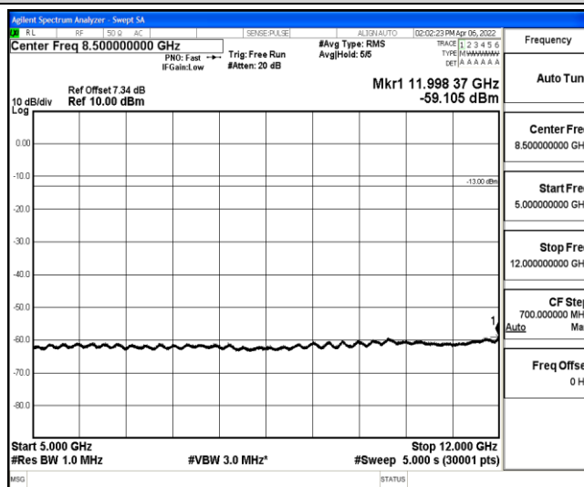
Band5-5MHz-QPSK-20525-1-0-Low-5000-12000--59.11-PASS
