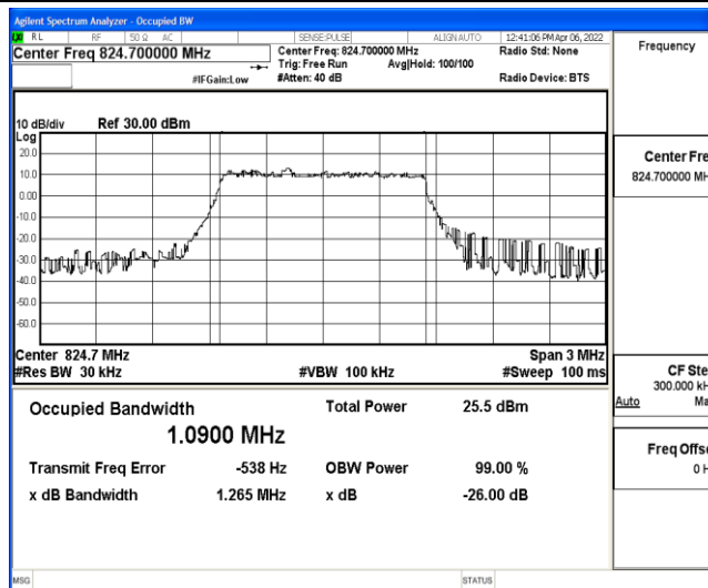
Band5-1.4MHz-16QAM-20407-6-0-Low-1.0900-1.265-PASS
