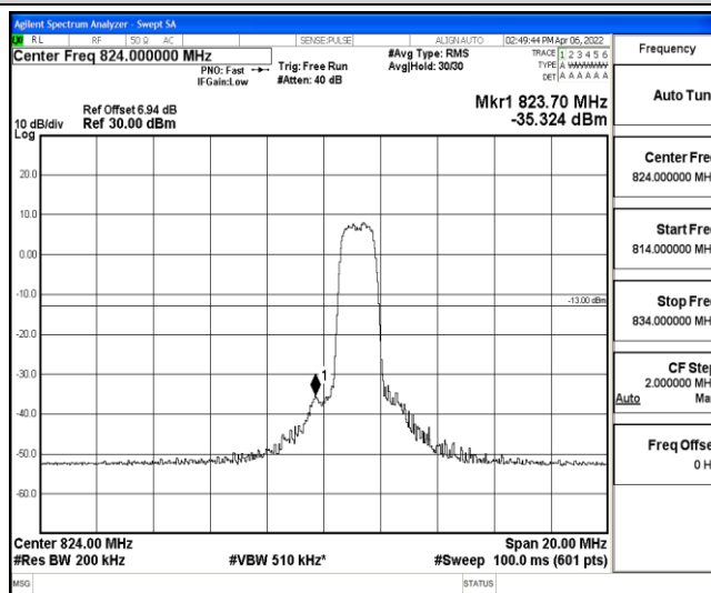
Band5-10MHz-QPSK-20450-6-0-Low--35.32-PASS
