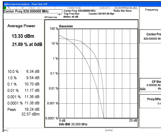
Band5-10MHz-16QAM-20450-6-0-Low-10.70-&lt;=13-PASS
