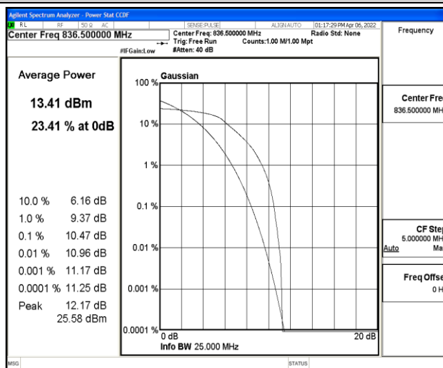
Band5-3MHz-QPSK-20525-6-0-Low-10.47-&lt;=13-PASS
