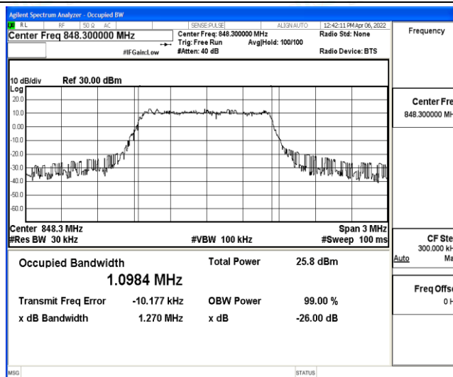
Band5-1.4MHz-QPSK-20643-6-0-High-1.0984-1.270-PASS
