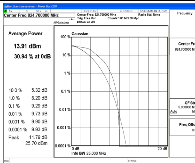
Band5-1.4MHz-QPSK-20407-6-0-Low-9.29-&lt;=13-PASS
