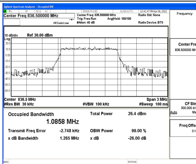
Band5-1.4MHz-16QAM-20525-6-0-Low-1.0858-1.265-PASS
