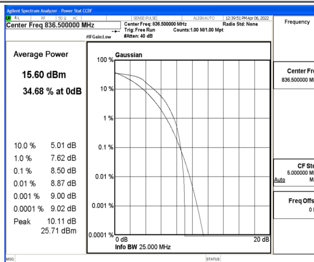
Band5-1.4MHz-QPSK-20525-6-0-Low-8.50-&lt;=13-PASS
