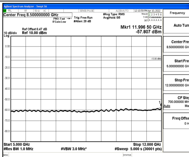
Band4-20MHz-QPSK-20300-1-0-High-5000-12000--57.81-PASS
