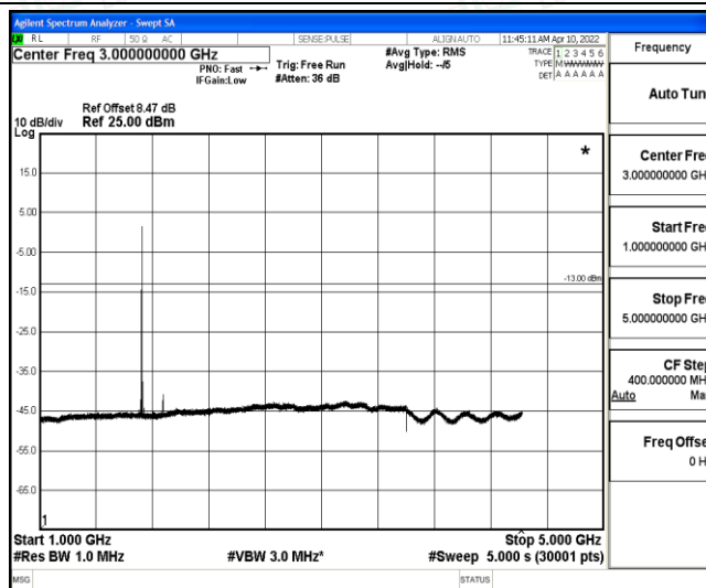
Band4-15MHz-16QAM-20175-1-0-Low-1000-5000--41.27-PASS
