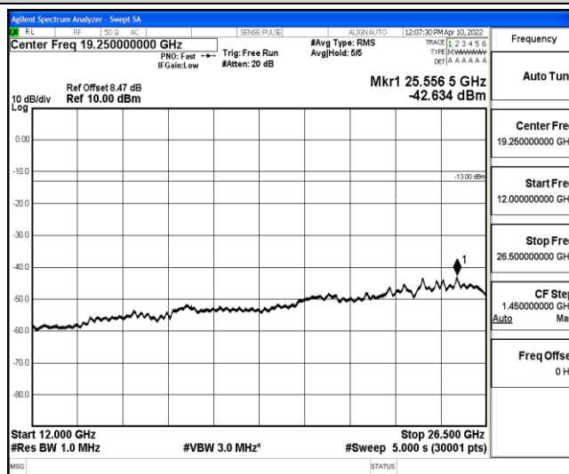
Band4-20MHz-QPSK-20175-1-0-Low-12000-26500--42.63-PASS
