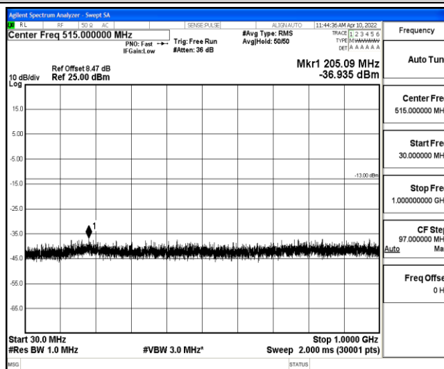
Band4-15MHz-16QAM-20175-1-0-Low-30-1000--36.94-PASS
