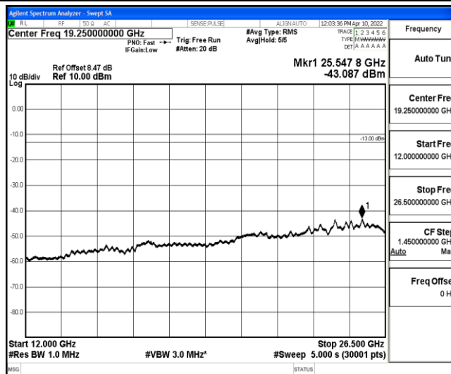
Band4-20MHz-QPSK-20050-1-0-Low-12000-26500--43.09-PASS
