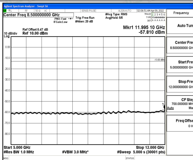
Band4-15MHz-16QAM-20025-1-0-Low-5000-12000--57.81-PASS
