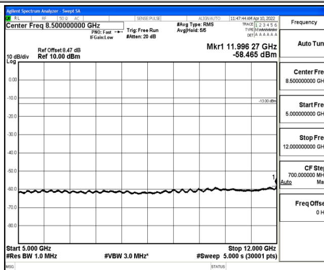
Band4-15MHz-QPSK-20325-1-0-High-5000-12000--58.47-PASS
