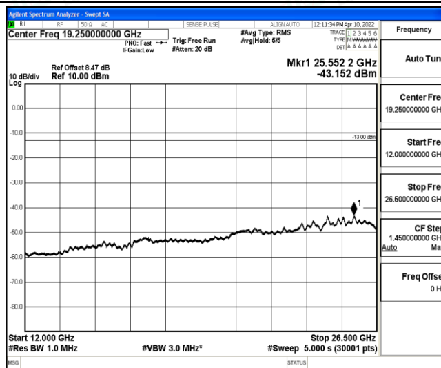
Band4-20MHz-QPSK-20300-1-0-High-12000-26500--43.15-PASS
