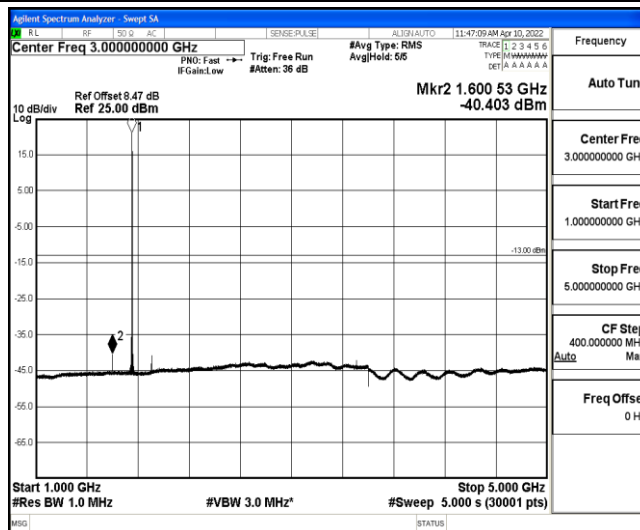
Band4-15MHz-QPSK-20325-1-0-High-1000-5000--40.4-PASS
