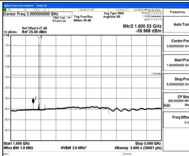
Band4-15MHz-16QAM-20325-1-0-High-1000-5000--39.97-PASS
