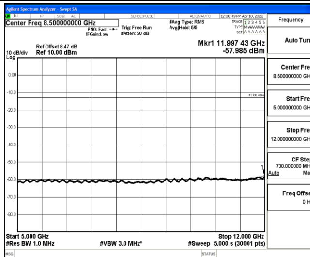
Band4-20MHz-16QAM-20175-1-0-Low-5000-12000--57.99-PASS
