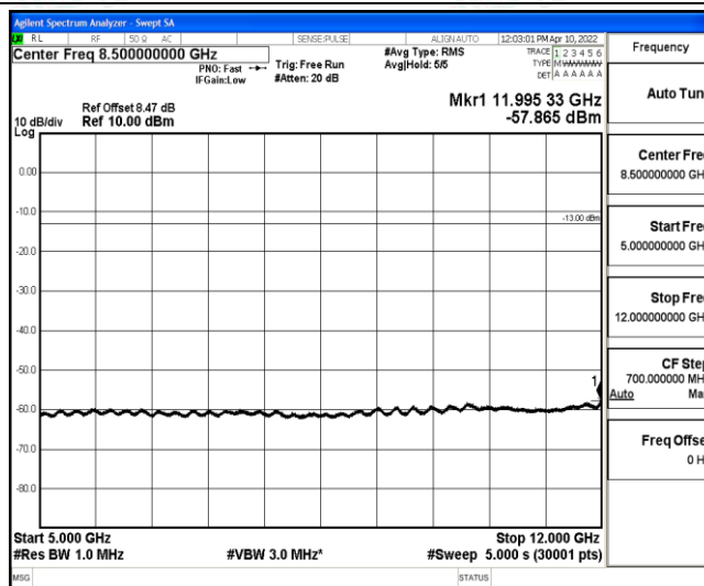
Band4-20MHz-QPSK-20050-1-0-Low-5000-12000--57.87-PASS
