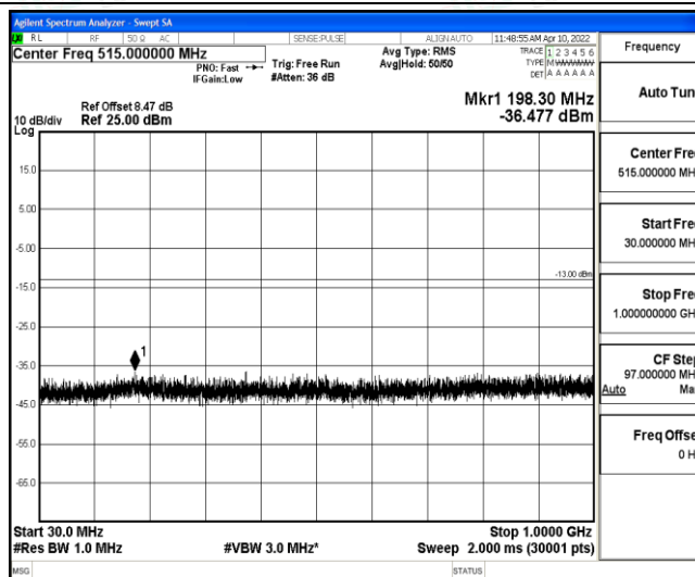
Band4-15MHz-16QAM-20325-1-0-High-30-1000--36.48-PASS
