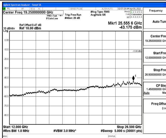
Band4-15MHz-16QAM-20025-1-0-Low-12000-26500--43.18-PASS
