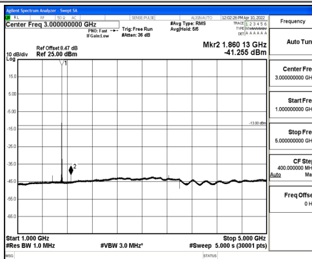
Band4-20MHz-QPSK-20050-1-0-Low-1000-5000--41.26-PASS
