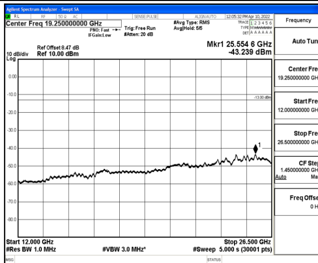
Band4-20MHz-16QAM-20050-1-0-Low-12000-26500--43.24-PASS
