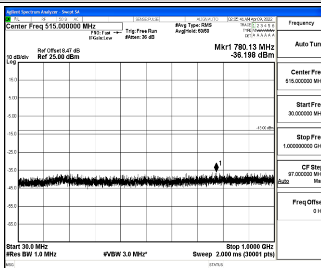
Band4-15MHz-16QAM-20025-1-0-Low-30-1000--36.2-PASS
