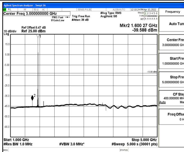
Band4-20MHz-QPSK-20300-1-0-High-1000-5000--39.59-PASS
