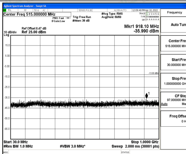
Band4-20MHz-QPSK-20300-1-0-High-30-1000--35.99-PASS
