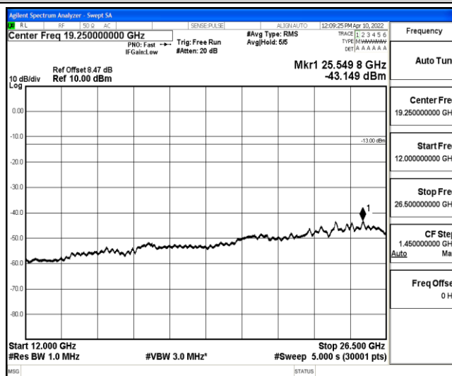
Band4-20MHz-16QAM-20175-1-0-Low-12000-26500--43.15-PASS
