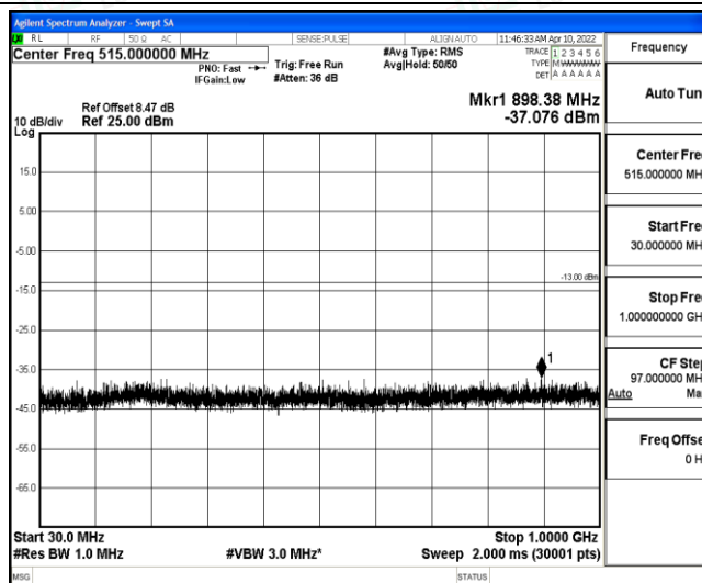
Band4-15MHz-QPSK-20325-1-0-High-30-1000--37.08-PASS
