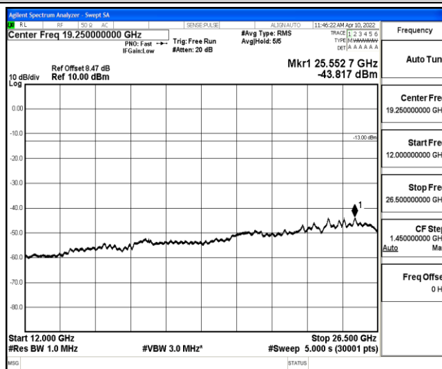
Band4-15MHz-16QAM-20175-1-0-Low-12000-26500--43.82-PASS
