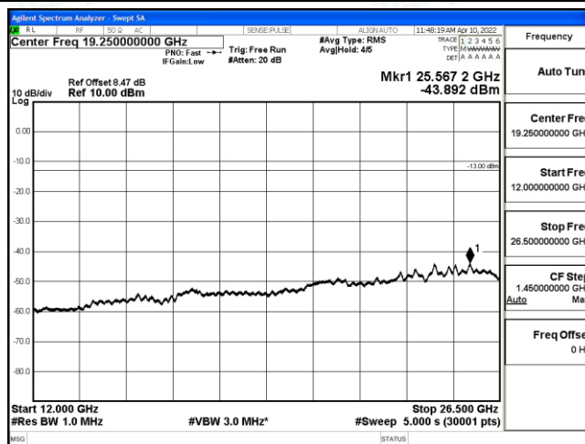
Band4-15MHz-QPSK-20325-1-0-High-12000-26500--43.89-PASS
