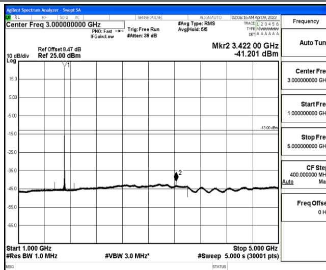
Band4-15MHz-16QAM-20025-1-0-Low-1000-5000--41.2-PASS
