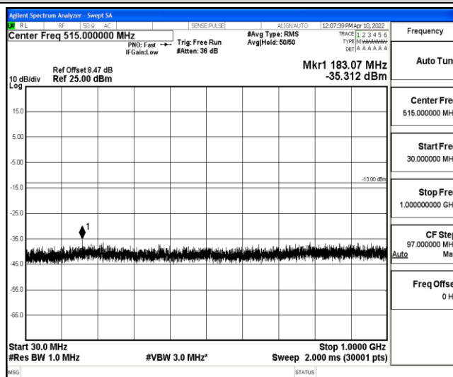
Band4-20MHz-16QAM-20175-1-0-Low-30-1000--35.31-PASS
