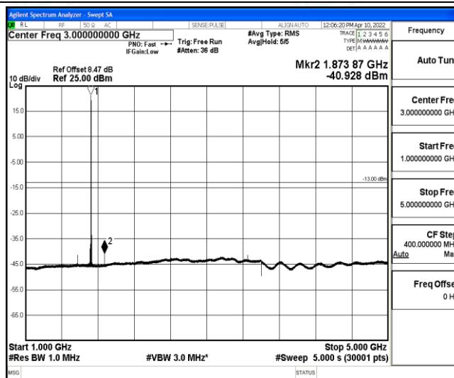
Band4-20MHz-QPSK-20175-1-0-Low-1000-5000--40.93-PASS
