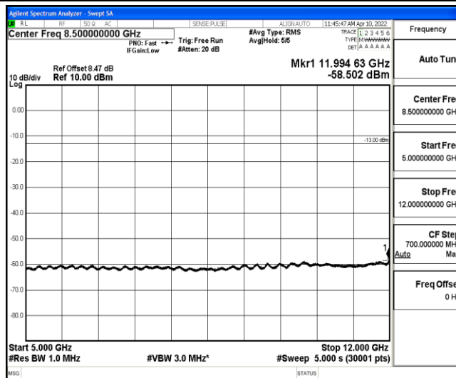
Band4-15MHz-16QAM-20175-1-0-Low-5000-12000--58.5-PASS
