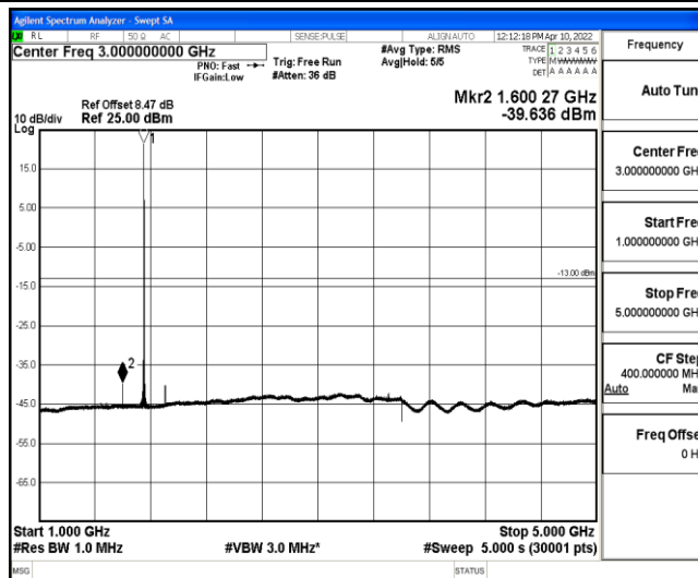
Band4-20MHz-16QAM-20300-1-0-High-1000-5000--39.64-PASS
