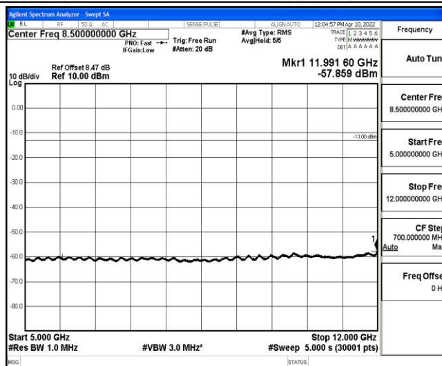
Band4-20MHz-16QAM-20050-1-0-Low-5000-12000--57.86-PASS
