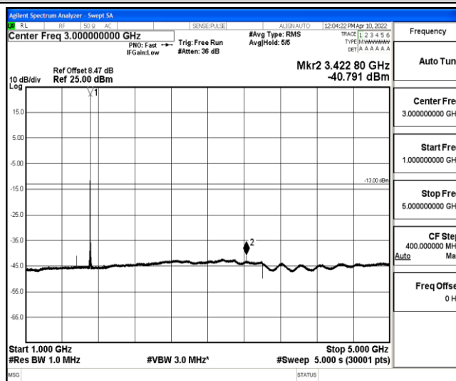
Band4-20MHz-16QAM-20050-1-0-Low-1000-5000--40.79-PASS
