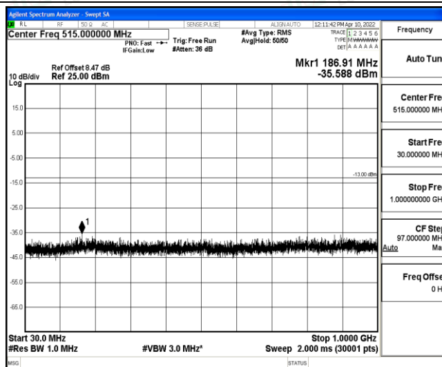
Band4-20MHz-16QAM-20300-1-0-High-30-1000--35.59-PASS
