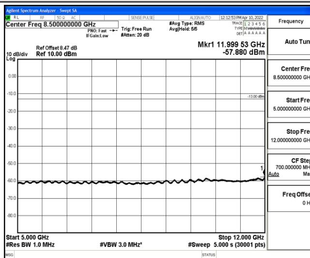
Band4-20MHz-16QAM-20300-1-0-High-5000-12000--57.88-PASS
