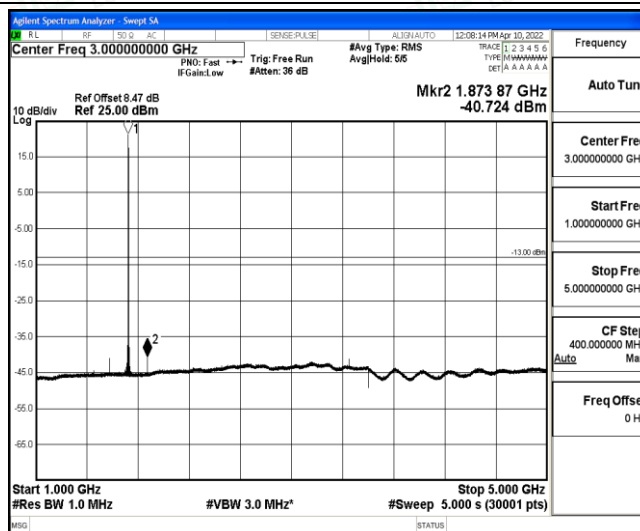
Band4-20MHz-16QAM-20175-1-0-Low-1000-5000--40.72-PASS
