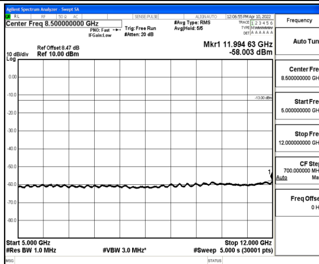
Band4-20MHz-QPSK-20175-1-0-Low-5000-12000--58-PASS
