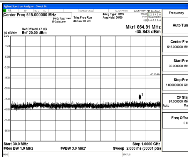
Band4-20MHz-QPSK-20175-1-0-Low-30-1000--35.84-PASS
