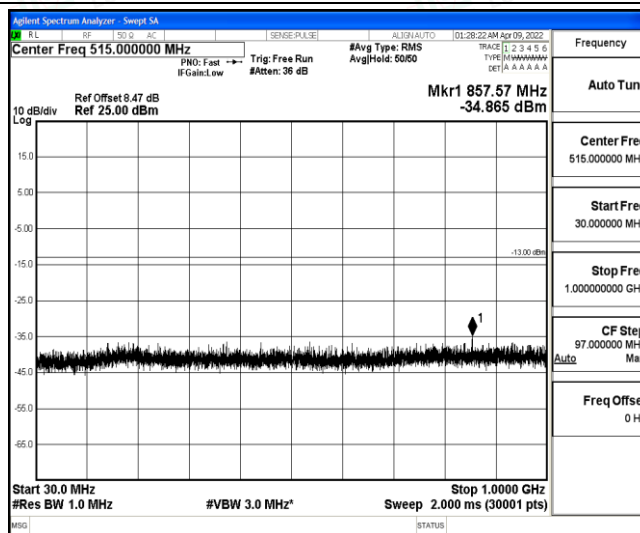
Band4-5MHz-QPSK-20375-1-0-High-30-1000--34.87-PASS
