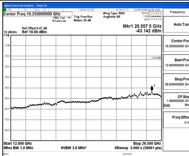
Band4-3MHz-QPSK-19965-1-0-Low-12000-26500--43.14-PASS
