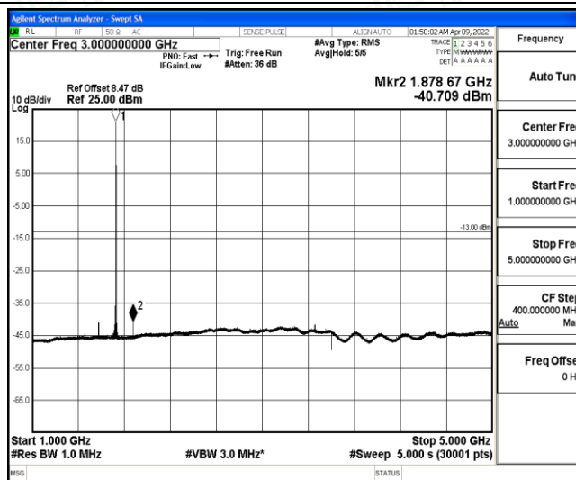
Band4-10MHz-16QAM-20175-1-0-Low-1000-5000--40.71-PASS
