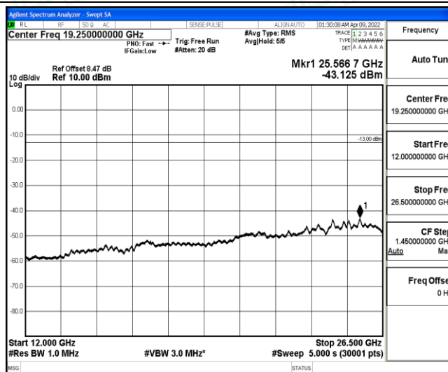
Band4-5MHz-QPSK-20375-1-0-High-12000-26500--43.13-PASS
