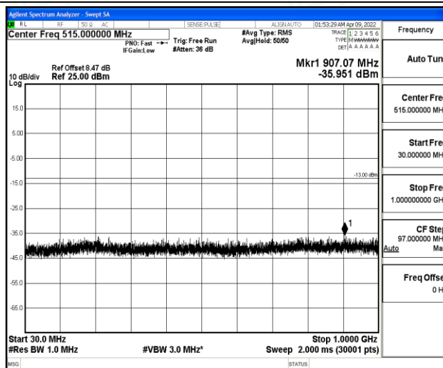
Band4-10MHz-16QAM-20350-1-0-High-30-1000--35.95-PASS
