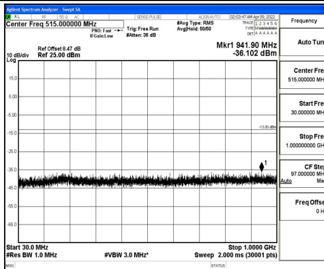
Band4-15MHz-QPSK-20025-1-0-Low-30-1000--36.1-PASS
