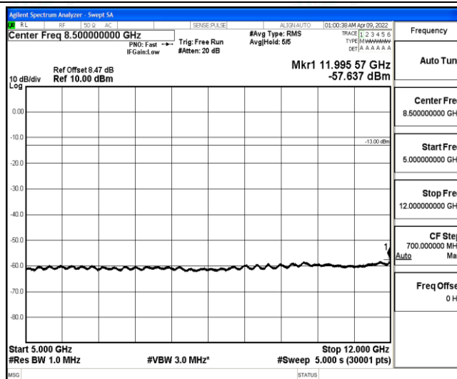
Band4-3MHz-16QAM-19965-1-0-Low-5000-12000--57.64-PASS
