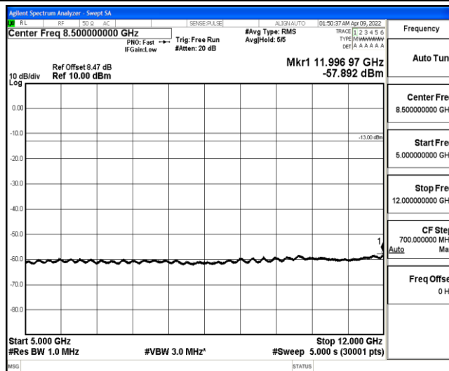
Band4-10MHz-16QAM-20175-1-0-Low-5000-12000--57.89-PASS
