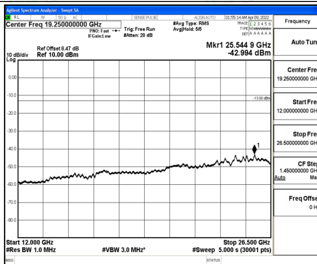
Band4-10MHz-16QAM-20350-1-0-High-12000-26500--42.99-PASS
