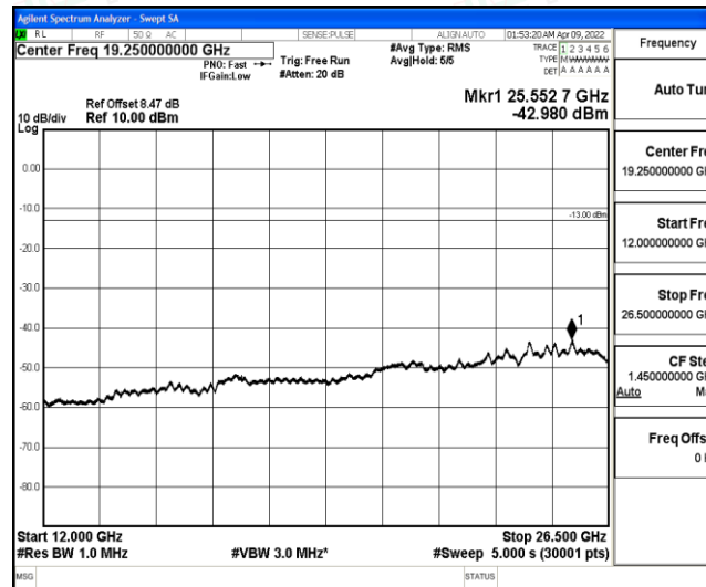
Band4-10MHz-QPSK-20350-1-0-High-12000-26500--42.98-PASS
