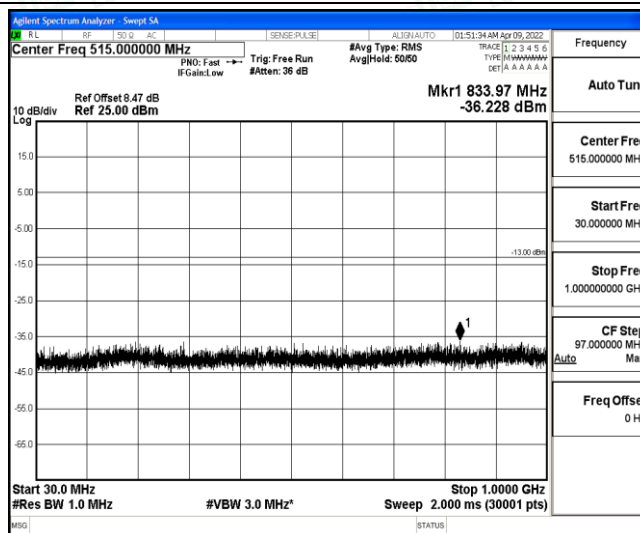
Band4-10MHz-QPSK-20350-1-0-High-30-1000--36.23-PASS
