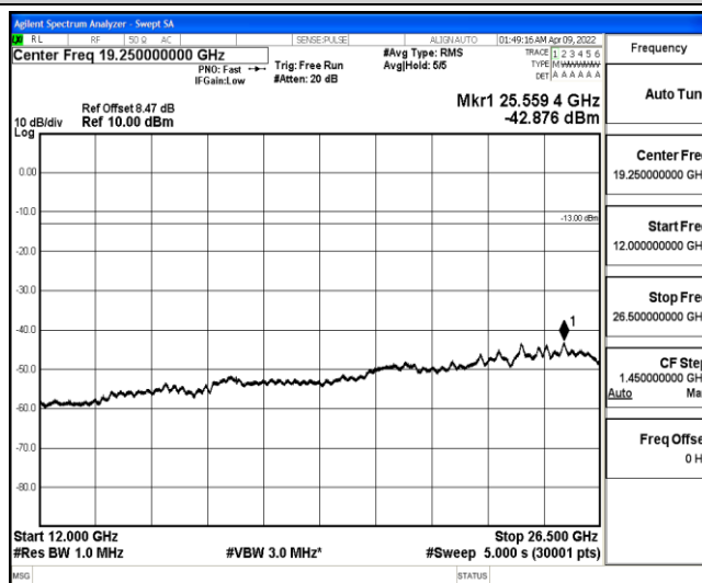
Band4-10MHz-QPSK-20175-1-0-Low-12000-26500--42.88-PASS
