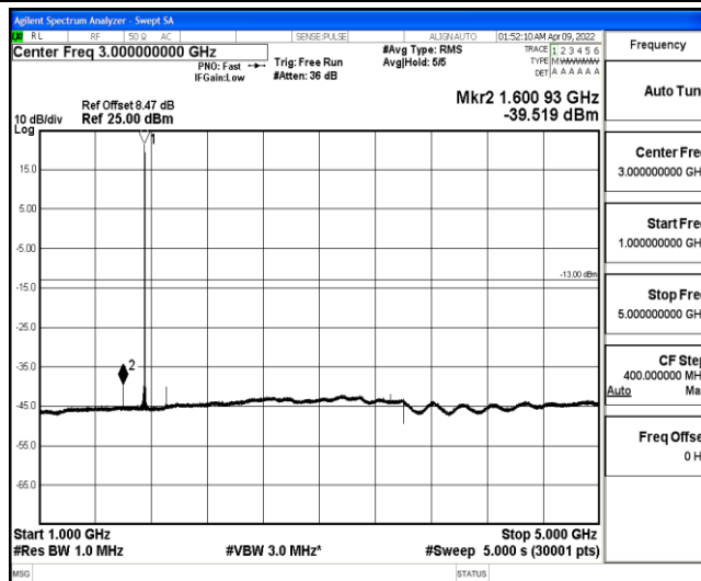
Band4-10MHz-QPSK-20350-1-0-High-1000-5000--39.52-PASS
