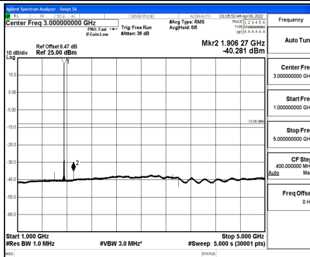
Band4-3MHz-QPSK-20385-1-0-High-1000-5000--40.28-PASS
