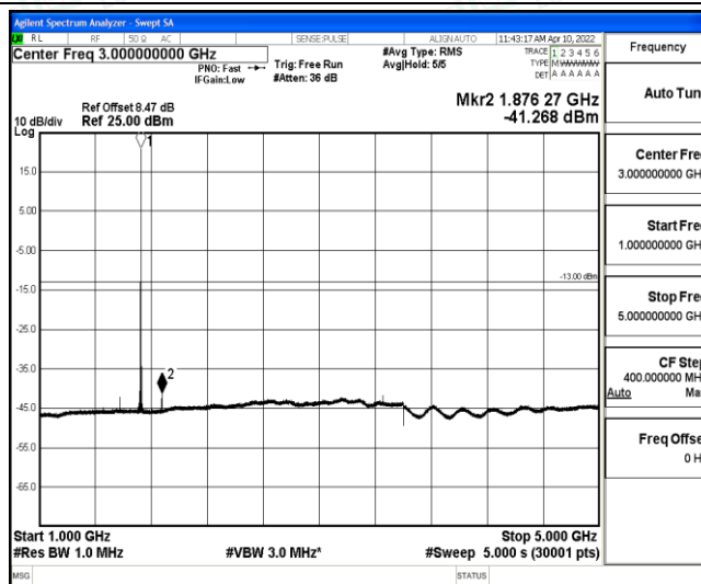
Band4-15MHz-QPSK-20175-1-0-Low-1000-5000--41.27-PASS
