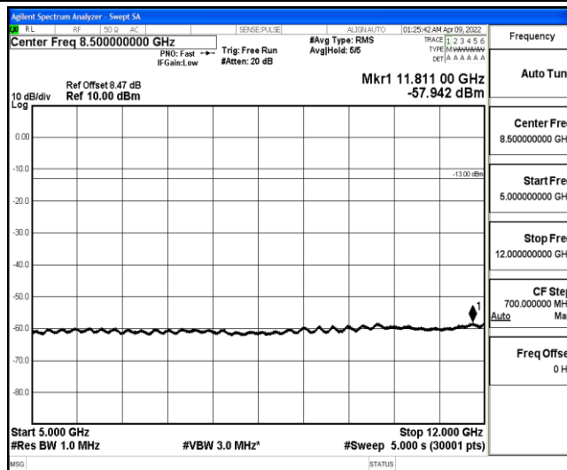
Band4-5MHz-QPSK-20175-1-0-Low-5000-12000--57.94-PASS
