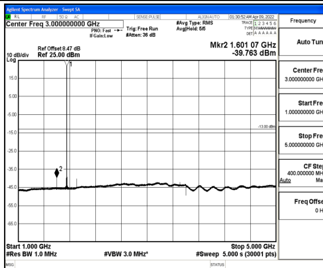
Band4-5MHz-16QAM-20375-1-0-High-1000-5000--39.76-PASS
