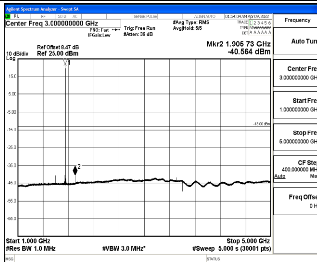
Band4-10MHz-16QAM-20350-1-0-High-1000-5000--40.56-PASS
