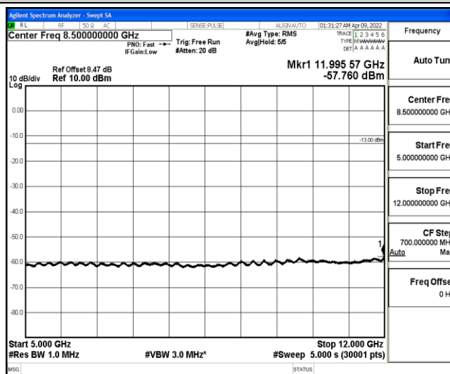
Band4-5MHz-16QAM-20375-1-0-High-5000-12000--57.76-PASS
