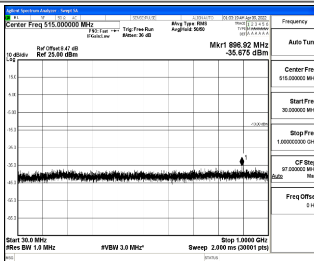
Band4-3MHz-16QAM-20175-1-0-Low-30-1000--35.68-PASS
