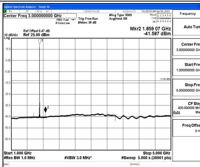
Band4-3MHz-16QAM-19965-1-0-Low-1000-5000--41.59-PASS
