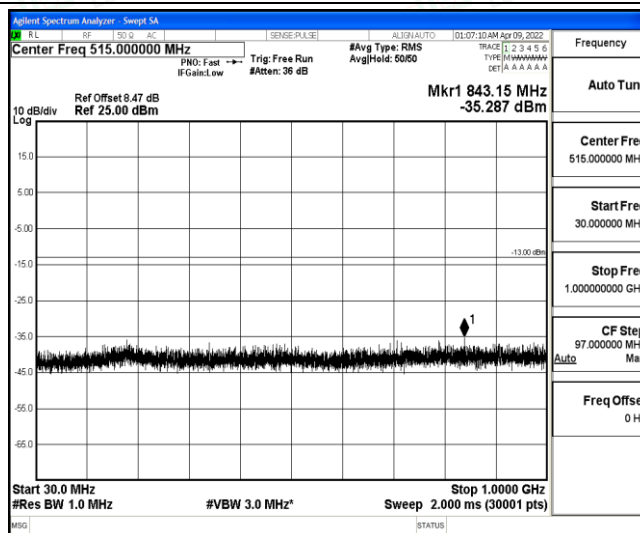
Band4-3MHz-16QAM-20385-1-0-High-30-1000--35.29-PASS
