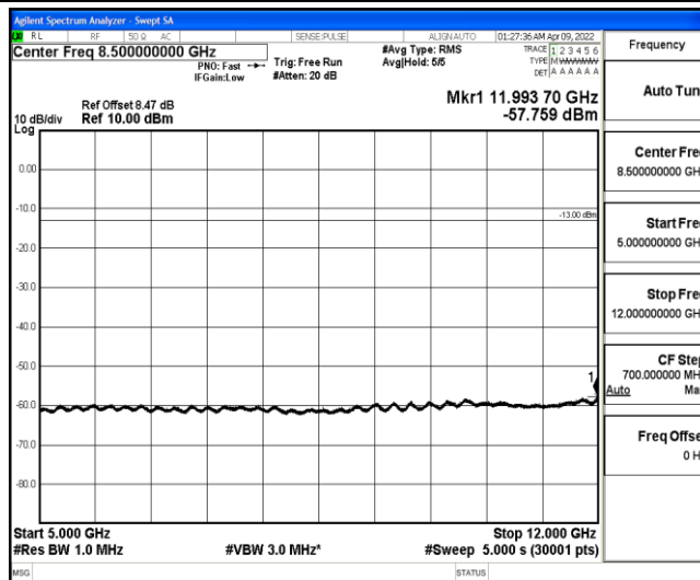
Band4-5MHz-16QAM-20175-1-0-Low-5000-12000--57.76-PASS
