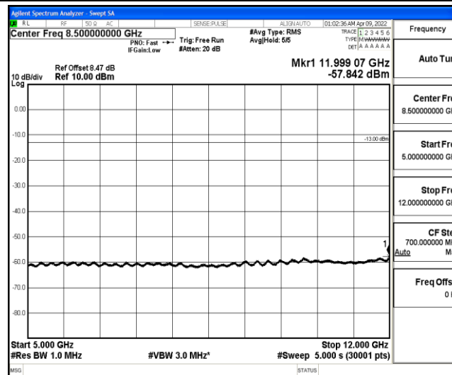
Band4-3MHz-QPSK-20175-1-0-Low-5000-12000--57.84-PASS
