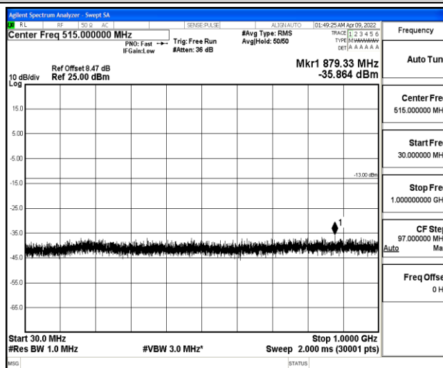
Band4-10MHz-16QAM-20175-1-0-Low-30-1000--35.86-PASS
