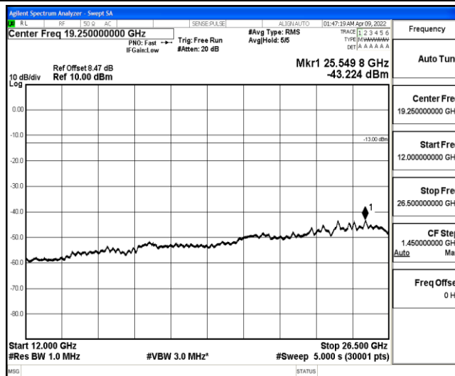
Band4-10MHz-16QAM-20000-1-0-Low-12000-26500--43.22-PASS
