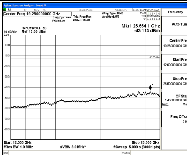
Band4-3MHz-16QAM-19965-1-0-Low-12000-26500--43.11-PASS
