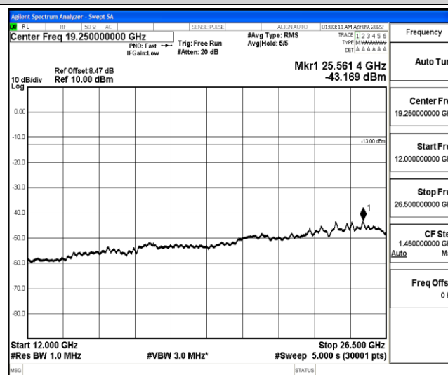
Band4-3MHz-QPSK-20175-1-0-Low-12000-26500--43.17-PASS
