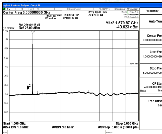
Band4-5MHz-QPSK-20175-1-0-Low-1000-5000--40.62-PASS
