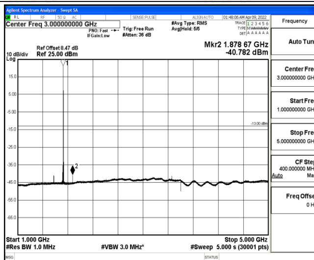
Band4-10MHz-QPSK-20175-1-0-Low-1000-5000--40.78-PASS
