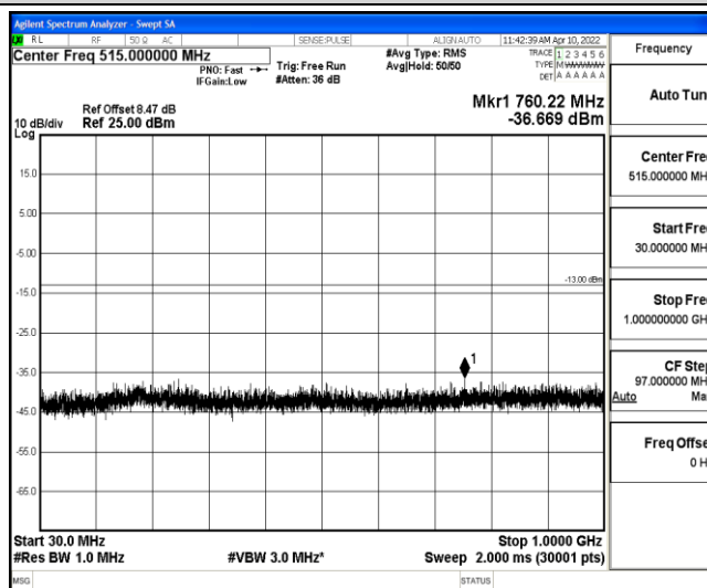
Band4-15MHz-QPSK-20175-1-0-Low-30-1000--36.67-PASS
