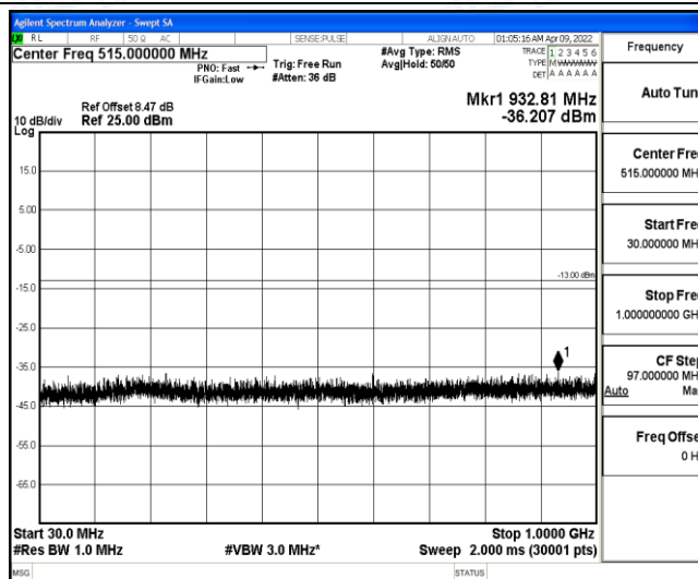
Band4-3MHz-QPSK-20385-1-0-High-30-1000--36.21-PASS
