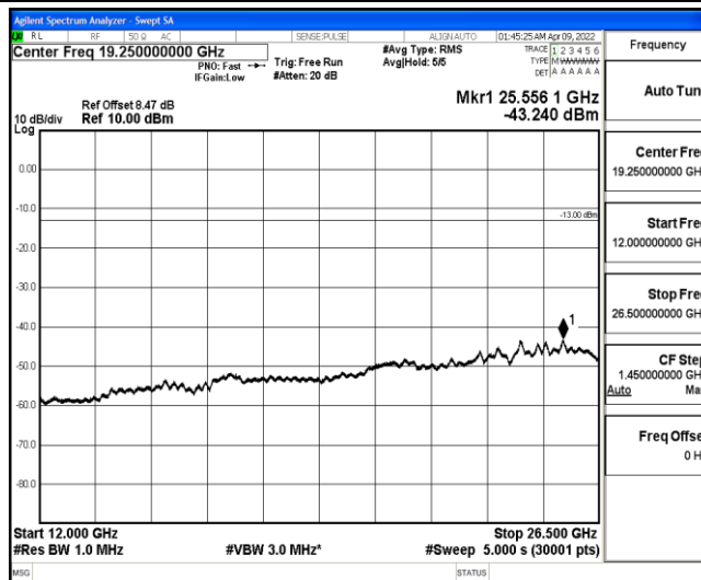
Band4-10MHz-QPSK-20000-1-0-Low-12000-26500--43.24-PASS
