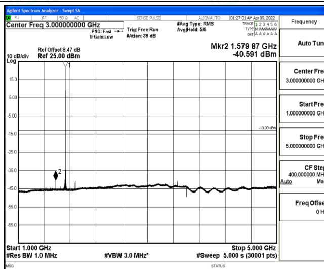
Band4-5MHz-16QAM-20175-1-0-Low-1000-5000--40.59-PASS
