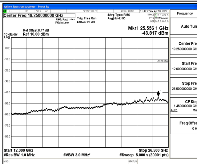
Band4-15MHz-QPSK-20175-1-0-Low-12000-26500--43.82-PASS
