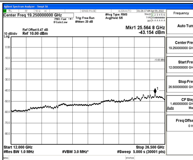
Band4-5MHz-QPSK-20175-1-0-Low-12000-26500--43.15-PASS
