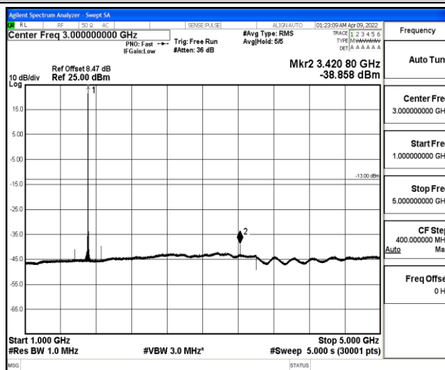
Band4-5MHz-16QAM-19975-1-0-Low-1000-5000--38.86-PASS
