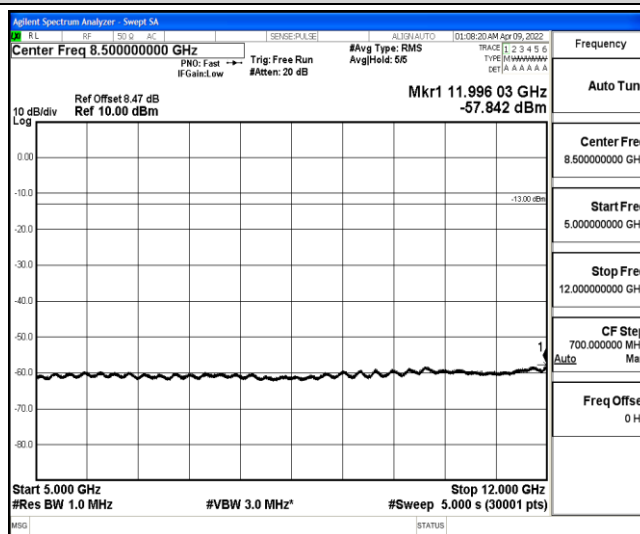
Band4-3MHz-16QAM-20385-1-0-High-5000-12000--57.84-PASS
