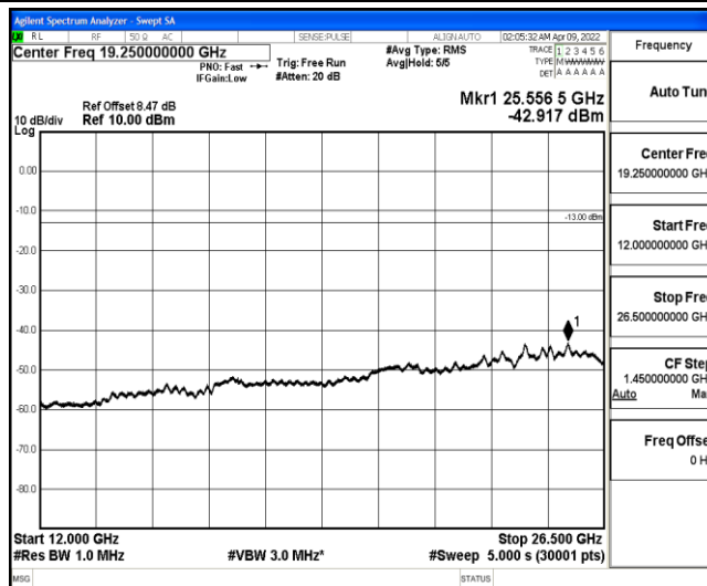
Band4-15MHz-QPSK-20025-1-0-Low-12000-26500--42.92-PASS
