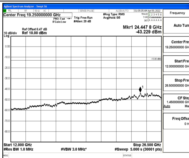
Band4-3MHz-16QAM-20175-1-0-Low-12000-26500--43.23-PASS
