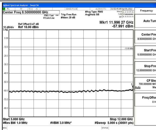
Band4-10MHz-QPSK-20350-1-0-High-5000-12000--57.99-PASS
