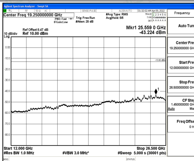
Band4-5MHz-16QAM-20375-1-0-High-12000-26500--43.22-PASS
