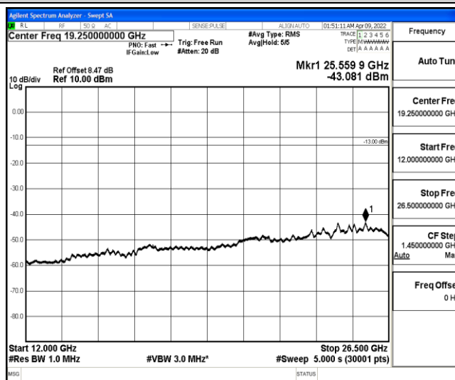
Band4-10MHz-16QAM-20175-1-0-Low-12000-26500--43.08-PASS
