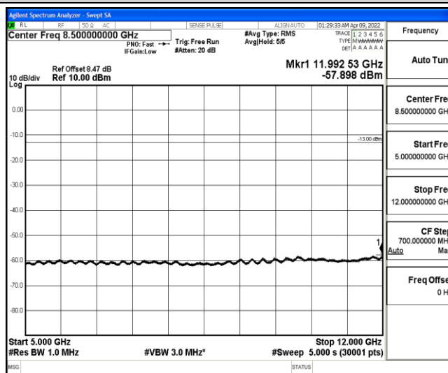
Band4-5MHz-QPSK-20375-1-0-High-5000-12000--57.9-PASS
