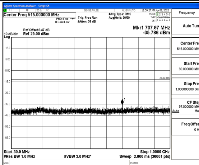
Band4-3MHz-16QAM-19965-1-0-Low-30-1000--35.79-PASS
