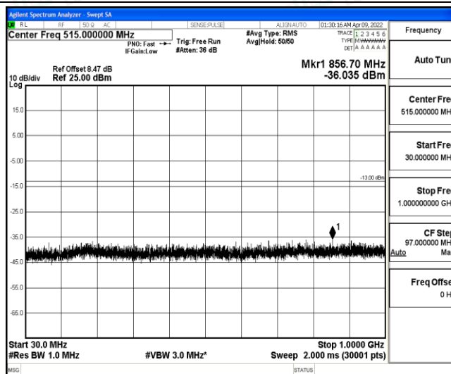
Band4-5MHz-16QAM-20375-1-0-High-30-1000--36.04-PASS
