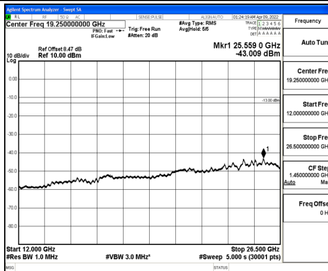
Band4-5MHz-16QAM-19975-1-0-Low-12000-26500--43.01-PASS
