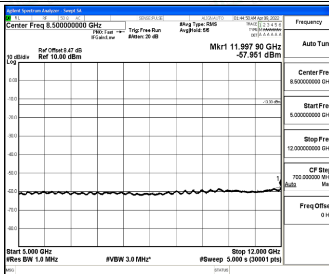
Band4-10MHz-QPSK-20000-1-0-Low-5000-12000--57.95-PASS
