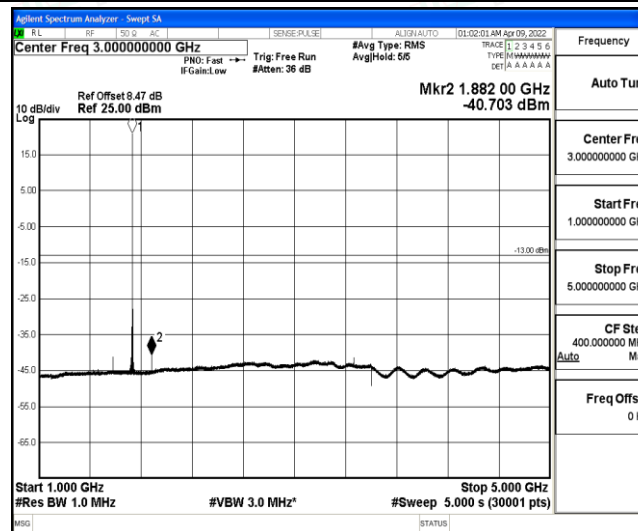
Band4-3MHz-QPSK-20175-1-0-Low-1000-5000--40.7-PASS
