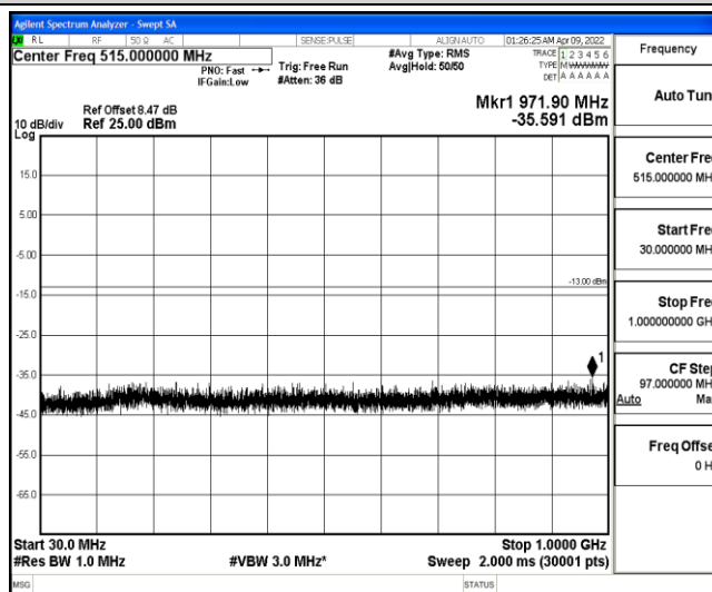
Band4-5MHz-16QAM-20175-1-0-Low-30-1000--35.59-PASS
