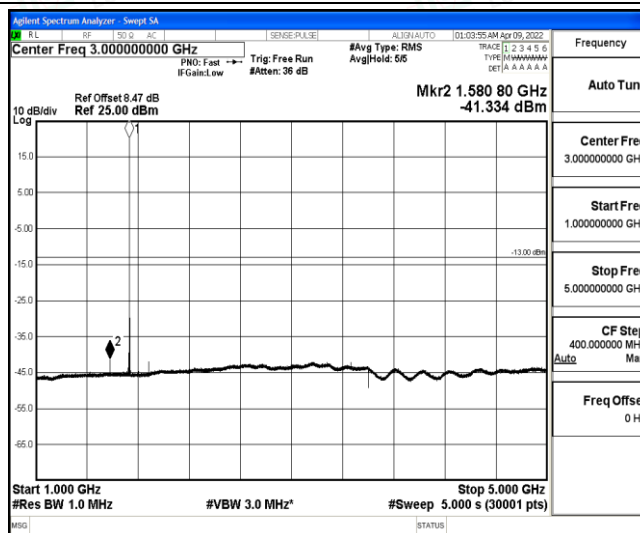
Band4-3MHz-16QAM-20175-1-0-Low-1000-5000--41.33-PASS
