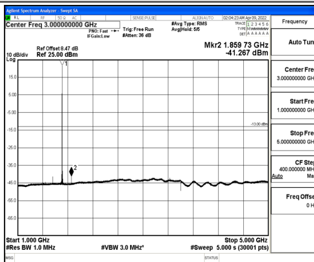
Band4-15MHz-QPSK-20025-1-0-Low-1000-5000--41.27-PASS
