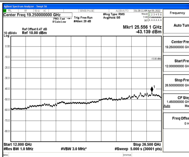
Band4-5MHz-16QAM-20175-1-0-Low-12000-26500--43.14-PASS
