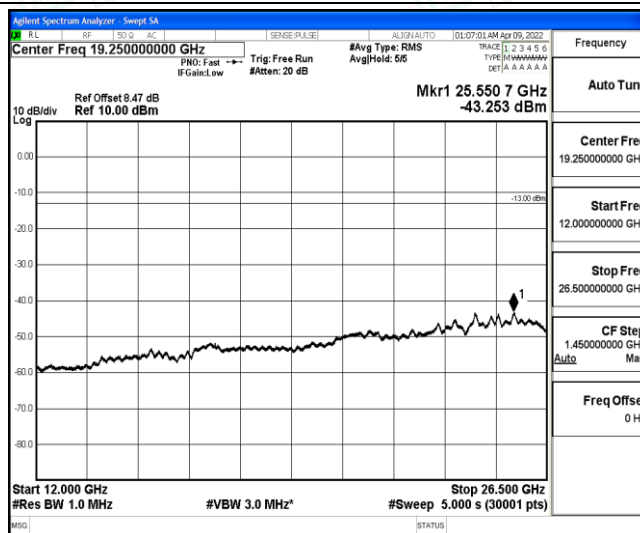
Band4-3MHz-QPSK-20385-1-0-High-12000-26500--43.25-PASS
