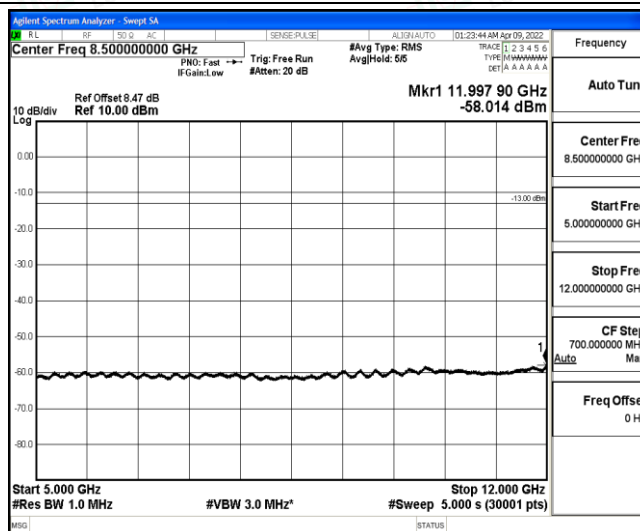
Band4-5MHz-16QAM-19975-1-0-Low-5000-12000--58.01-PASS
