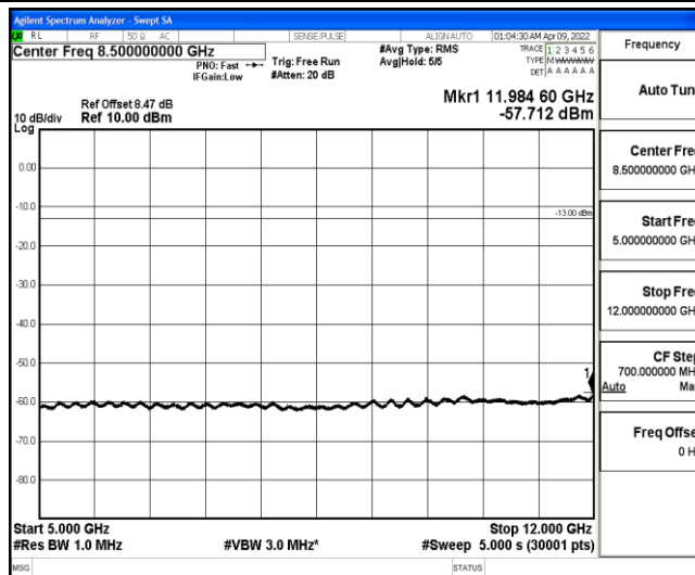
Band4-3MHz-16QAM-20175-1-0-Low-5000-12000--57.71-PASS
