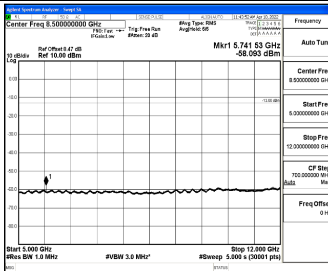
Band4-15MHz-QPSK-20175-1-0-Low-5000-12000--58.09-PASS
