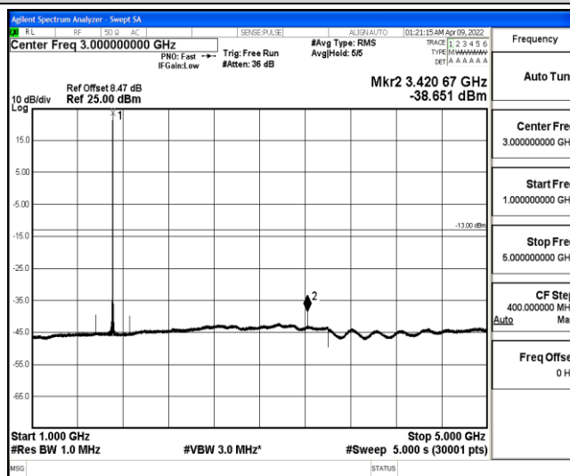
Band4-5MHz-QPSK-19975-1-0-Low-1000-5000--38.65-PASS
