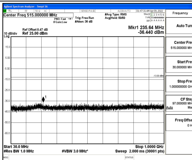
Band4-10MHz-QPSK-20175-1-0-Low-30-1000--36.44-PASS
