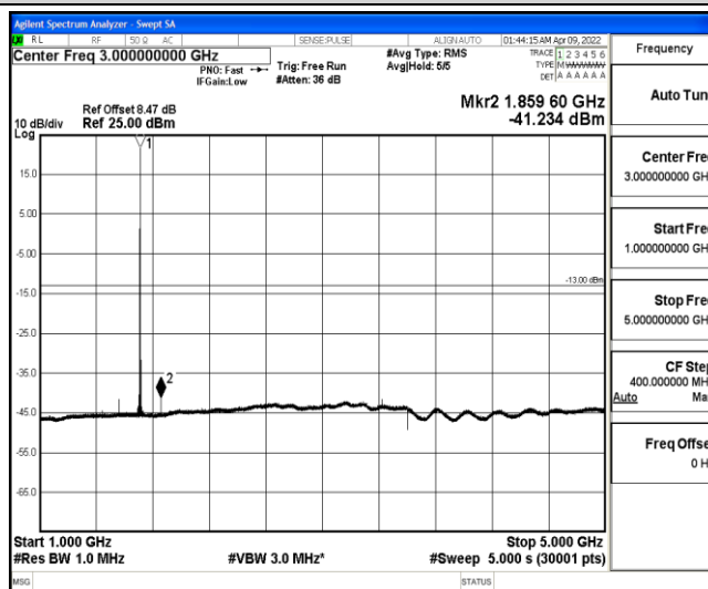
Band4-10MHz-QPSK-20000-1-0-Low-1000-5000--41.23-PASS
