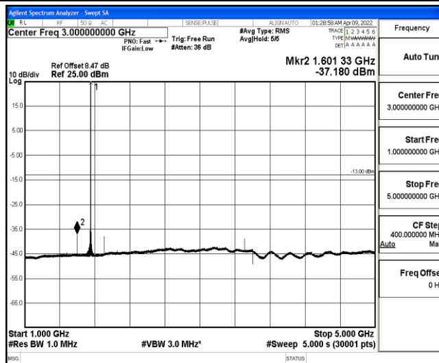
Band4-5MHz-QPSK-20375-1-0-High-1000-5000--37.18-PASS
