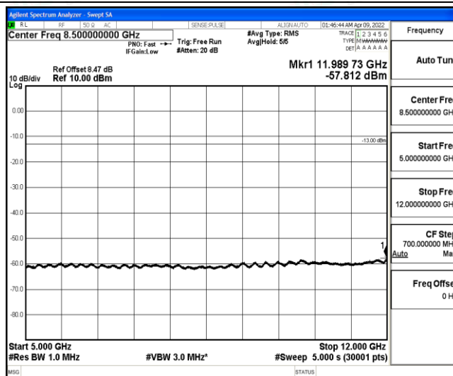
Band4-10MHz-16QAM-20000-1-0-Low-5000-12000--57.81-PASS
