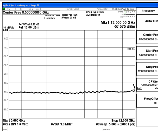
Band4-3MHz-QPSK-20385-1-0-High-5000-12000--57.58-PASS
