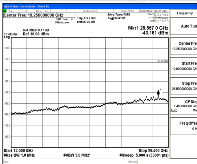
Band4-3MHz-16QAM-20385-1-0-High-12000-26500--43.18-PASS
