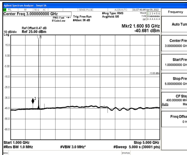
Band4-3MHz-16QAM-20385-1-0-High-1000-5000--40.68-PASS
