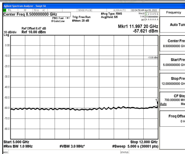
Band4-15MHz-QPSK-20025-1-0-Low-5000-12000--57.62-PASS
