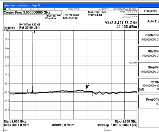
Band4-10MHz-16QAM-20000-1-0-Low-1000-5000--41.14-PASS
