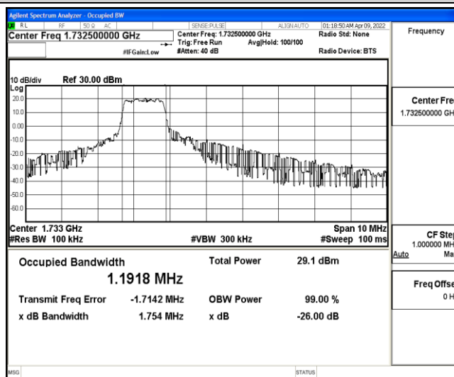
Band4-5MHz-QPSK-20175-6-0-Low-1.1918-1.754-PASS
