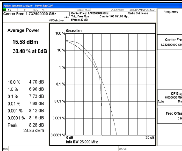
Band4-1.4MHz-QPSK-20175-6-0-Low-7.73-&lt;=13-PASS
