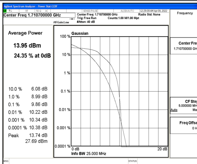
Band4-1.4MHz-QPSK-19957-6-0-Low-9.86-&lt;=13-PASS
