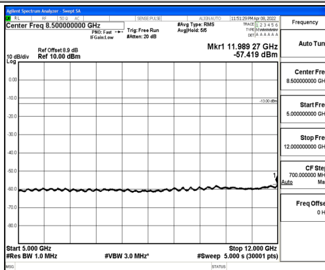
Band2-20MHz-16QAM-19100-1-0-High-5000-12000--57.42-PASS
