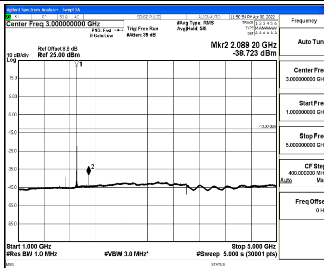
Band2-20MHz-16QAM-19100-1-0-High-1000-5000--38.72-PASS
