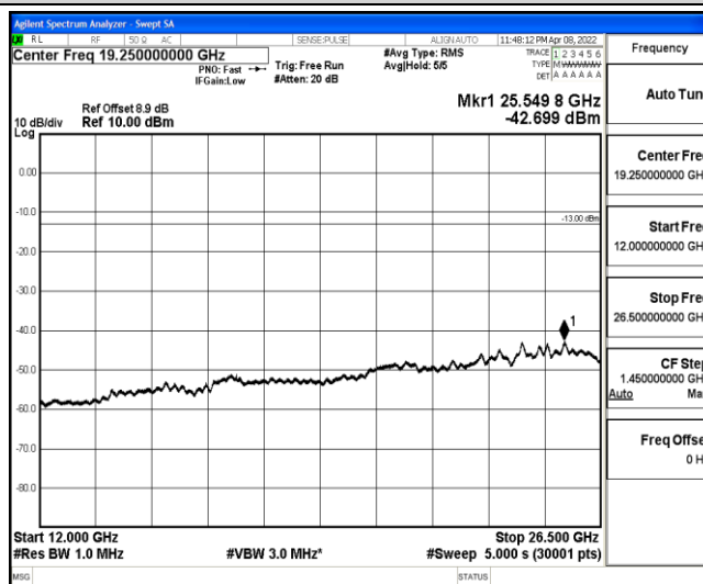
Band2-20MHz-16QAM-18900-1-0-Low-12000-26500--42.7-PASS
