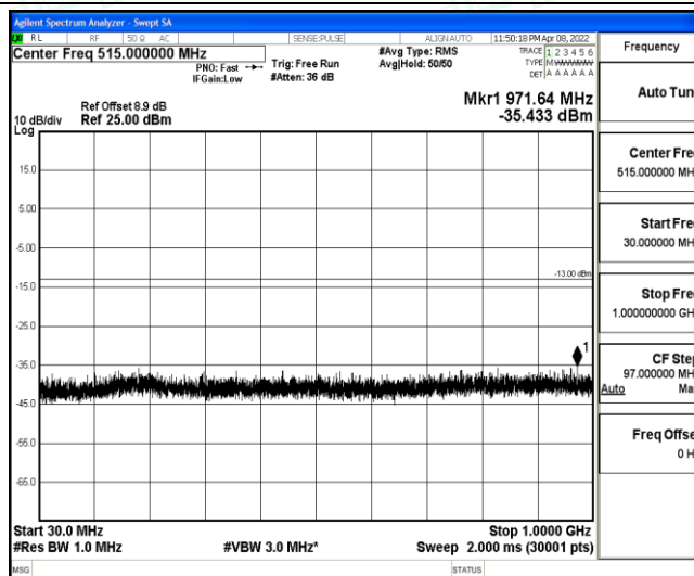
Band2-20MHz-16QAM-19100-1-0-High-30-1000--35.43-PASS
