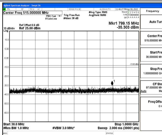
Band2-20MHz-16QAM-18900-1-0-Low-30-1000--35.3-PASS
