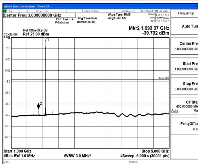
Band2-20MHz-16QAM-18900-1-0-Low-1000-5000--39.7-PASS
