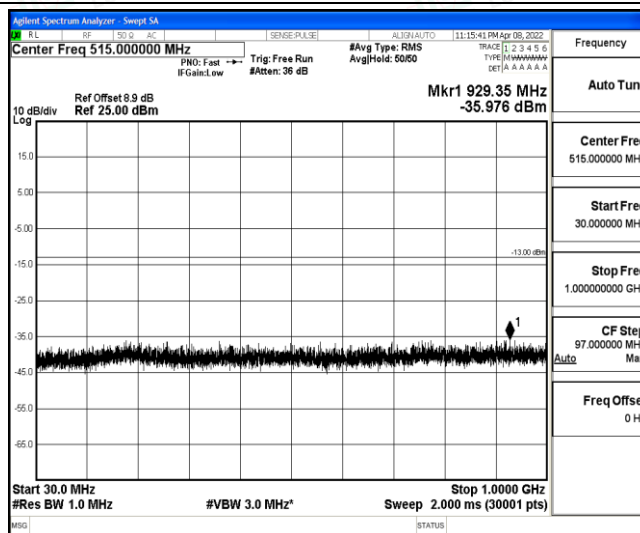
Band2-15MHz-16QAM-19125-1-0-High-30-1000--35.98-PASS
