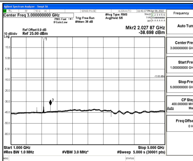
Band2-20MHz-QPSK-18700-1-0-Low-1000-5000--38.7-PASS
