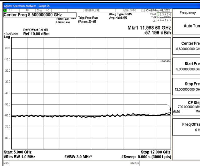
Band2-20MHz-QPSK-18900-1-0-Low-5000-12000--57.2-PASS
