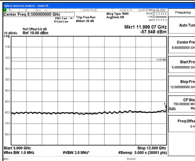
Band2-20MHz-16QAM-18900-1-0-Low-5000-12000--57.55-PASS
