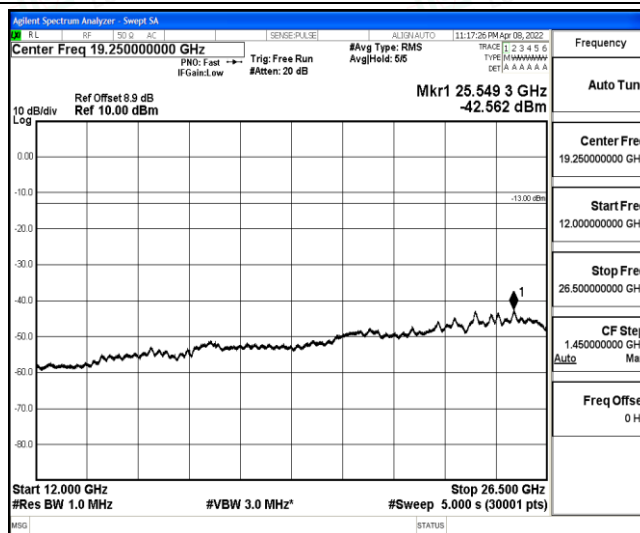
Band2-15MHz-16QAM-19125-1-0-High-12000-26500--42.56-PASS
