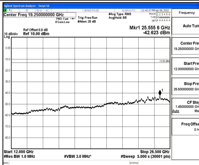
Band2-20MHz-QPSK-18700-1-0-Low-12000-26500--42.62-PASS
