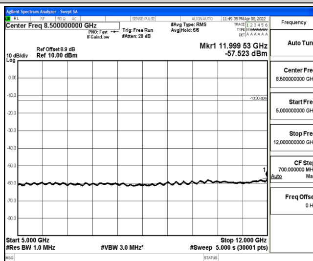
Band2-20MHz-QPSK-19100-1-0-High-5000-12000--57.52-PASS
