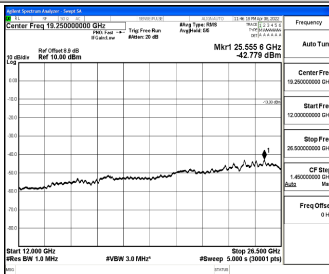
Band2-20MHz-QPSK-18900-1-0-Low-12000-26500--42.78-PASS
