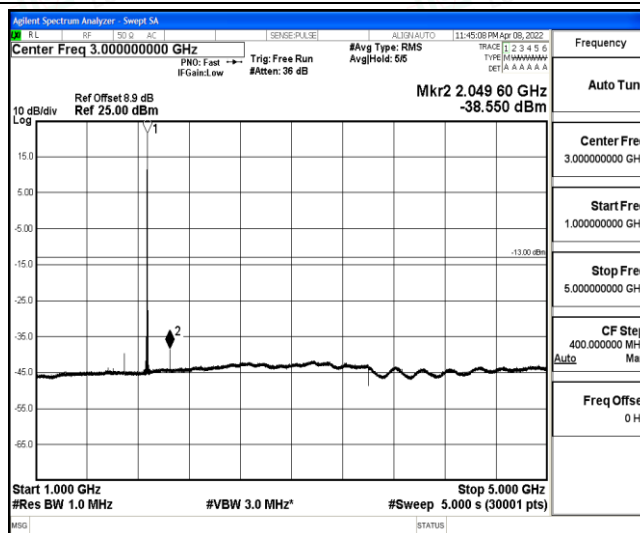
Band2-20MHz-QPSK-18900-1-0-Low-1000-5000--38.55-PASS
