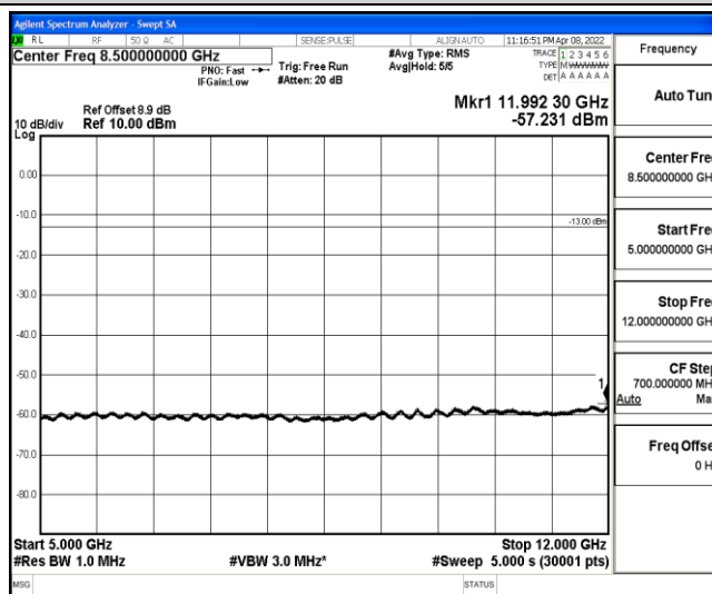
Band2-15MHz-16QAM-19125-1-0-High-5000-12000--57.23-PASS
