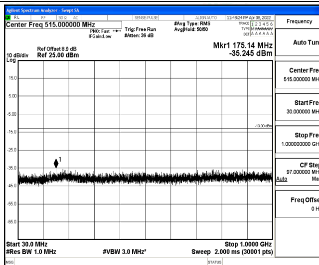
Band2-20MHz-QPSK-19100-1-0-High-30-1000--35.25-PASS
