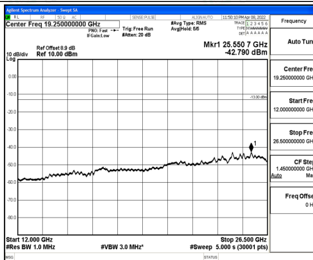
Band2-20MHz-QPSK-19100-1-0-High-12000-26500--42.79-PASS
