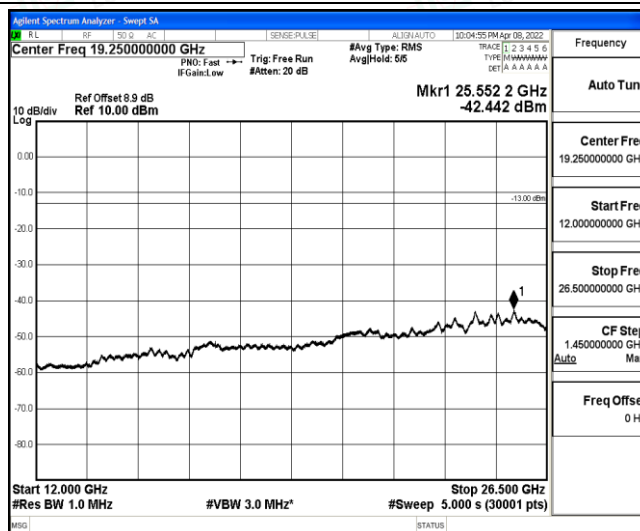
Band2-3MHz-16QAM-19185-1-0-High-12000-26500--42.44-PASS
