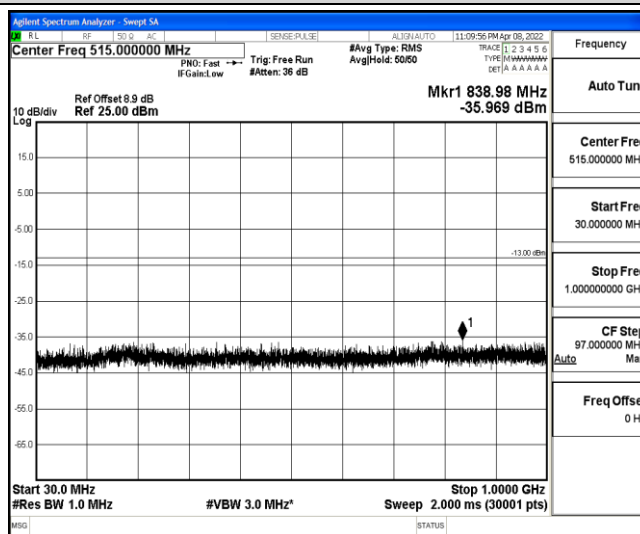
Band2-15MHz-QPSK-18900-1-0-Low-30-1000--35.97-PASS
