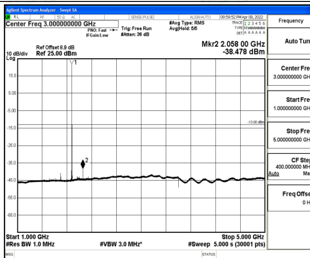
Band2-3MHz-16QAM-18900-1-0-Low-1000-5000--38.48-PASS
