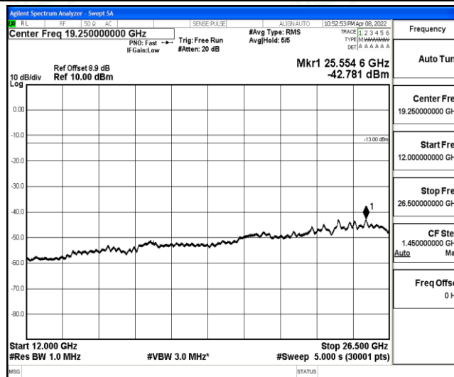
Band2-10MHz-16QAM-19150-1-0-High-12000-26500--42.78-PASS
