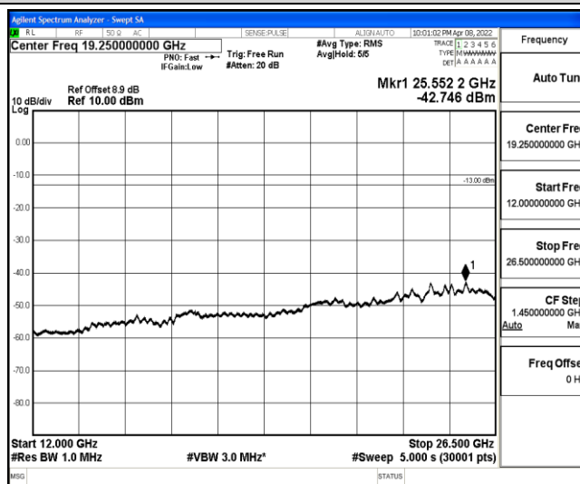
Band2-3MHz-16QAM-18900-1-0-Low-12000-26500--42.75-PASS
