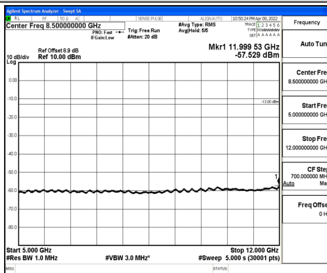
Band2-10MHz-QPSK-19150-1-0-High-5000-12000--57.53-PASS
