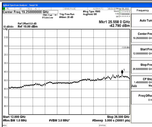
Band2-5MHz-16QAM-18625-1-0-Low-12000-26500--42.79-PASS
