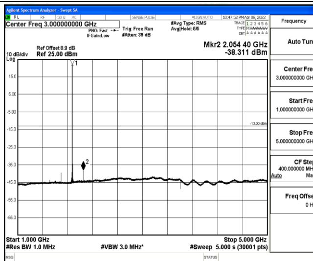
Band2-10MHz-16QAM-18900-1-0-Low-1000-5000--38.31-PASS
