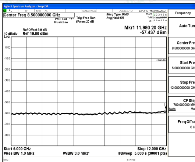
Band2-10MHz-QPSK-18650-1-0-Low-5000-12000--57.44-PASS
