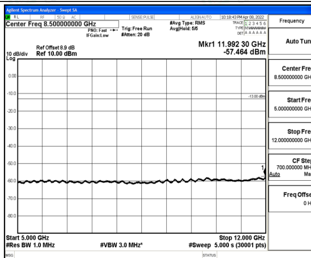
Band2-5MHz-QPSK-18625-1-0-Low-5000-12000--57.46-PASS
