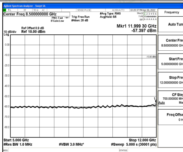
Band2-5MHz-16QAM-18625-1-0-Low-5000-12000--57.4-PASS
