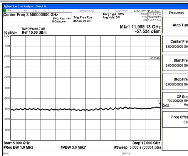
Band2-10MHz-16QAM-19150-1-0-High-5000-12000--57.53-PASS
