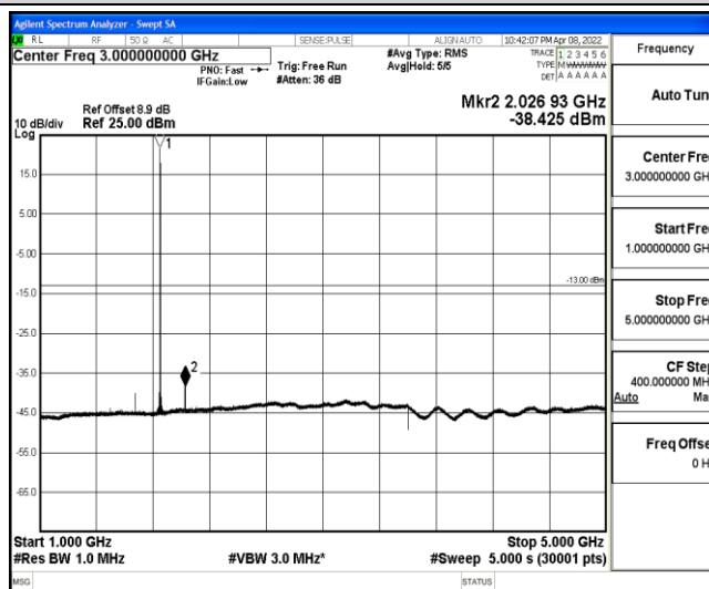
Band2-10MHz-QPSK-18650-1-0-Low-1000-5000--38.43-PASS
