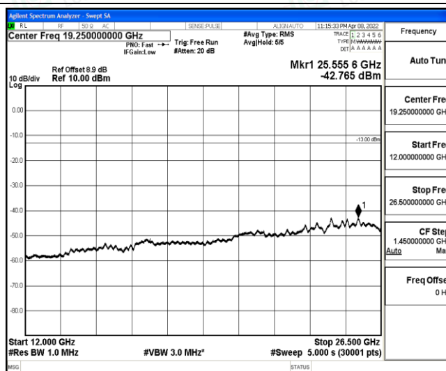
Band2-15MHz-QPSK-19125-1-0-High-12000-26500--42.77-PASS
