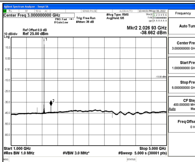
Band2-10MHz-16QAM-18650-1-0-Low-1000-5000--38.66-PASS
