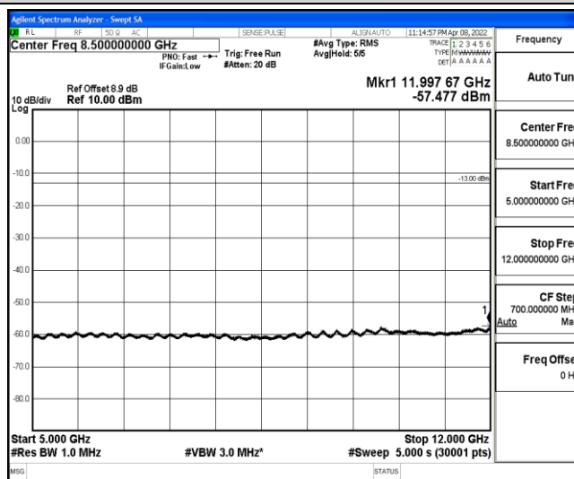
Band2-15MHz-QPSK-19125-1-0-High-5000-12000--57.48-PASS
