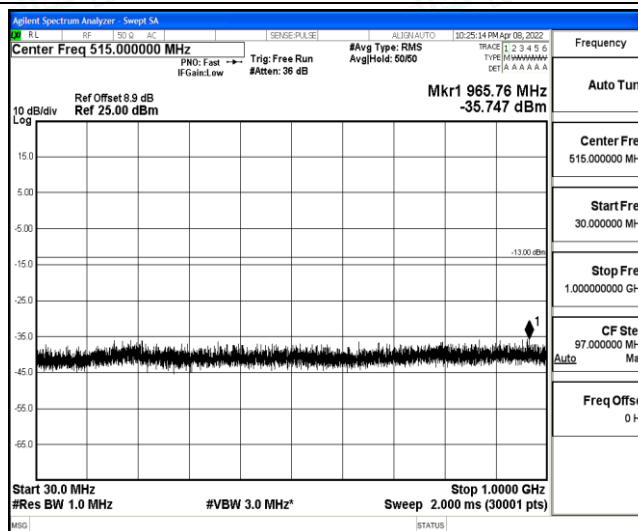
Band2-5MHz-QPSK-19175-1-0-High-30-1000--35.75-PASS
