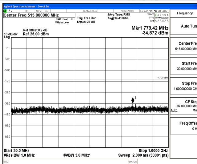
Band2-15MHz-QPSK-19125-1-0-High-30-1000--34.87-PASS
