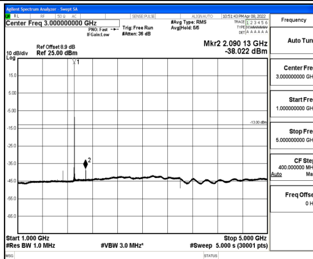
Band2-10MHz-16QAM-19150-1-0-High-1000-5000--38.02-PASS
