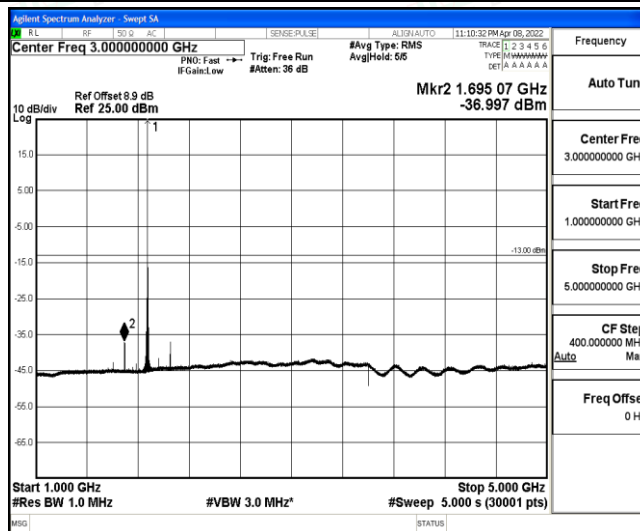
Band2-15MHz-QPSK-18900-1-0-Low-1000-5000--37-PASS
