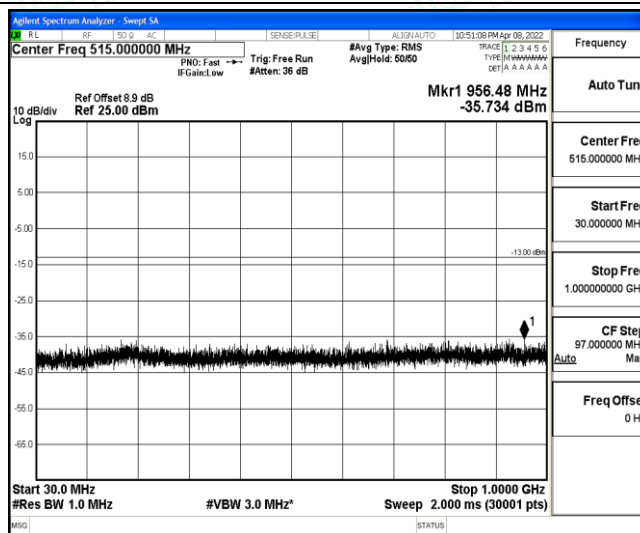
Band2-10MHz-16QAM-19150-1-0-High-30-1000--35.73-PASS
