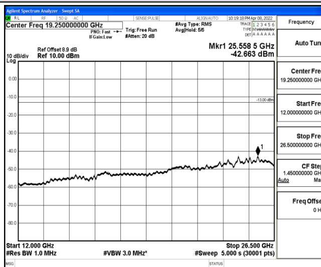
Band2-5MHz-QPSK-18625-1-0-Low-12000-26500--42.66-PASS
