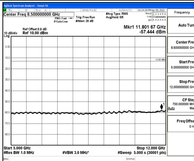
Band2-5MHz-16QAM-18900-1-0-Low-5000-12000--57.44-PASS
