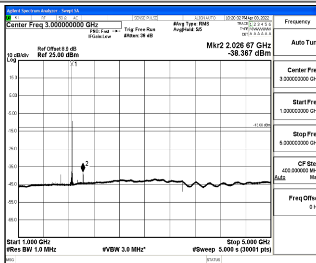
Band2-5MHz-16QAM-18625-1-0-Low-1000-5000--38.37-PASS
