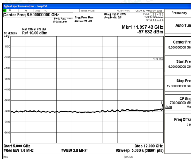
Band2-3MHz-16QAM-18615-1-0-Low-5000-12000--57.53-PASS
