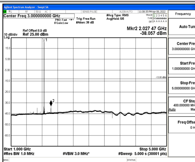
Band2-15MHz-16QAM-18675-1-0-Low-1000-5000--38.06-PASS
