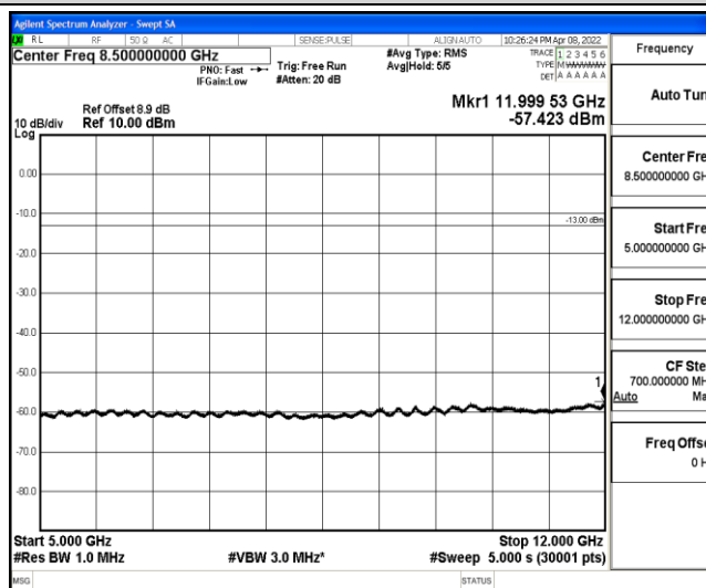
Band2-5MHz-QPSK-19175-1-0-High-5000-12000--57.42-PASS
