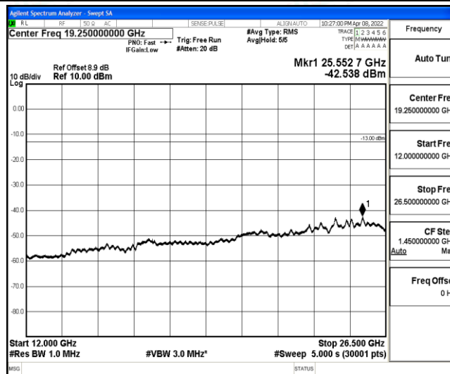
Band2-5MHz-QPSK-19175-1-0-High-12000-26500--42.54-PASS
