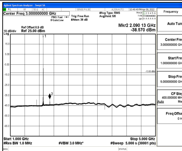
Band2-10MHz-QPSK-19150-1-0-High-1000-5000--38.57-PASS
