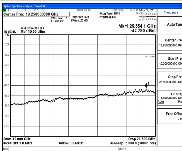
Band2-15MHz-QPSK-18900-1-0-Low-12000-26500--42.78-PASS
