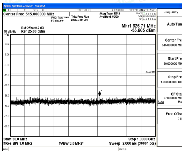
Band2-3MHz-16QAM-19185-1-0-High-30-1000--35.87-PASS
