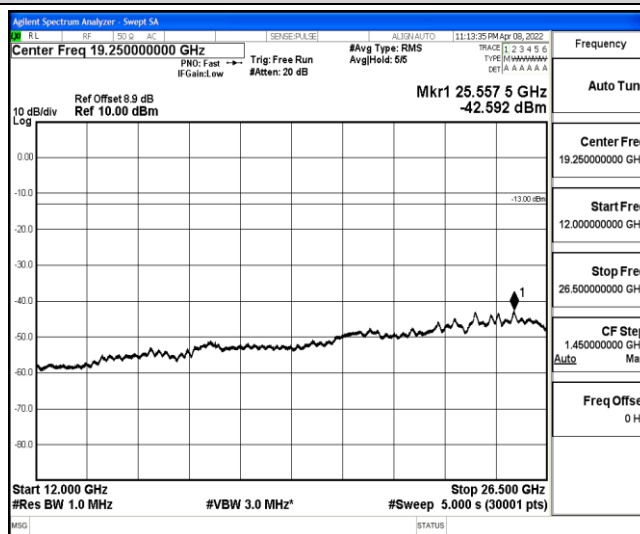
Band2-15MHz-16QAM-18900-1-0-Low-12000-26500--42.59-PASS
