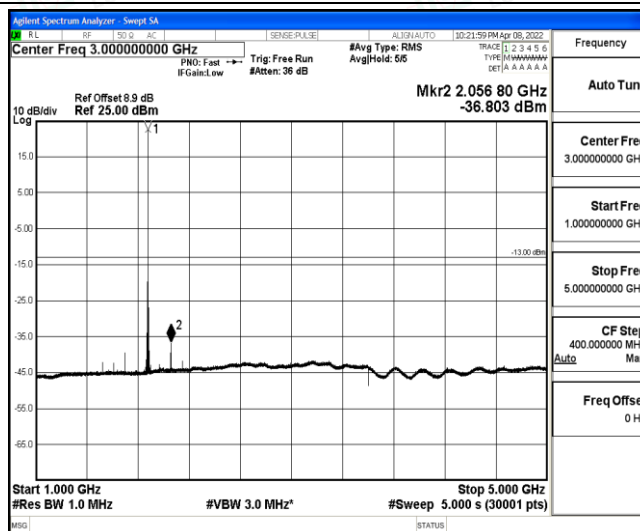
Band2-5MHz-QPSK-18900-1-0-Low-1000-5000--36.8-PASS
