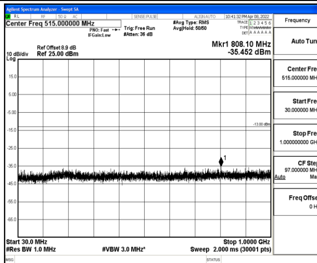
Band2-10MHz-QPSK-18650-1-0-Low-30-1000--35.45-PASS
