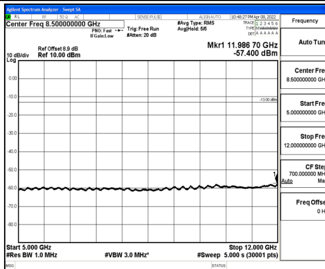
Band2-10MHz-16QAM-18900-1-0-Low-5000-12000--57.4-PASS
