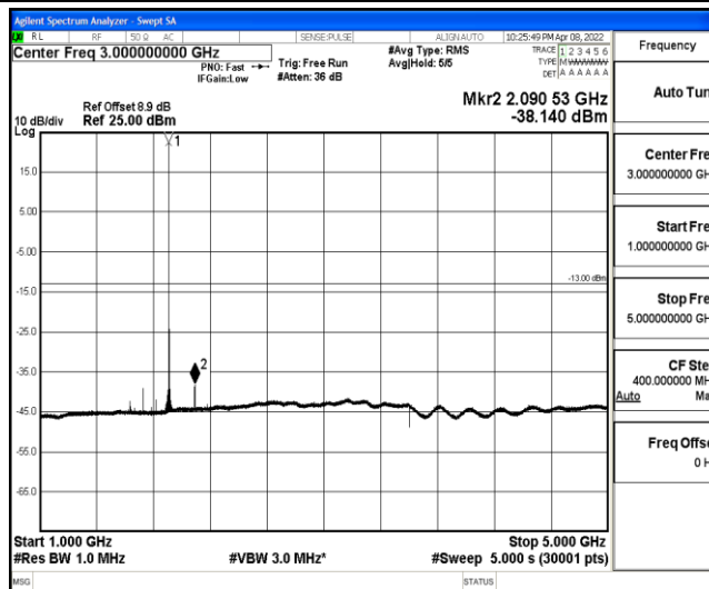
Band2-5MHz-QPSK-19175-1-0-High-1000-5000--38.14-PASS
