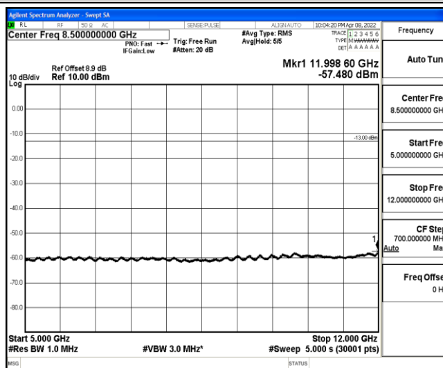
Band2-3MHz-16QAM-19185-1-0-High-5000-12000--57.48-PASS
