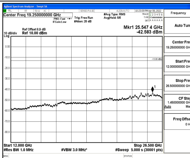
Band2-5MHz-QPSK-18900-1-0-Low-12000-26500--42.58-PASS
