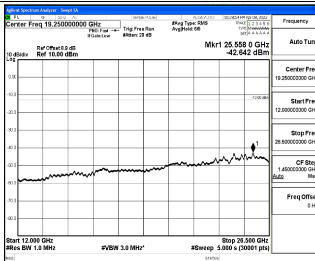
Band2-5MHz-16QAM-19175-1-0-High-12000-26500--42.64-PASS
