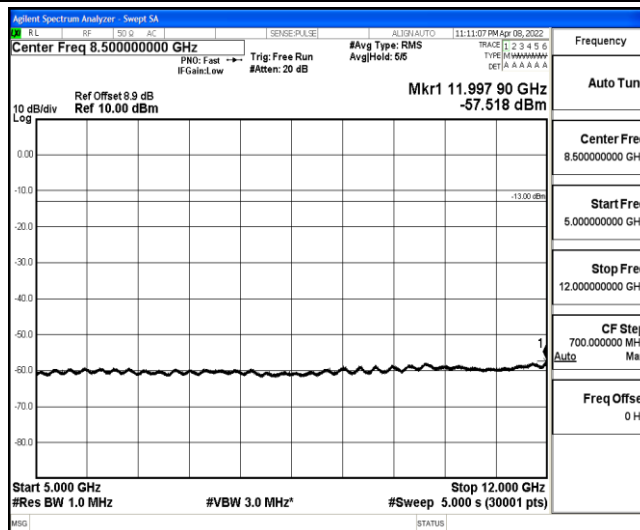
Band2-15MHz-QPSK-18900-1-0-Low-5000-12000--57.52-PASS
