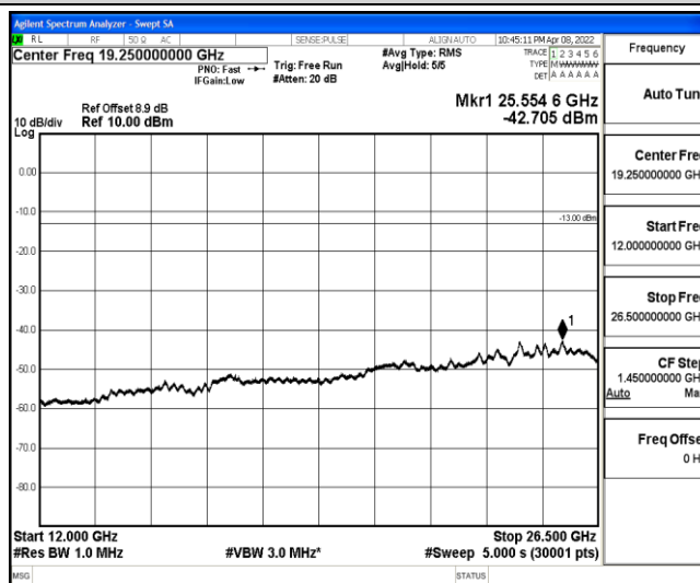
Band2-10MHz-16QAM-18650-1-0-Low-12000-26500--42.71-PASS
