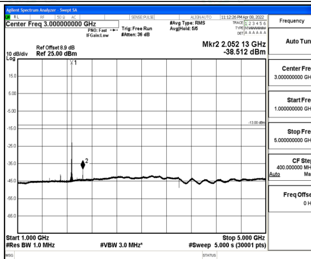
Band2-15MHz-16QAM-18900-1-0-Low-1000-5000--38.51-PASS
