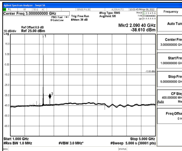
Band2-3MHz-16QAM-19185-1-0-High-1000-5000--38.61-PASS
