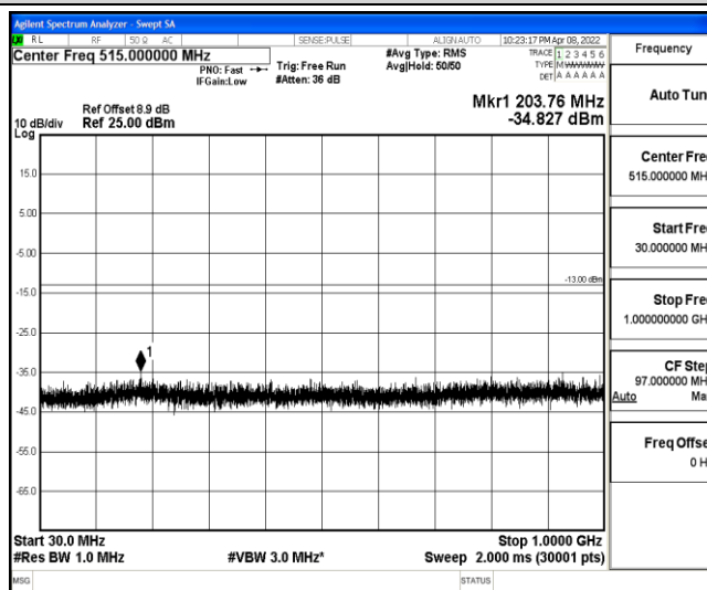
Band2-5MHz-16QAM-18900-1-0-Low-30-1000--34.83-PASS
