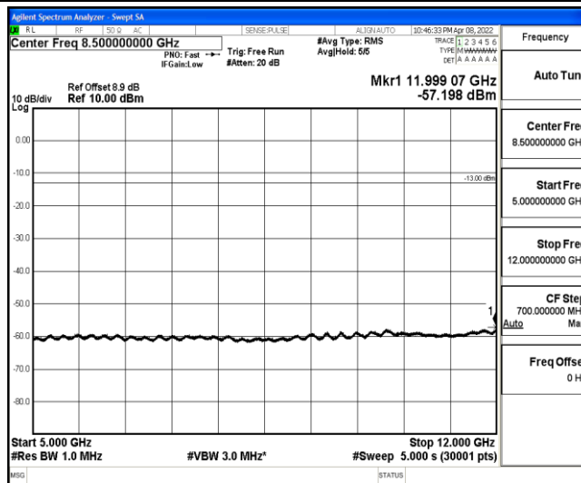
Band2-10MHz-QPSK-18900-1-0-Low-5000-12000--57.2-PASS
