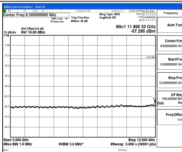
Band2-5MHz-16QAM-19175-1-0-High-5000-12000--57.3-PASS
