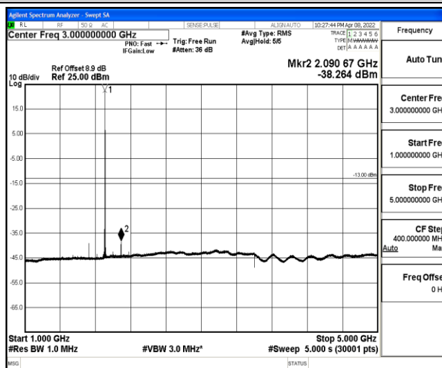
Band2-5MHz-16QAM-19175-1-0-High-1000-5000--38.26-PASS
