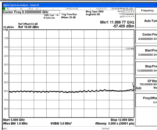
Band2-10MHz-16QAM-18650-1-0-Low-5000-12000--57.41-PASS
