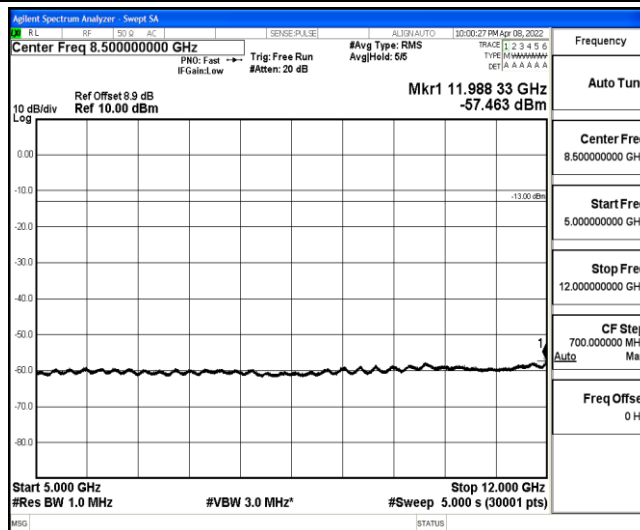
Band2-3MHz-16QAM-18900-1-0-Low-5000-12000--57.46-PASS
