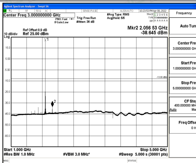
Band2-5MHz-16QAM-18900-1-0-Low-1000-5000--38.65-PASS
