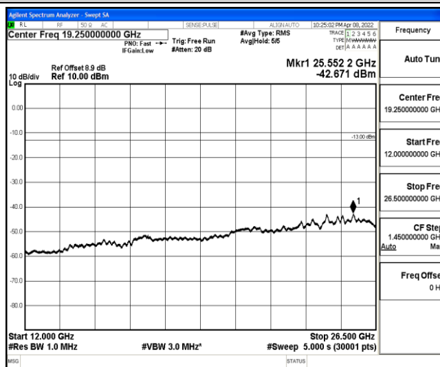
Band2-5MHz-16QAM-18900-1-0-Low-12000-26500--42.67-PASS
