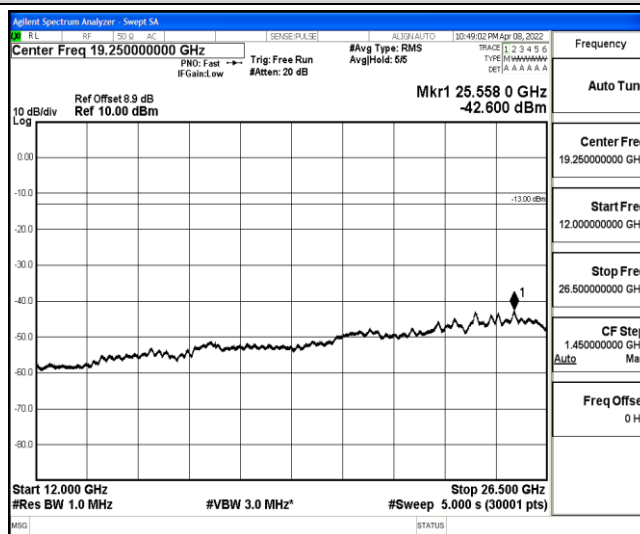
Band2-10MHz-16QAM-18900-1-0-Low-12000-26500--42.6-PASS
