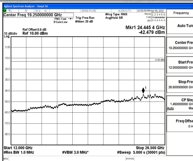
Band2-10MHz-QPSK-19150-1-0-High-12000-26500--42.48-PASS
