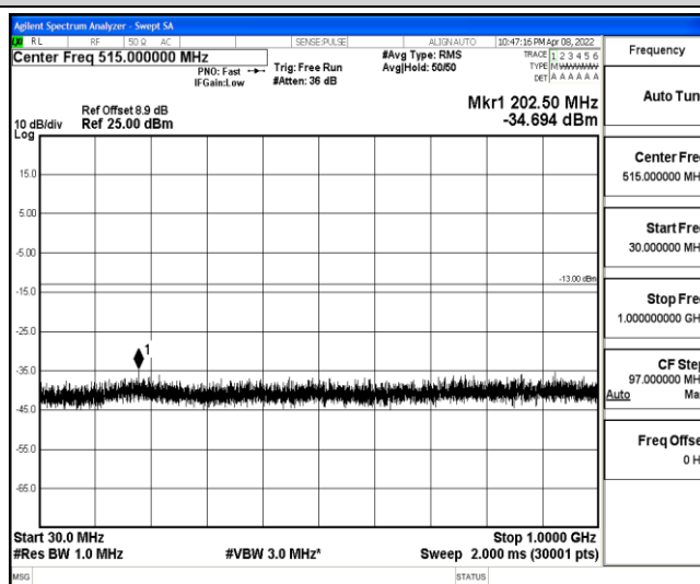
Band2-10MHz-16QAM-18900-1-0-Low-30-1000--34.69-PASS
