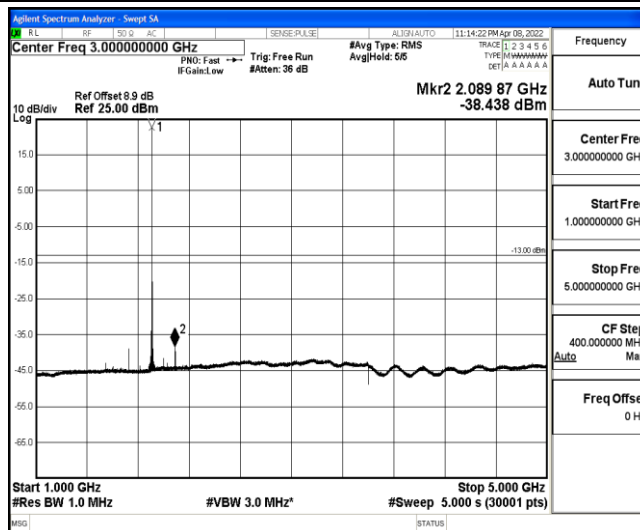
Band2-15MHz-QPSK-19125-1-0-High-1000-5000--38.44-PASS
