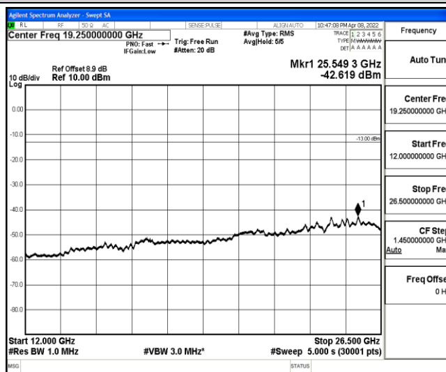
Band2-10MHz-QPSK-18900-1-0-Low-12000-26500--42.62-PASS
