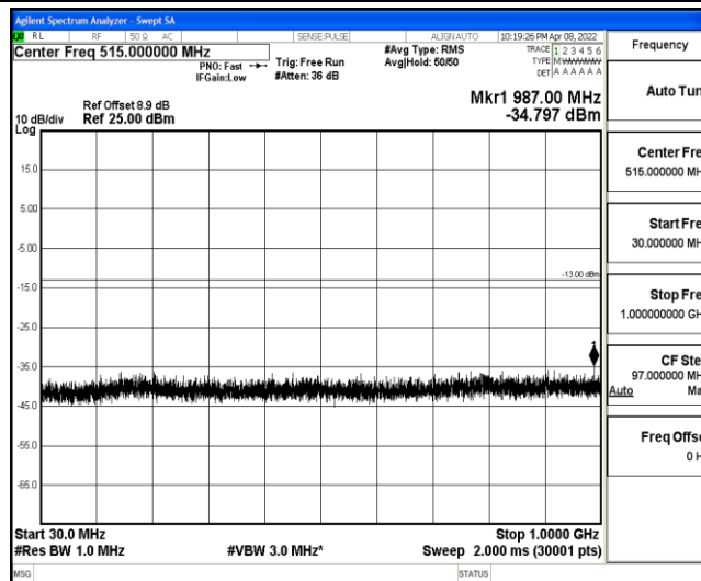
Band2-5MHz-16QAM-18625-1-0-Low-30-1000--34.8-PASS
