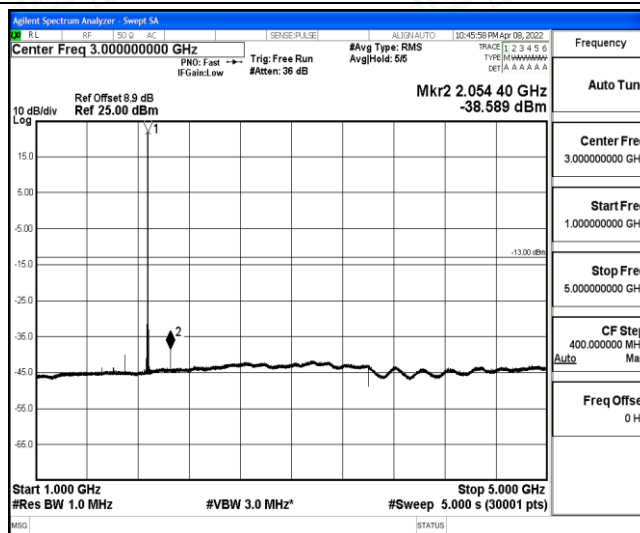
Band2-10MHz-QPSK-18900-1-0-Low-1000-5000--38.59-PASS
