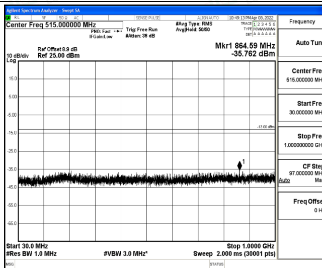
Band2-10MHz-QPSK-19150-1-0-High-30-1000--35.76-PASS
