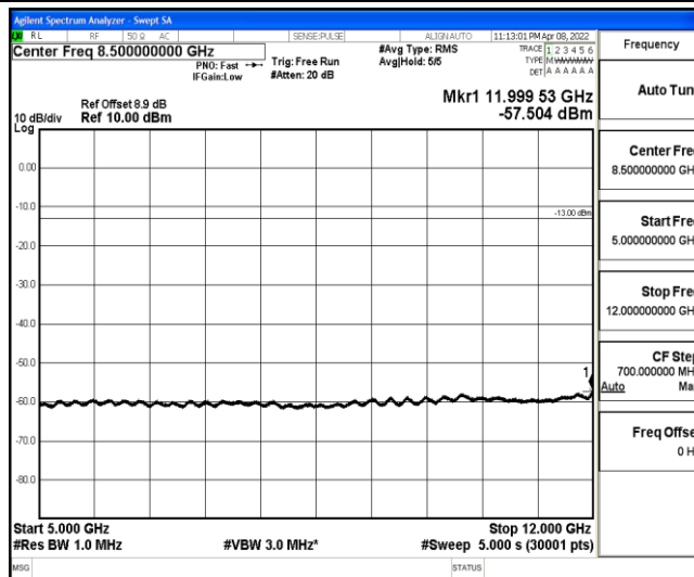
Band2-15MHz-16QAM-18900-1-0-Low-5000-12000--57.5-PASS
