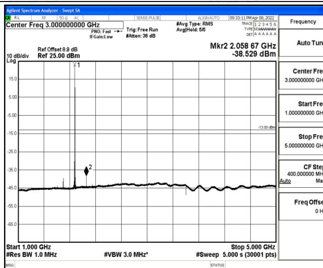
Band2-1.4MHz-QPSK-18900-1-0-Low-1000-5000--38.53-PASS
