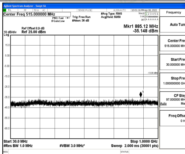
Band2-3MHz-QPSK-19185-1-0-High-30-1000--35.15-PASS
