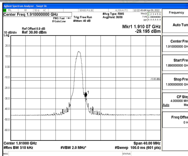
Band2-20MHz-QPSK-19100-6-0-High--29.20-PASS
