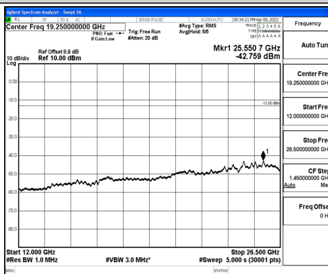
Band2-1.4MHz-QPSK-18900-1-0-Low-12000-26500--42.76-PASS
