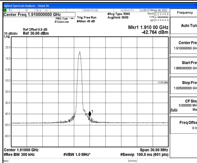
Band2-15MHz-16QAM-19125-1-0-High--42.76-PASS
