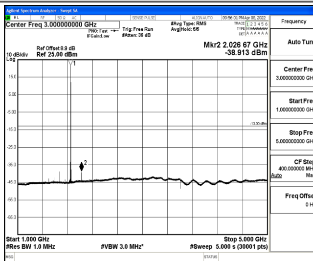
Band2-3MHz-16QAM-18615-1-0-Low-1000-5000--38.91-PASS
