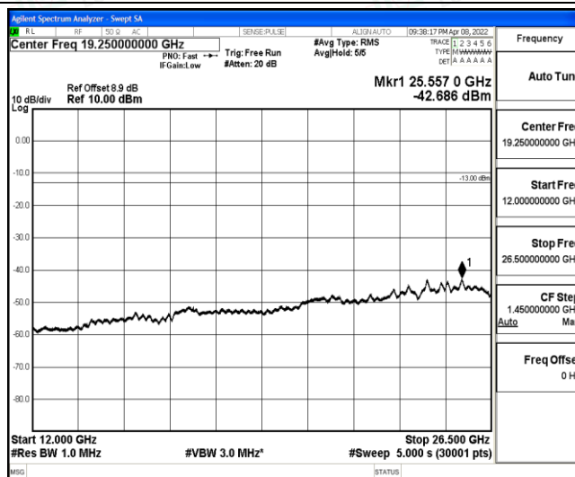
Band2-1.4MHz-QPSK-19193-1-0-High-12000-26500--42.69-PASS
