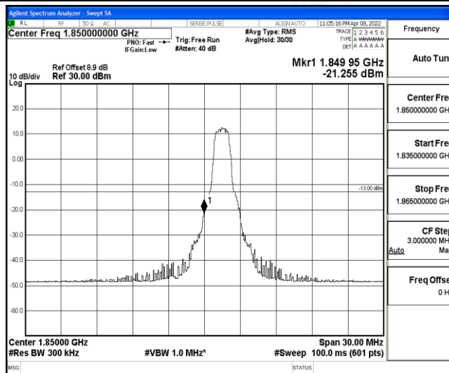
Band2-15MHz-16QAM-18675-6-0-Low--21.26-PASS
