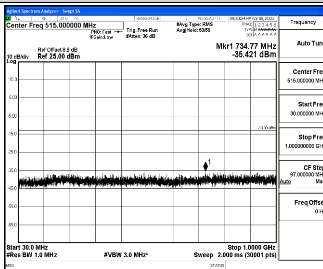
Band2-1.4MHz-16QAM-18607-1-0-Low-30-1000--35.42-PASS
