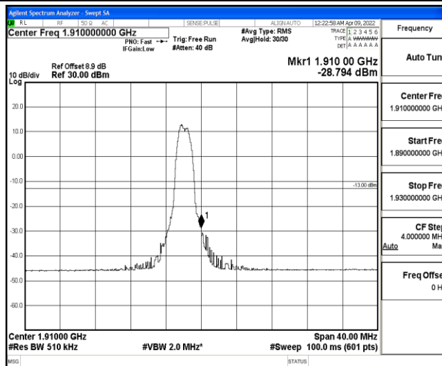
Band2-20MHz-16QAM-19100-6-0-High--28.79-PASS
