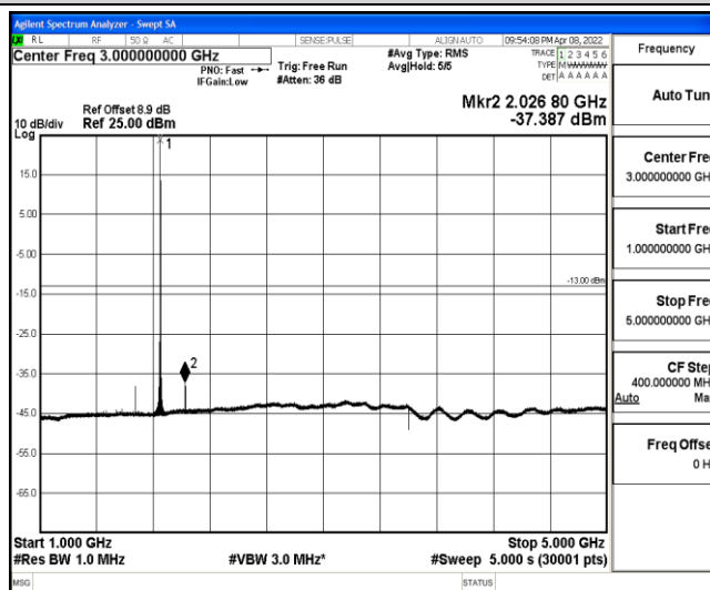
Band2-3MHz-QPSK-18615-1-0-Low-1000-5000--37.39-PASS
