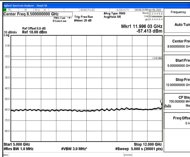
Band2-3MHz-QPSK-18900-1-0-Low-5000-12000--57.41-PASS
