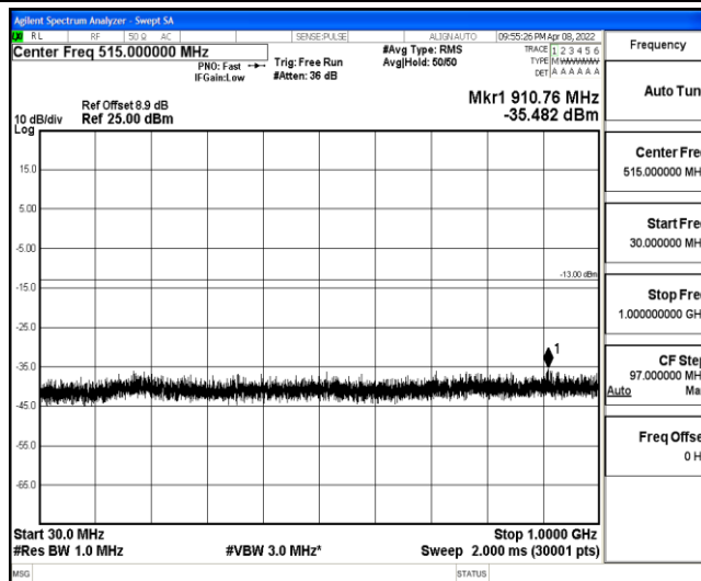
Band2-3MHz-16QAM-18615-1-0-Low-30-1000--35.48-PASS
