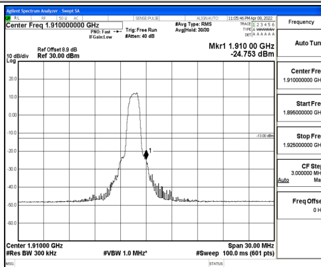
Band2-15MHz-QPSK-19125-6-0-High--24.75-PASS
