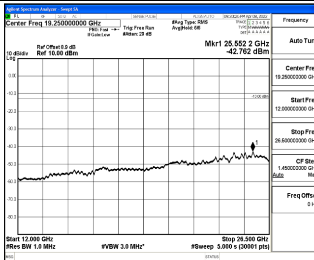
Band2-1.4MHz-QPSK-18607-1-0-Low-12000-26500--42.76-PASS
