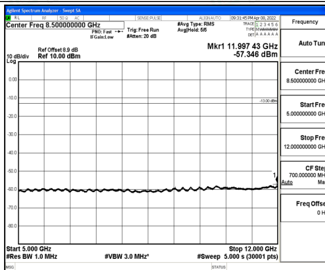
Band2-1.4MHz-16QAM-18607-1-0-Low-5000-12000--57.35-PASS
