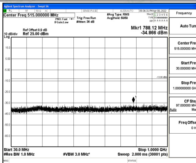
Band2-1.4MHz-QPSK-19193-1-0-High-30-1000--34.87-PASS
