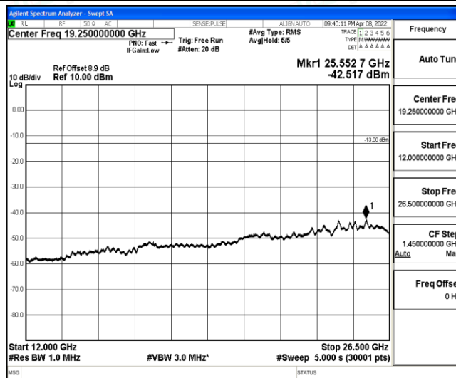
Band2-1.4MHz-16QAM-19193-1-0-High-12000-26500--42.52-PASS
