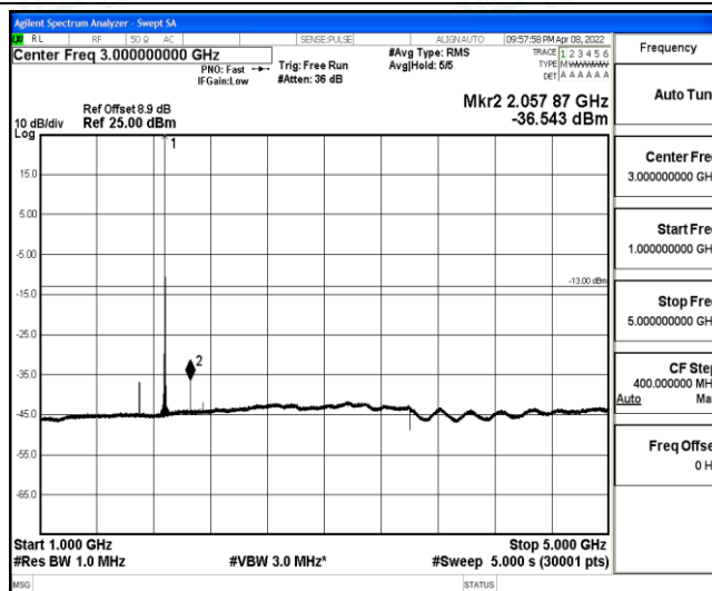
Band2-3MHz-QPSK-18900-1-0-Low-1000-5000--36.54-PASS
