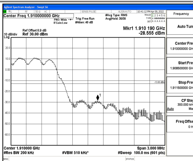
Band2-10MHz-QPSK-19150-6-0-High--28.56-PASS
