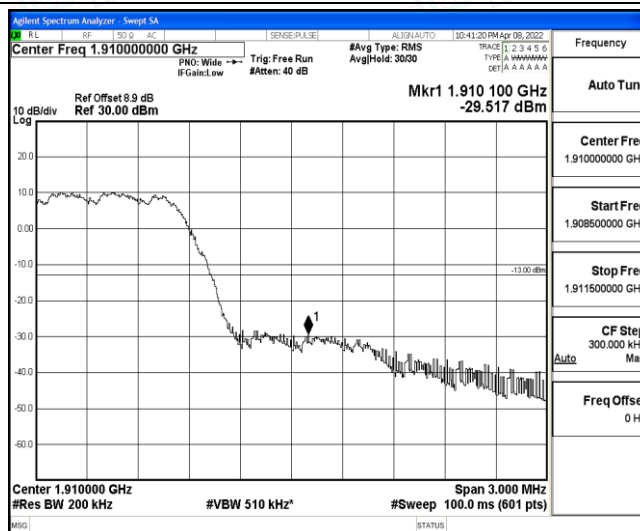
Band2-10MHz-16QAM-19150-6-0-High--29.52-PASS
