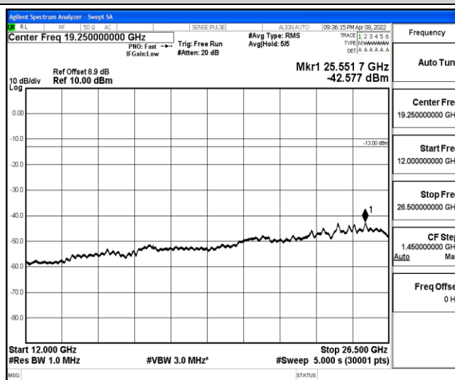
Band2-1.4MHz-16QAM-18900-1-0-Low-12000-26500--42.58-PASS
