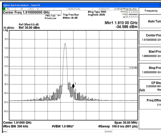
Band2-15MHz-QPSK-19125-1-0-High--34.59-PASS
