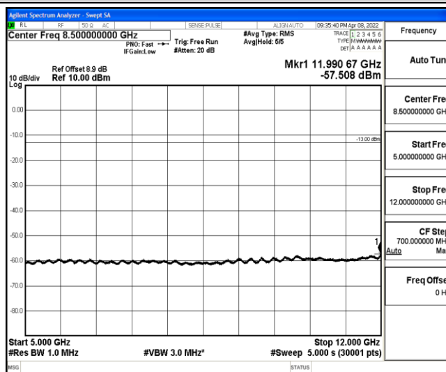
Band2-1.4MHz-16QAM-18900-1-0-Low-5000-12000--57.51-PASS
