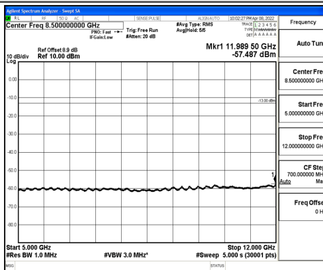
Band2-3MHz-QPSK-19185-1-0-High-5000-12000--57.49-PASS
