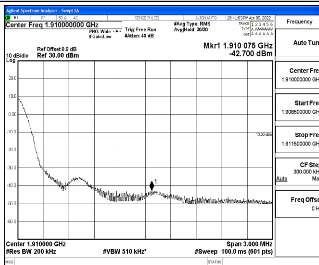
Band2-10MHz-16QAM-19150-1-0-High--42.70-PASS
