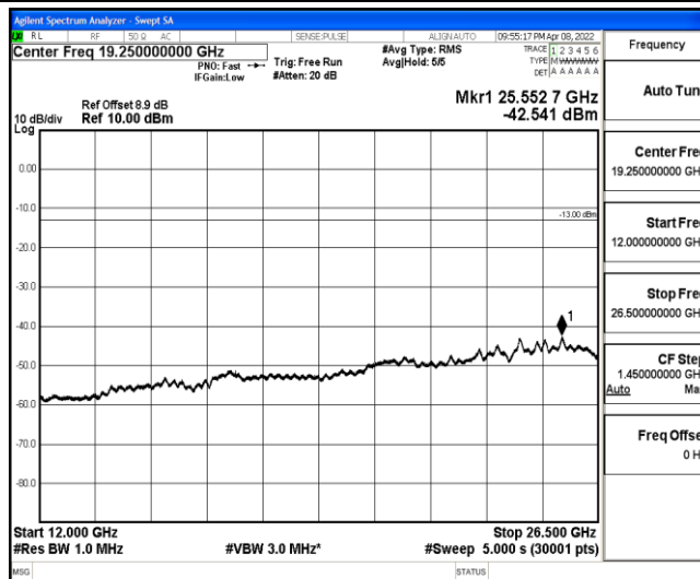
Band2-3MHz-QPSK-18615-1-0-Low-12000-26500--42.54-PASS
