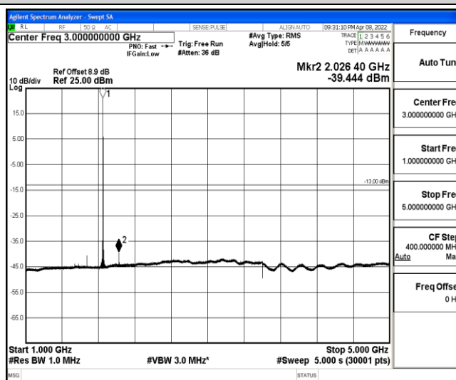
Band2-1.4MHz-16QAM-18607-1-0-Low-1000-5000--39.44-PASS
