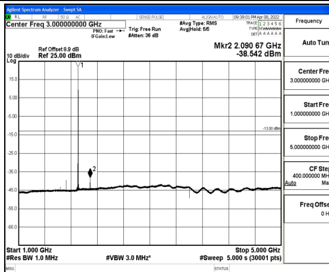
Band2-1.4MHz-16QAM-19193-1-0-High-1000-5000--38.54-PASS
