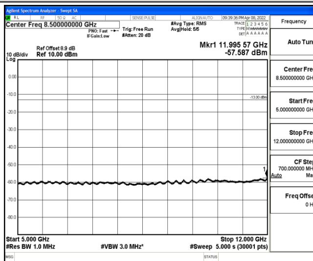
Band2-1.4MHz-16QAM-19193-1-0-High-5000-12000--57.59-PASS
