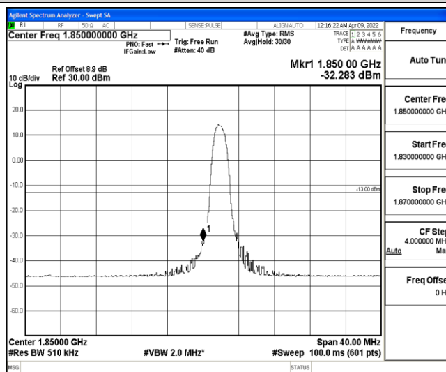
Band2-20MHz-QPSK-18700-6-0-Low--32.28-PASS
