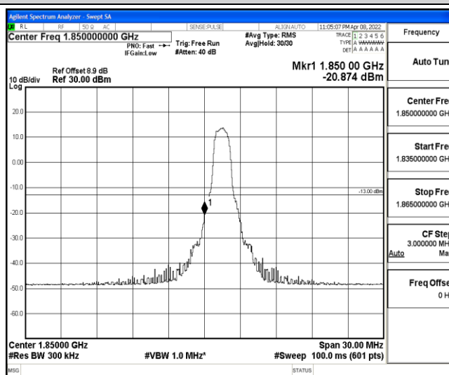
Band2-15MHz-QPSK-18675-6-0-Low--20.87-PASS
