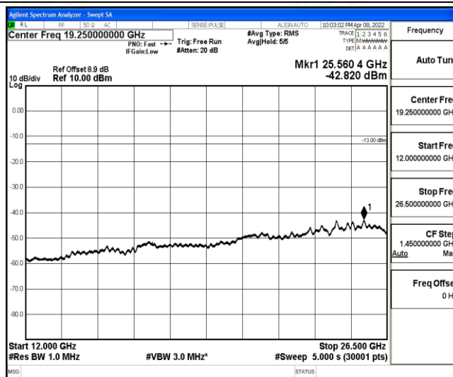
Band2-3MHz-QPSK-19185-1-0-High-12000-26500--42.82-PASS
