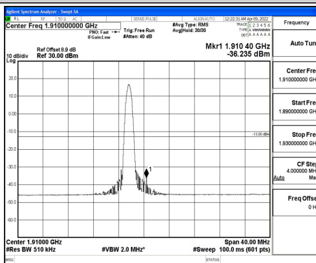
Band2-20MHz-QPSK-19100-1-0-High--36.24-PASS
