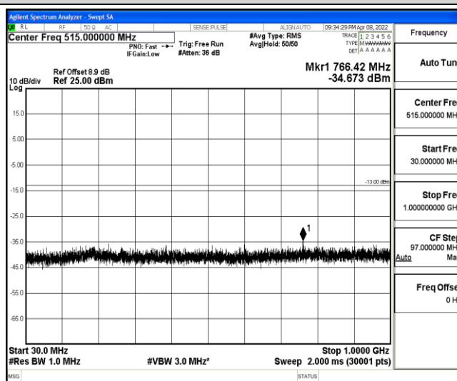
Band2-1.4MHz-16QAM-18900-1-0-Low-30-1000--34.67-PASS
