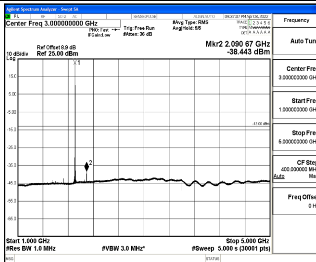
Band2-1.4MHz-QPSK-19193-1-0-High-1000-5000--38.44-PASS
