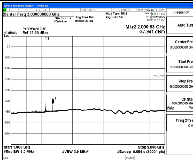
Band2-3MHz-QPSK-19185-1-0-High-1000-5000--37.94-PASS
