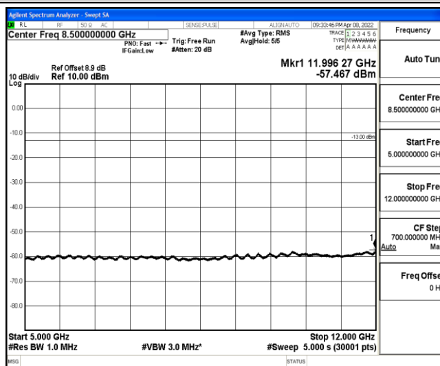
Band2-1.4MHz-QPSK-18900-1-0-Low-5000-12000--57.47-PASS
