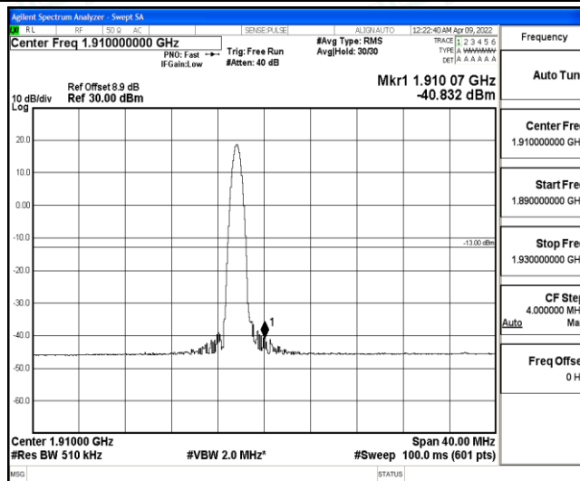
Band2-20MHz-16QAM-19100-1-0-High--40.83-PASS
