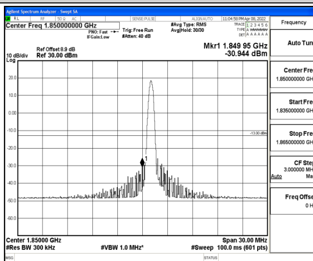
Band2-15MHz-16QAM-18675-1-0-Low--30.94-PASS
