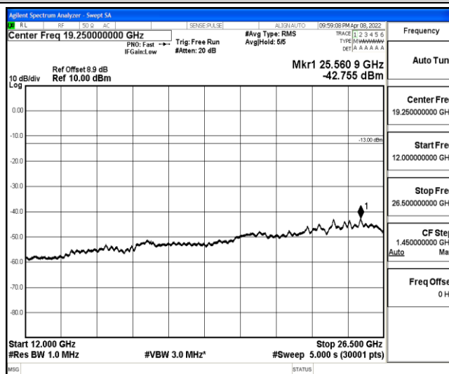
Band2-3MHz-QPSK-18900-1-0-Low-12000-26500--42.76-PASS
