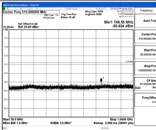
Band2-1.4MHz-16QAM-19193-1-0-High-30-1000--35.62-PASS
