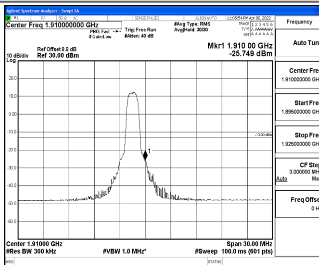
Band2-15MHz-16QAM-19125-6-0-High--25.75-PASS
