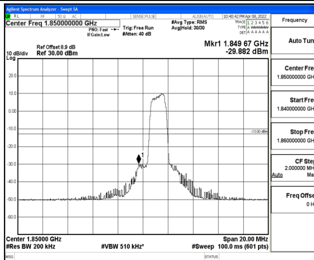
Band2-10MHz-16QAM-18650-6-0-Low--29.88-PASS
