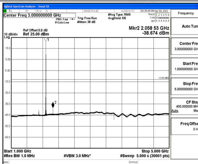
Band2-1.4MHz-16QAM-18900-1-0-Low-1000-5000--38.67-PASS
