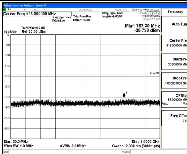
Band2-3MHz-QPSK-18615-1-0-Low-30-1000--35.73-PASS
