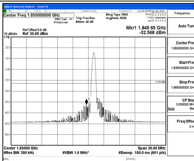
Band2-15MHz-QPSK-18675-1-0-Low--32.57-PASS
