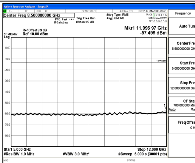
Band2-1.4MHz-QPSK-19193-1-0-High-5000-12000--57.5-PASS
