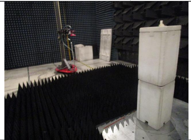
Above 1 GHz Radiated Setup
