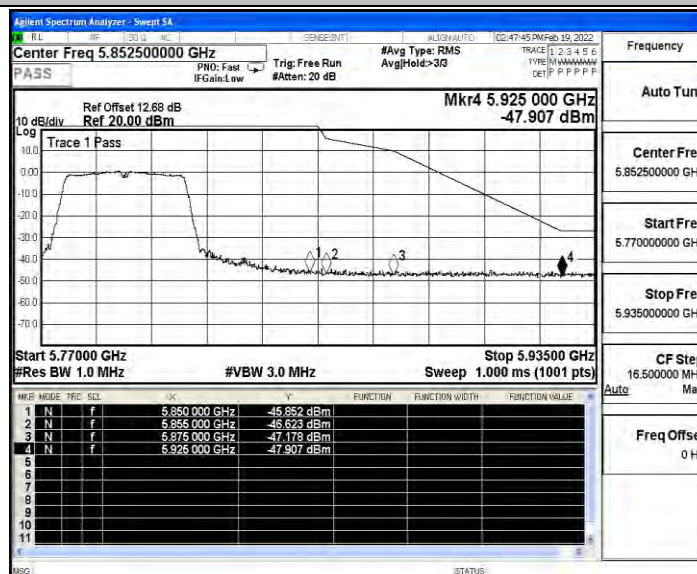
11AC40SISO_Ant7_High_5795_Peak
