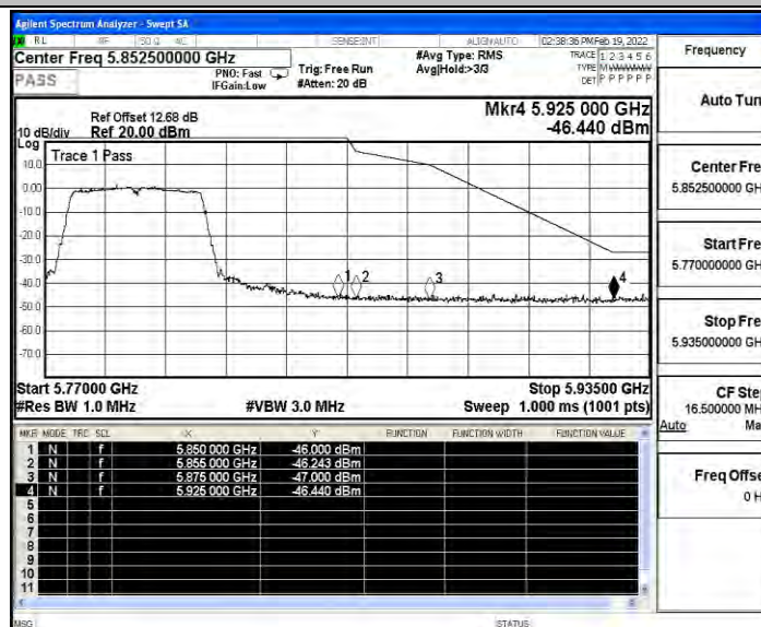
11AC40SISO_Ant5_High_5795_Peak
