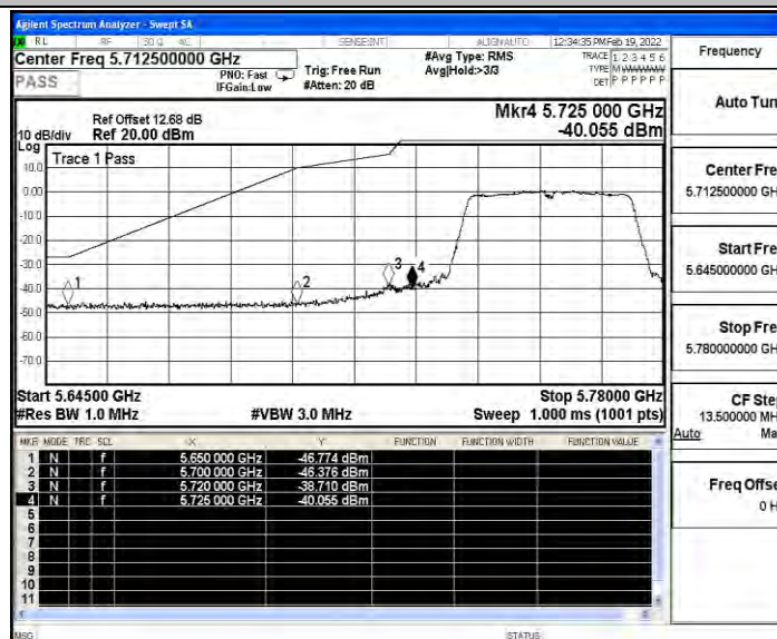
11N40SISO_Ant7_Low_5755_Peak
