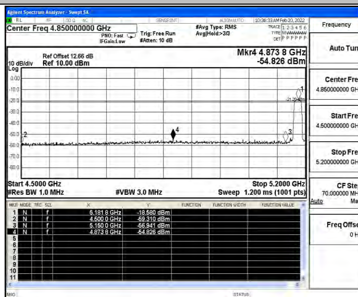
11AC20SISO_Ant6_High_5240_AV
