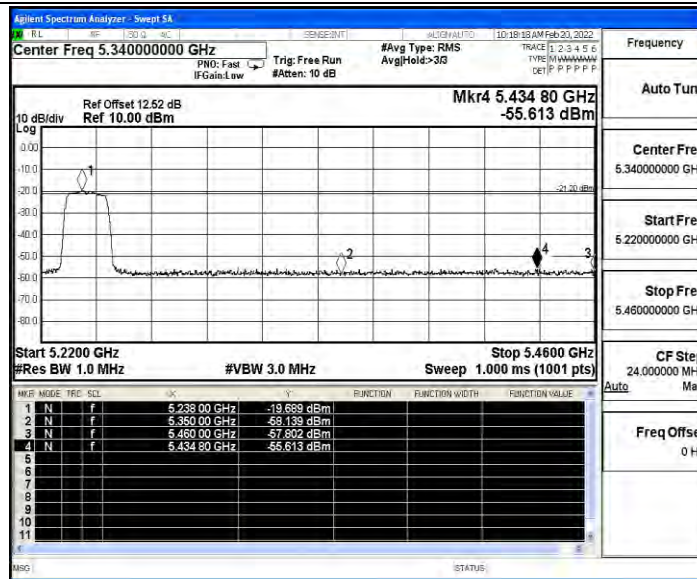
11N40SISO_Ant7_Low_5190_AV
