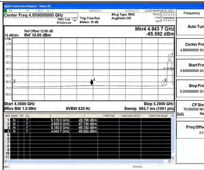
11AC20SISO_Ant6_Low_5180_Peak
