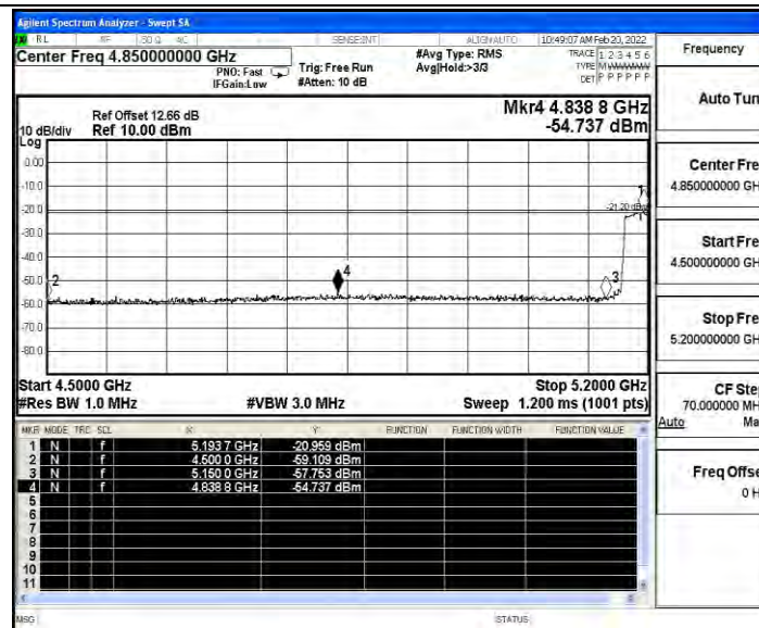
11AC40SISO_Ant6_High_5230_AV
