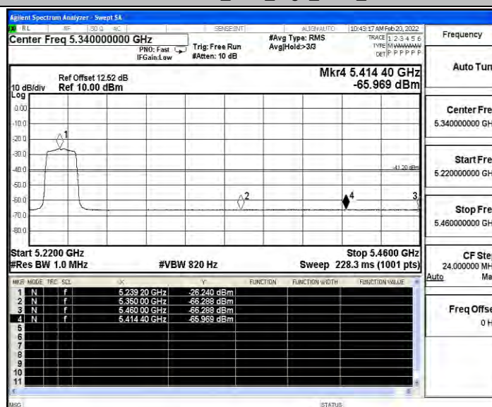
11AC20SISO_Ant6_High_5240_AV
