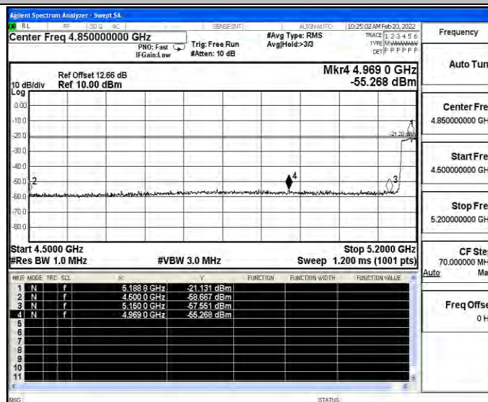
11N40SISO_Ant7_Low_5190_Peak
