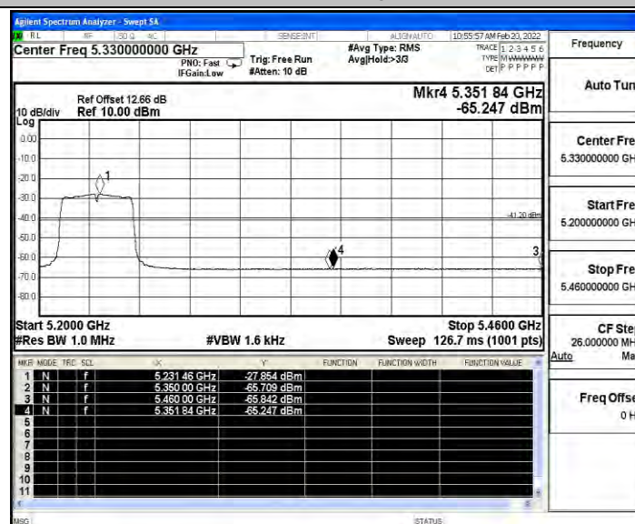
11AC40SISO_Ant6_High_5230_Peak
