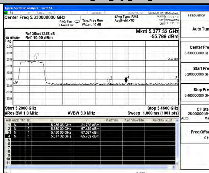
11AC40SISO_Ant4_High_5230_Peak
