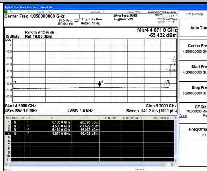
11N40SISO_Ant4_Low_5190_Peak
