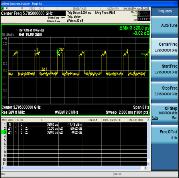
NTNV-11AC40MIMO-Ant2-5795
