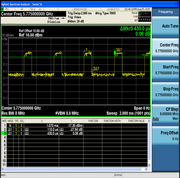
NTNV-11AX80MIMO-Ant2-5775
