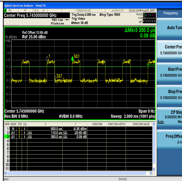
NTNV-11AX20MIMO-Ant2-5745
