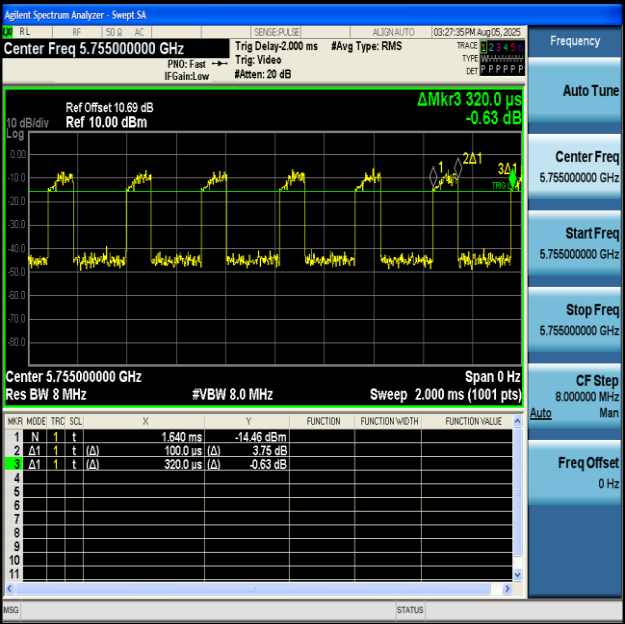
NTNV-11N40MIMO-Ant2-5755
