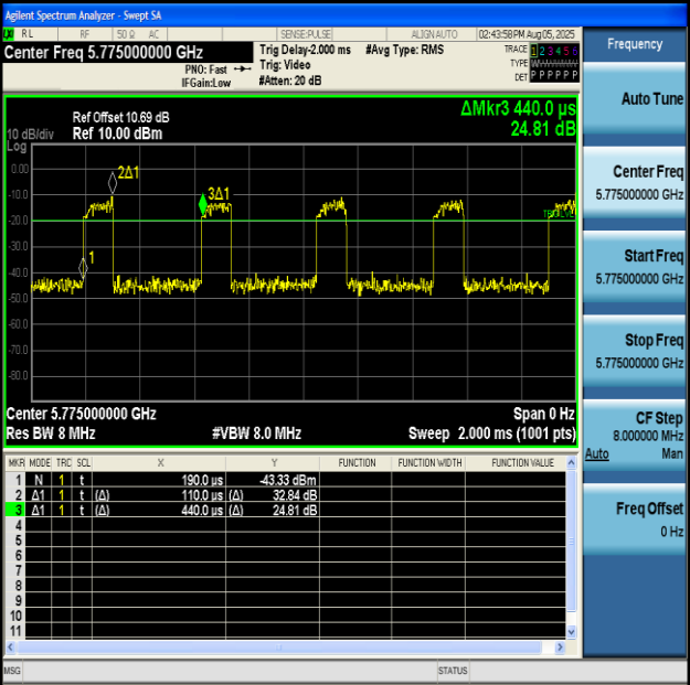
NTNV-11AX80MIMO-Ant1-5775
