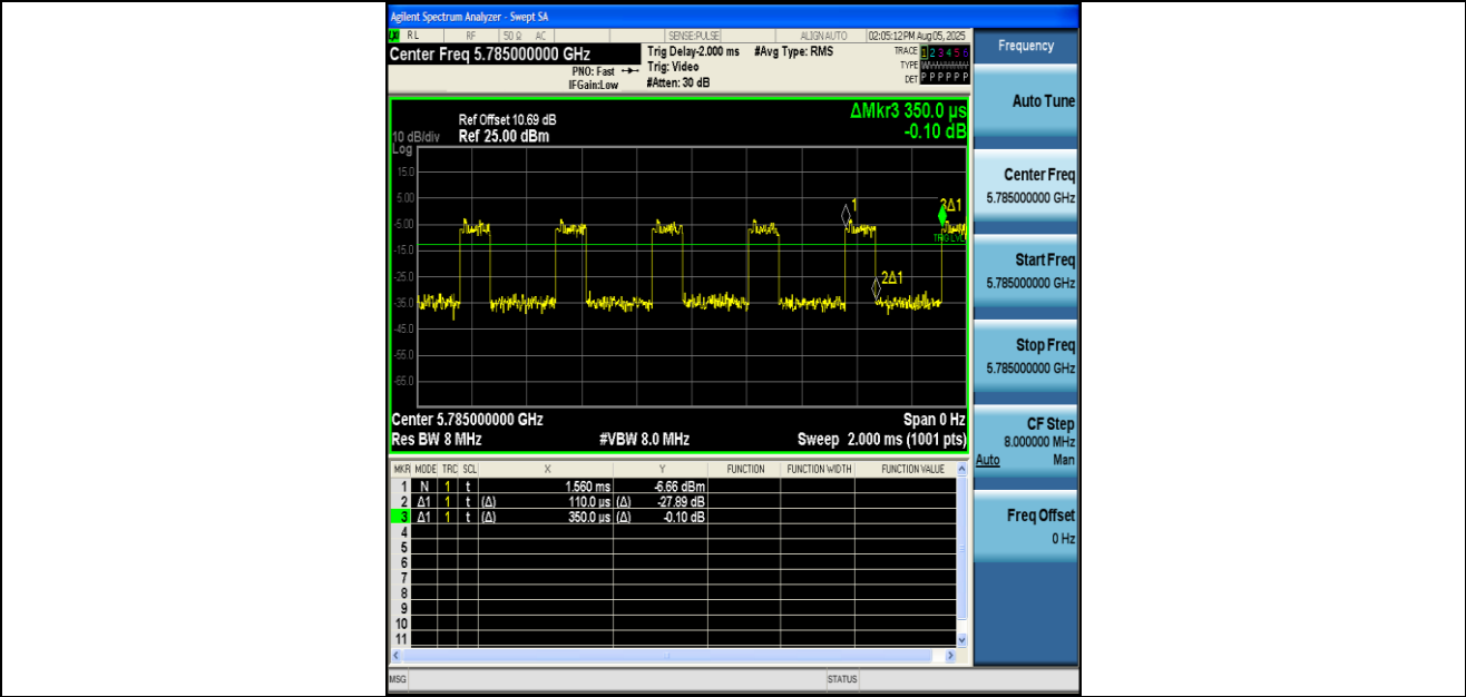
NTNV-11AX20MIMO-Ant2-5785
