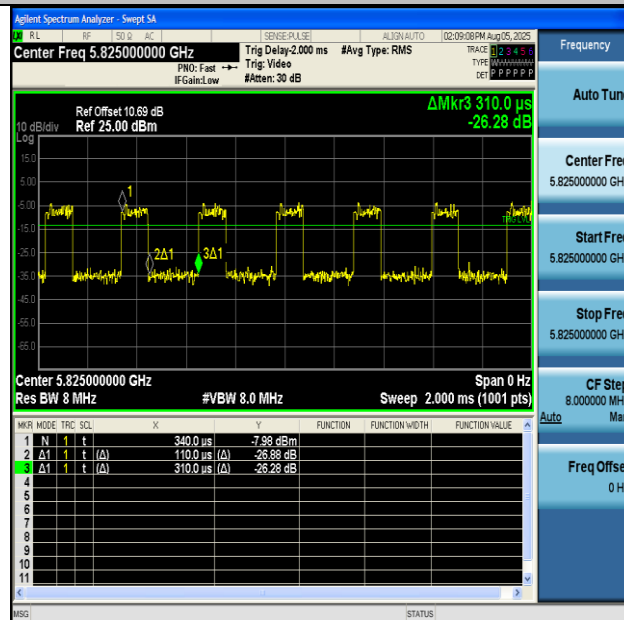
NTNV-11AX20MIMO-Ant2-5825
