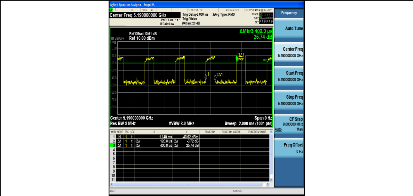
NTNV-11AX40MIMO-Ant2-5190
