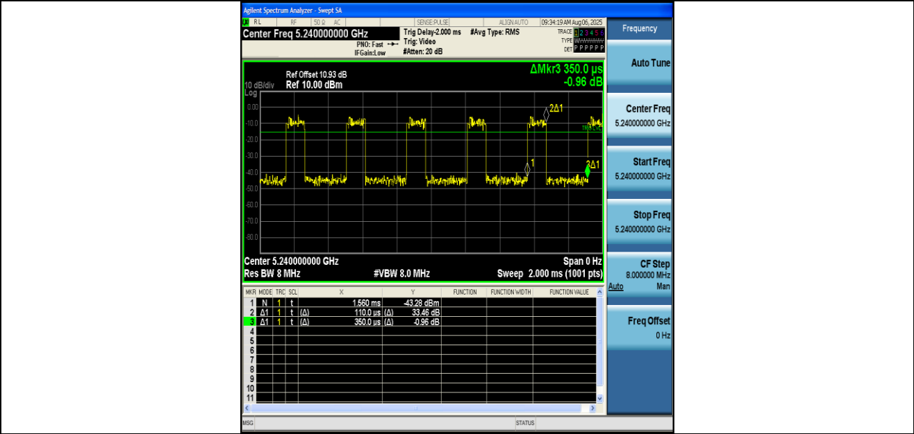
NTNV-11AX20MIMO-Ant2-5240
