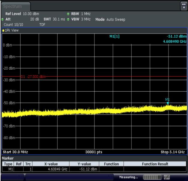
11AC80MIMO-Ant1-5210-30~5140-PASS
