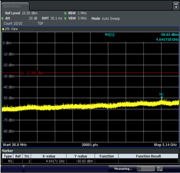
11AC40MIMO-Ant1-5230-30~5140-PASS
