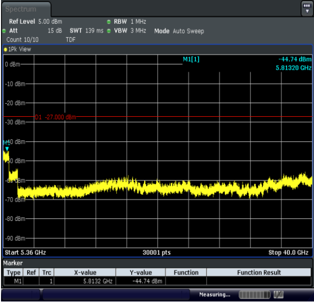
11AX40MIMO-Ant2-5190-5360~40000-PASS
