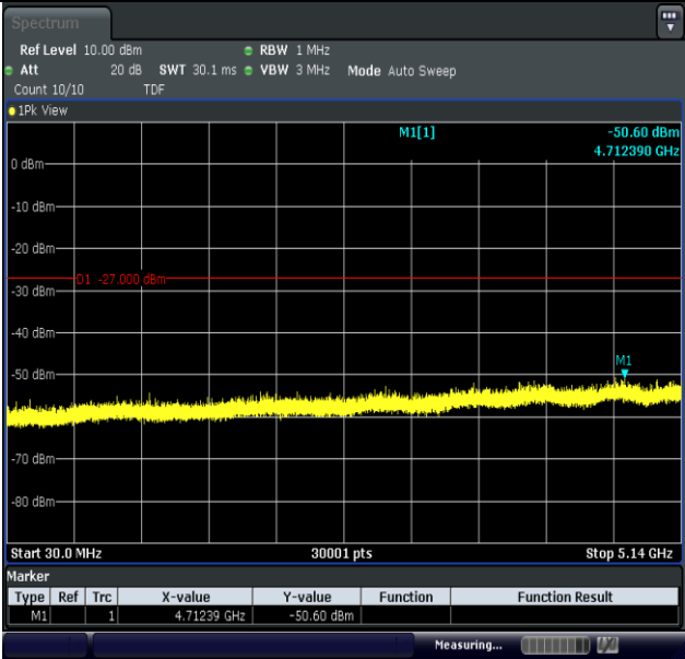
11AX80MIMO-Ant1-5210-30~5140-PASS
