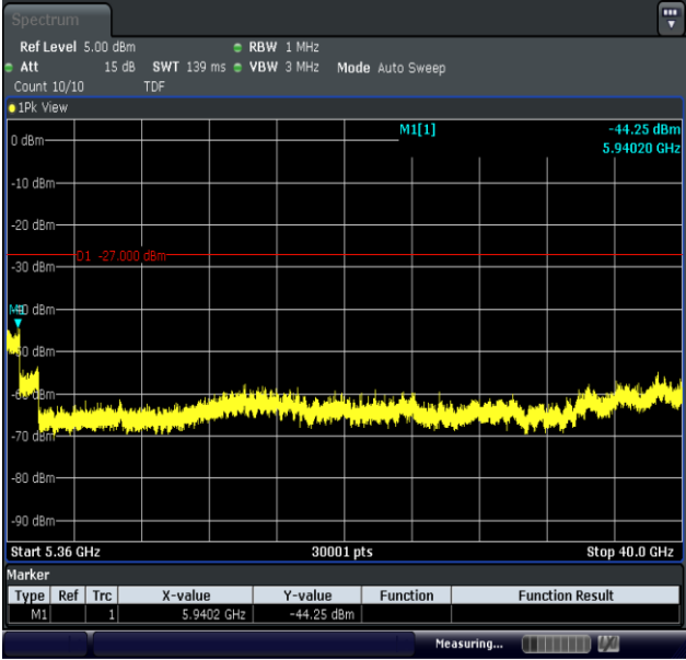
11N20MIMO-Ant2-5180-5360~40000-PASS
