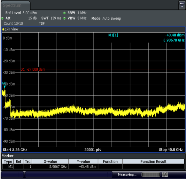
11AX20MIMO-Ant2-5180-5360~40000-PASS
