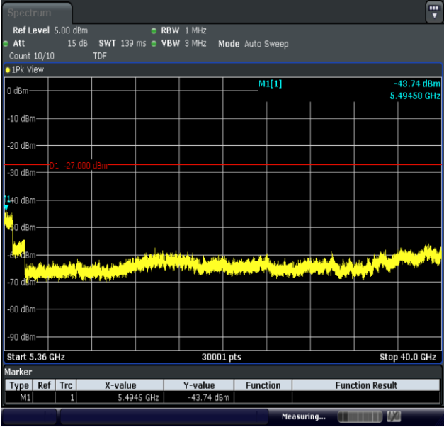
11AX40MIMO-Ant2-5230-5360~40000-PASS
