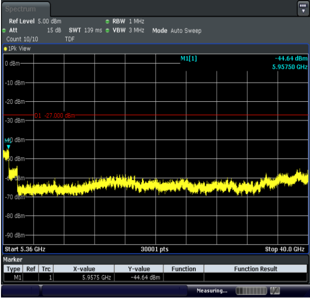
11AC20MIMO-Ant2-5180-5360~40000-PASS
