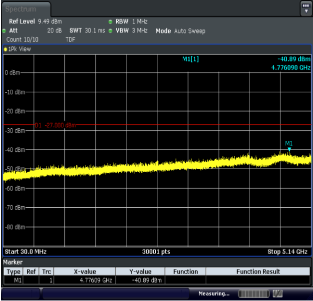
11AC20MIMO-Ant2-5200-30~5140-PASS
