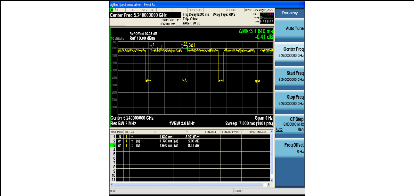
NTNV-11A-Ant2-5240
