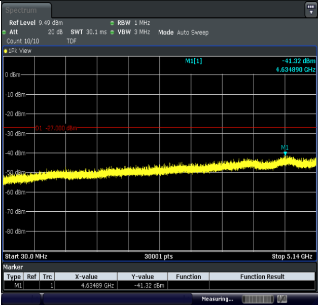
11N20MIMO-Ant2-5180-30~5140-PASS
