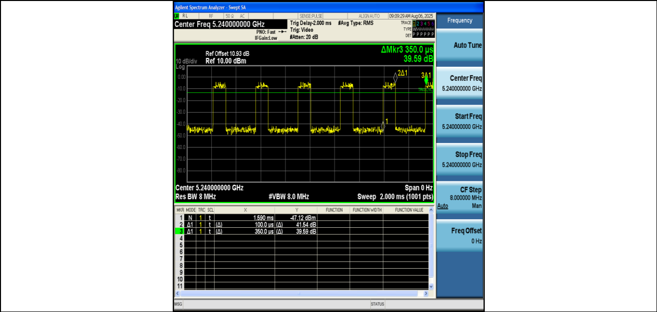
NTNV-11AC20MIMO-Ant2-5240
