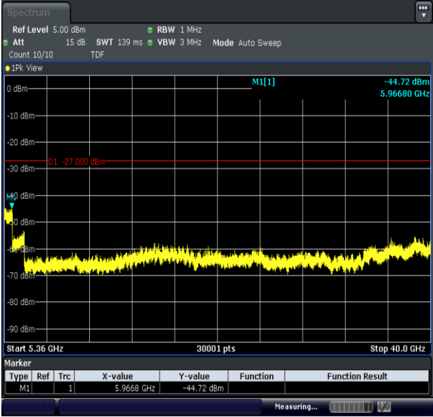
11N40MIMO-Ant2-5230-5360~40000-PASS
