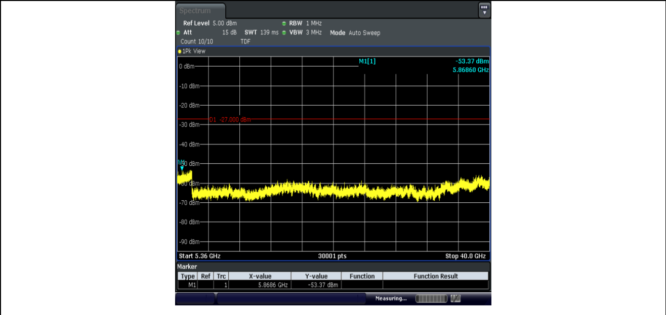
11N20MIMO-Ant1-5200-5360~40000-PASS
