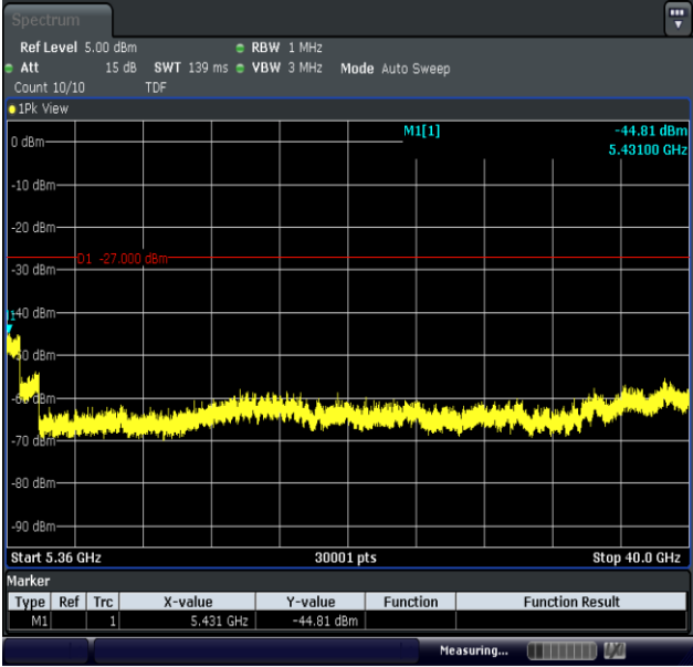
11N20MIMO-Ant2-5240-5360~40000-PASS
