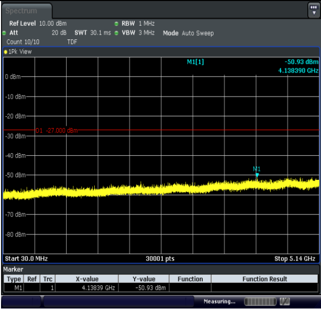
11AC20MIMO-Ant1-5240-30~5140-PASS
