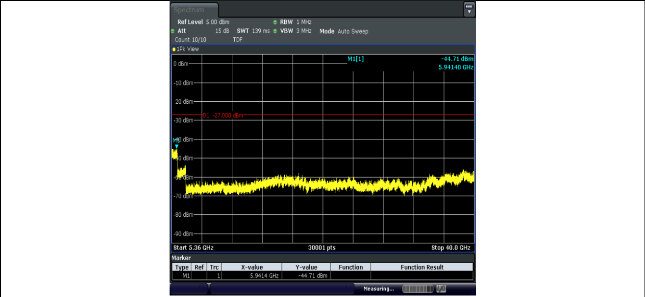
11AX80MIMO-Ant2-5210-5360~40000-PASS
