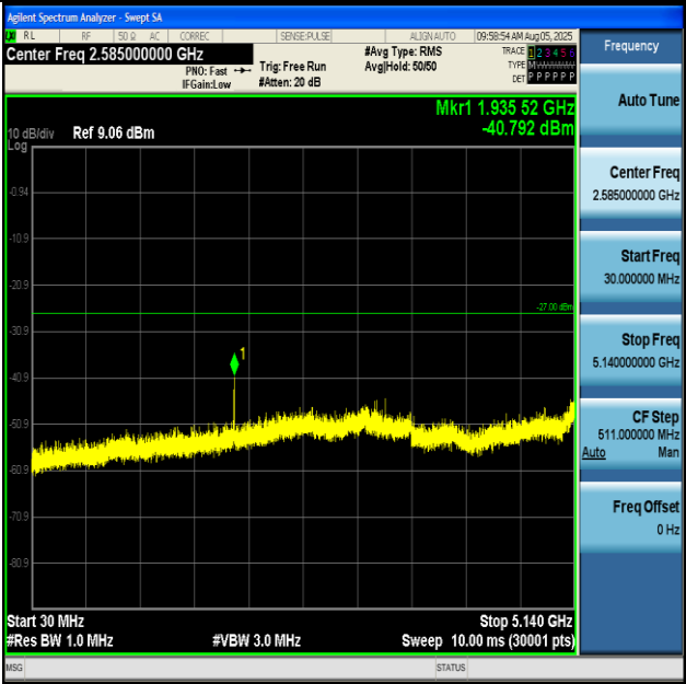
11A-Ant1-5240-30~5140-PASS
