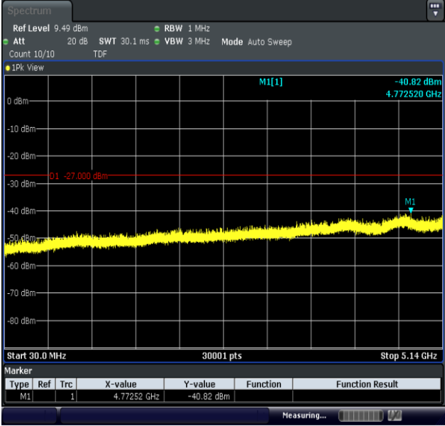
11AX20MIMO-Ant2-5180-30~5140-PASS
