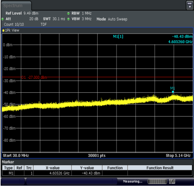
11N20MIMO-Ant2-5200-30~5140-PASS
