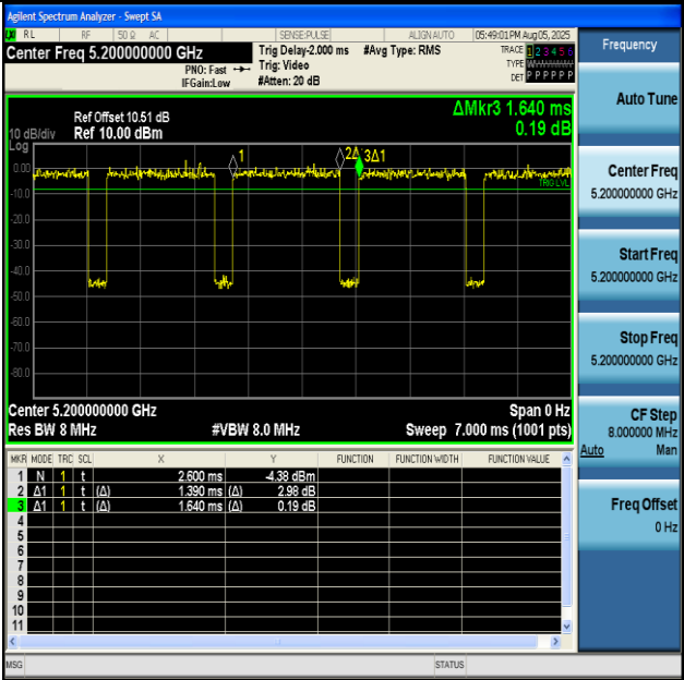
NTNV-11A-Ant2-5200
