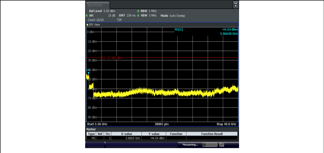
11AC40MIMO-Ant2-5190-5360~40000-PASS
