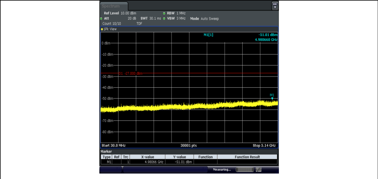
11N20MIMO-Ant1-5240-30~5140-PASS
