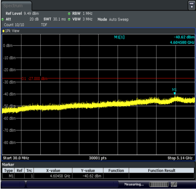
11N40MIMO-Ant2-5230-30~5140-PASS
