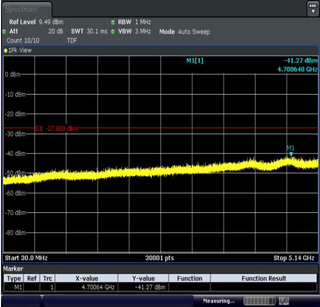
11AX80MIMO-Ant2-5210-30~5140-PASS
