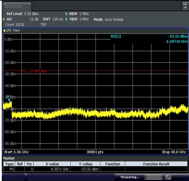
11AC40MIMO-Ant1-5230-5360~40000-PASS
