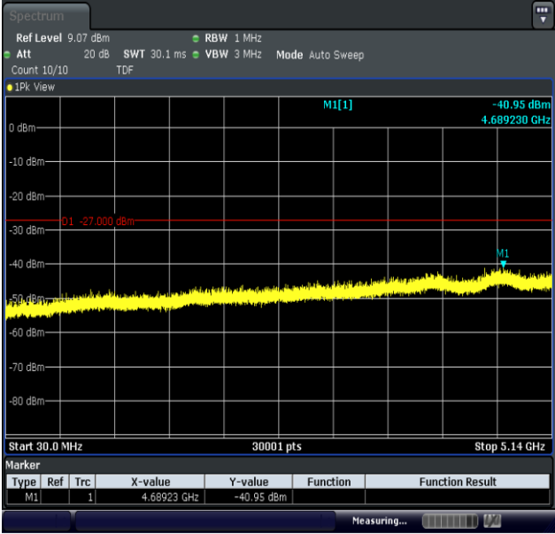
11AC20MIMO-Ant2-5240-30~5140-PASS
