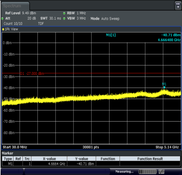
11AX40MIMO-Ant2-5230-30~5140-PASS
