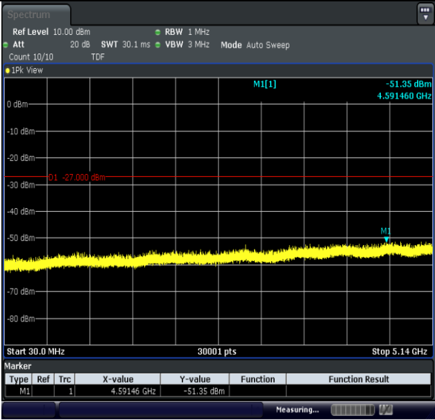
11AC20MIMO-Ant1-5180-30~5140-PASS
