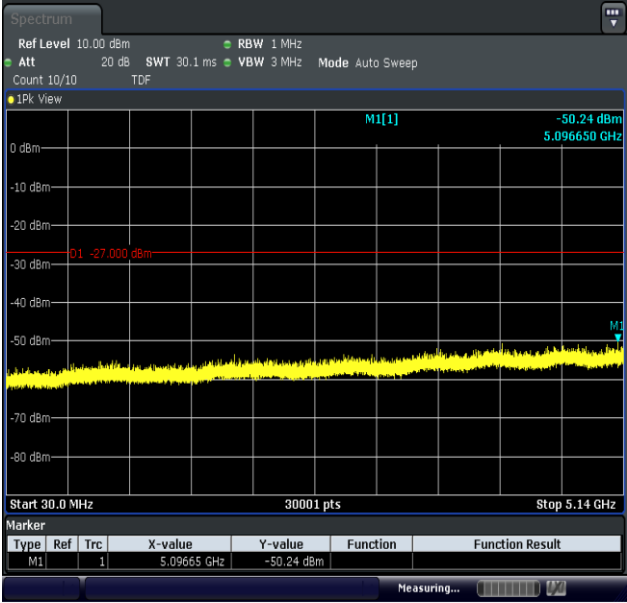
11AX20MIMO-Ant1-5180-30~5140-PASS
