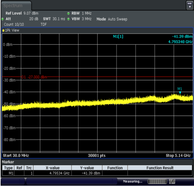
11AX20MIMO-Ant2-5240-30~5140-PASS
