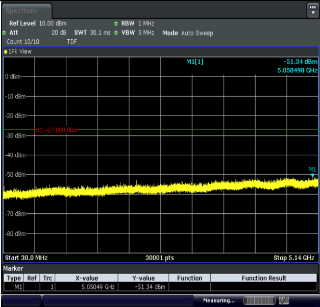
11AX40MIMO-Ant1-5190-30~5140-PASS
