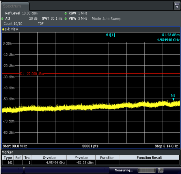
11AX40MIMO-Ant1-5230-30~5140-PASS
