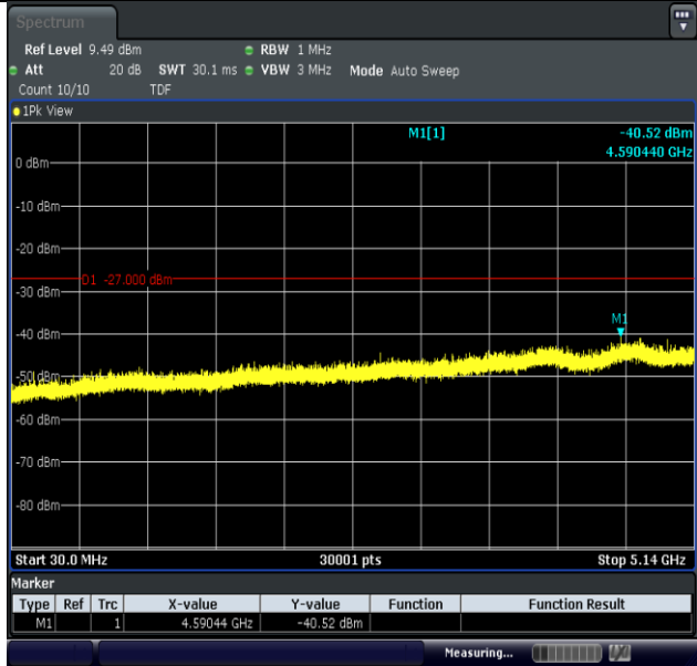
11AC40MIMO-Ant2-5190-30~5140-PASS
