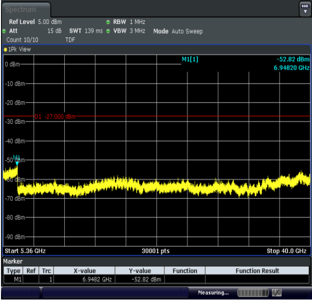
11AC20MIMO-Ant1-5200-5360~40000-PASS
