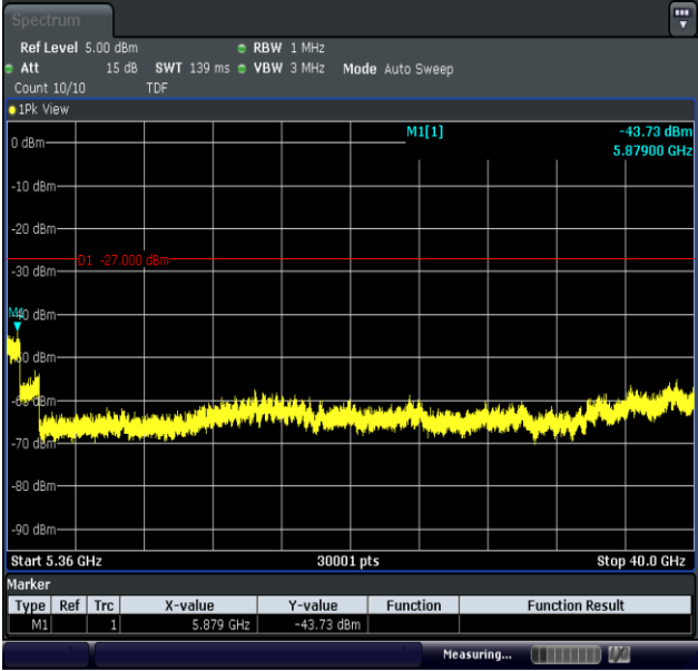
11AX20MIMO-Ant2-5240-5360~40000-PASS
