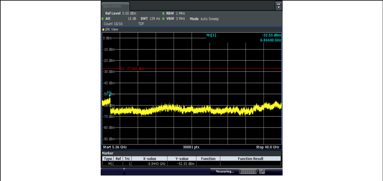
11N40MIMO-Ant1-5190-5360~40000-PASS
