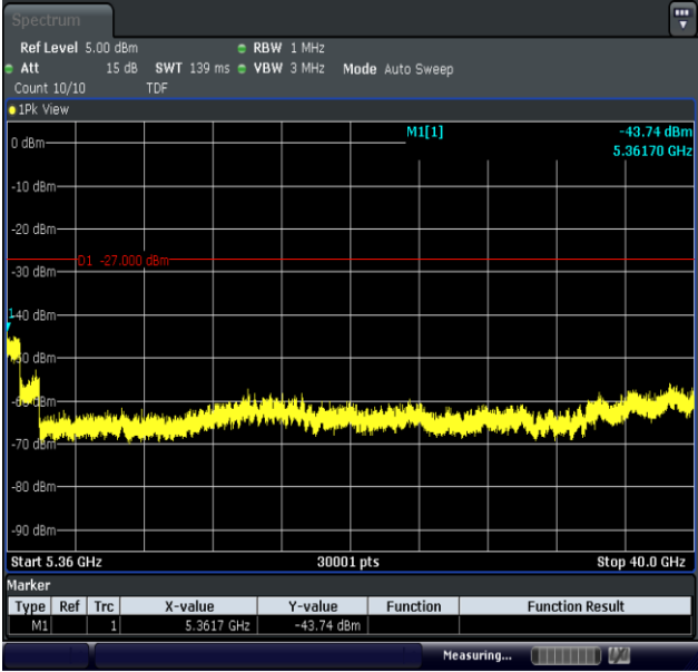
11AC20MIMO-Ant2-5240-5360~40000-PASS
