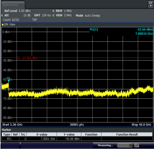
11N40MIMO-Ant1-5230-5360~40000-PASS
