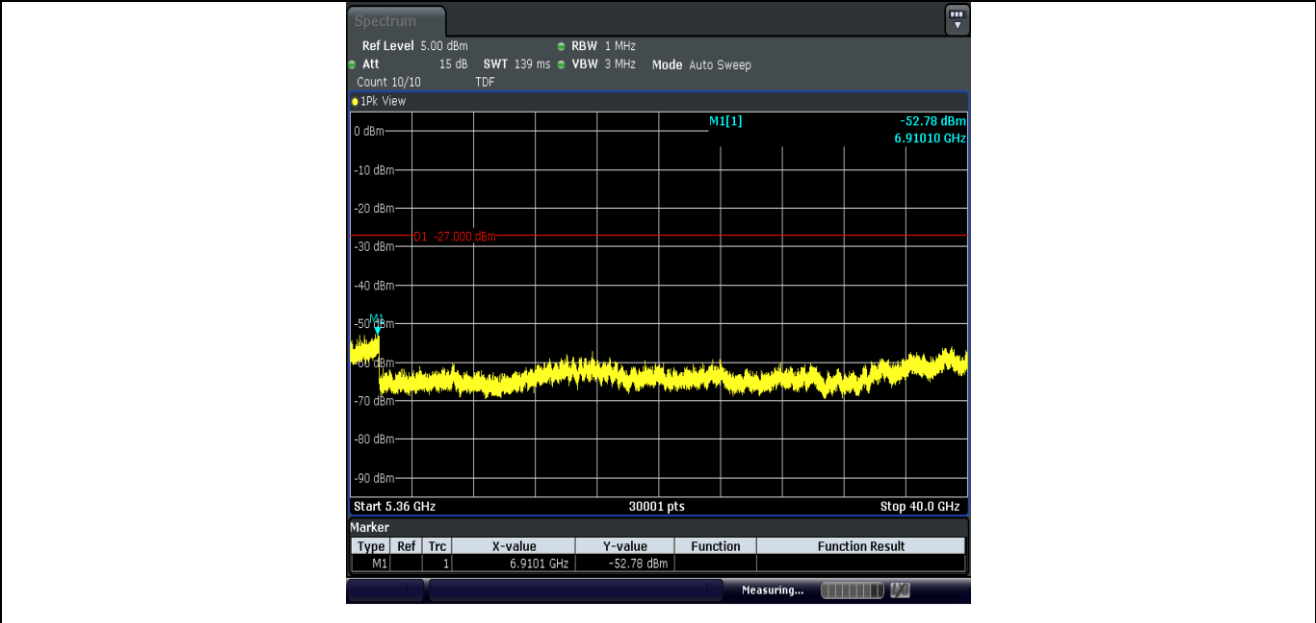
11AC40MIMO-Ant1-5190-5360~40000-PASS
