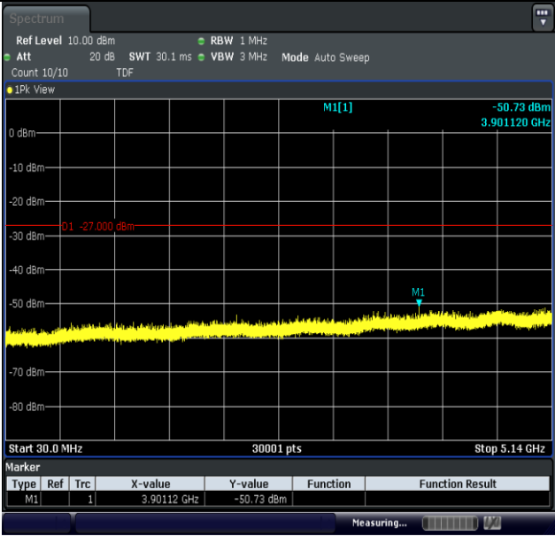
11N40MIMO-Ant1-5230-30~5140-PASS
