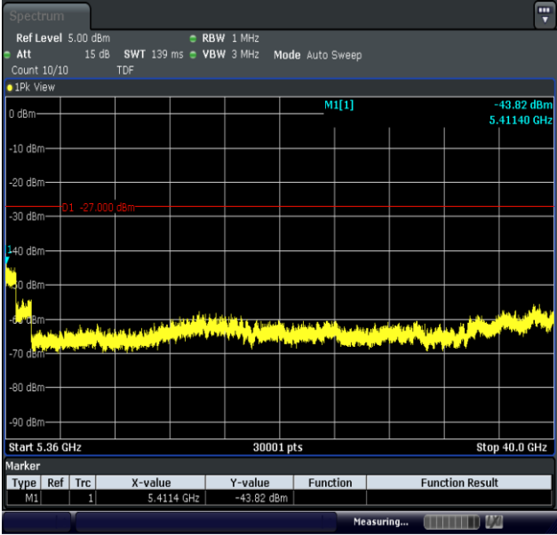
11AC20MIMO-Ant2-5200-5360~40000-PASS
