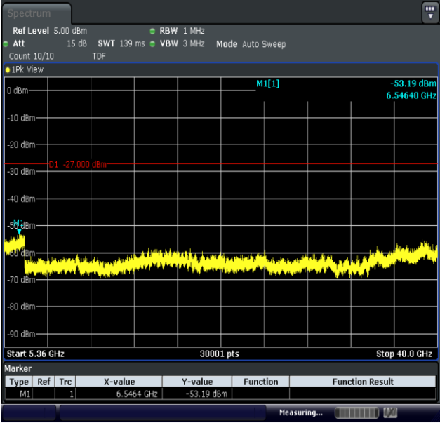
11AX20MIMO-Ant1-5200-5360~40000-PASS
