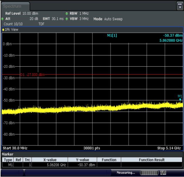
11N20MIMO-Ant1-5200-30~5140-PASS
