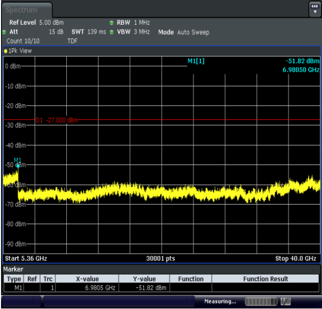
11AX40MIMO-Ant1-5190-5360~40000-PASS
