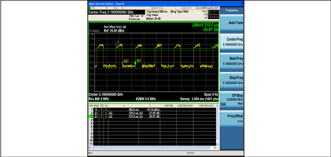
NTNV-11N40MIMO-Ant2-5190
