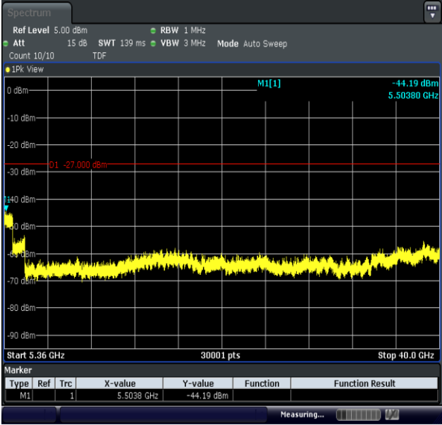
11AC80MIMO-Ant2-5210-5360~40000-PASS
