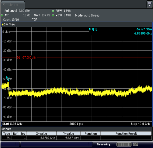
11AC20MIMO-Ant1-5240-5360~40000-PASS
