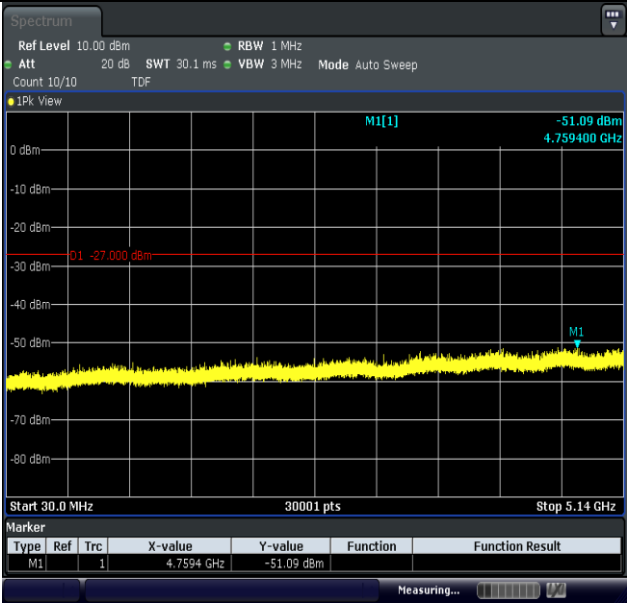
11N20MIMO-Ant1-5180-30~5140-PASS
