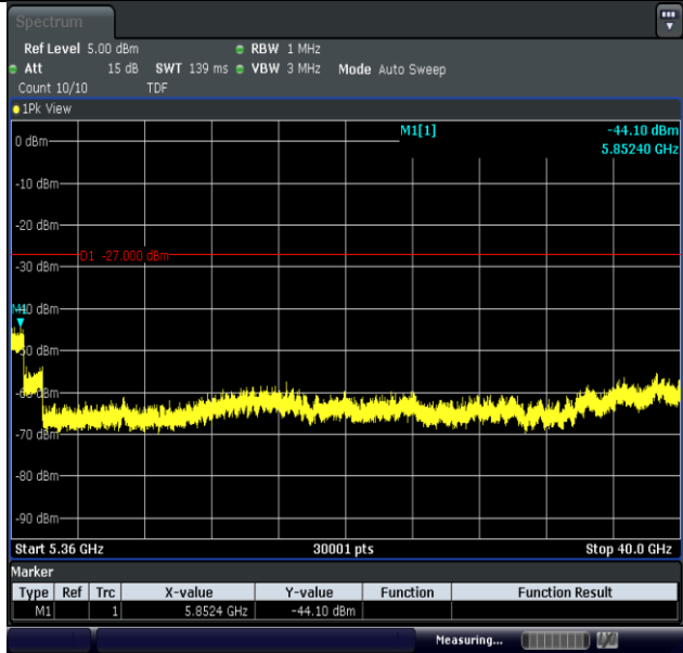
11AC40MIMO-Ant2-5230-5360~40000-PASS
