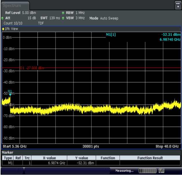
11AX20MIMO-Ant1-5240-5360~40000-PASS
