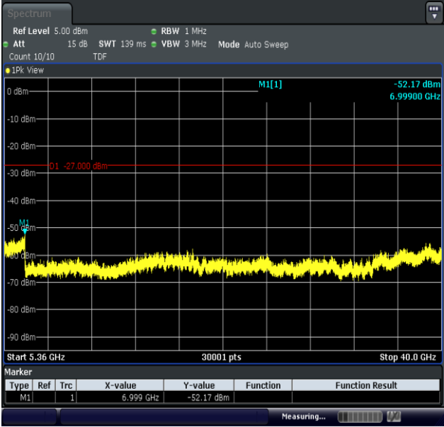
11N20MIMO-Ant1-5240-5360~40000-PASS
