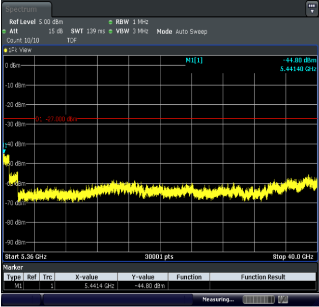
11AX20MIMO-Ant2-5200-5360~40000-PASS
