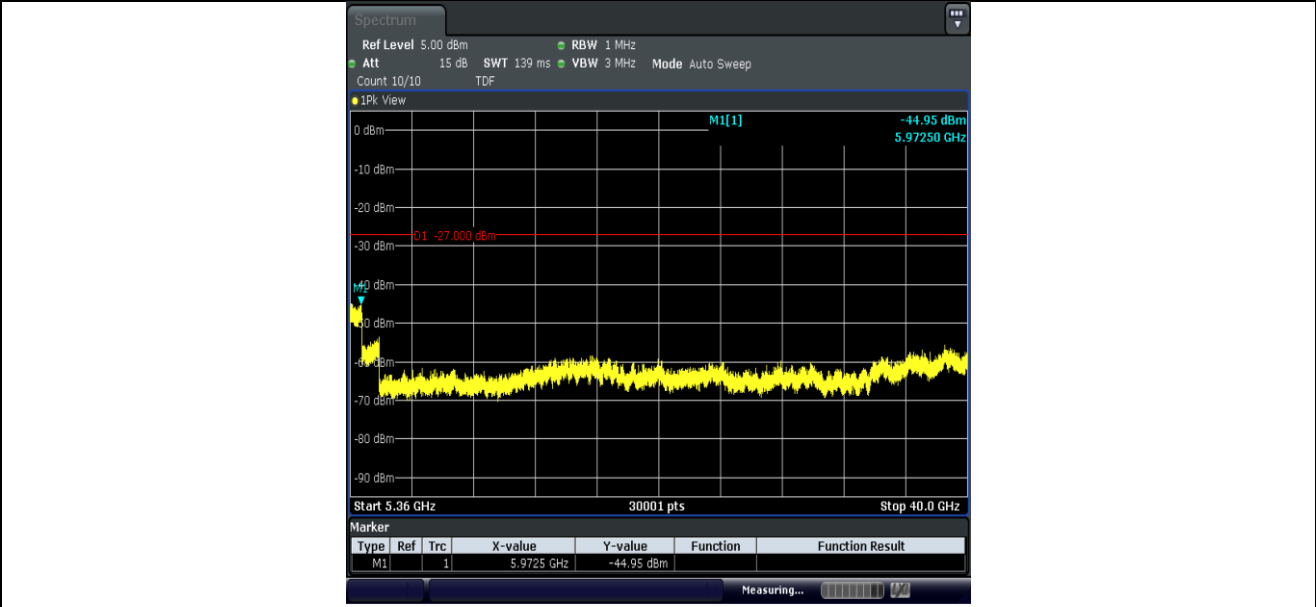
11N40MIMO-Ant2-5190-5360~40000-PASS
