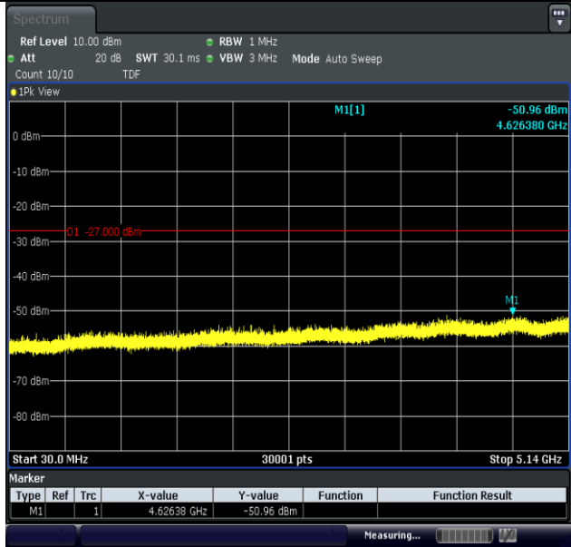
11AC40MIMO-Ant1-5190-30~5140-PASS
