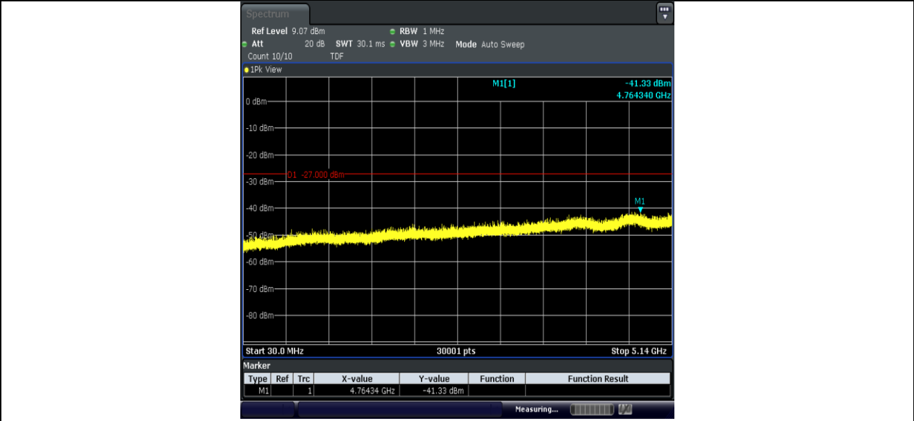
11N20MIMO-Ant2-5240-30~5140-PASS
