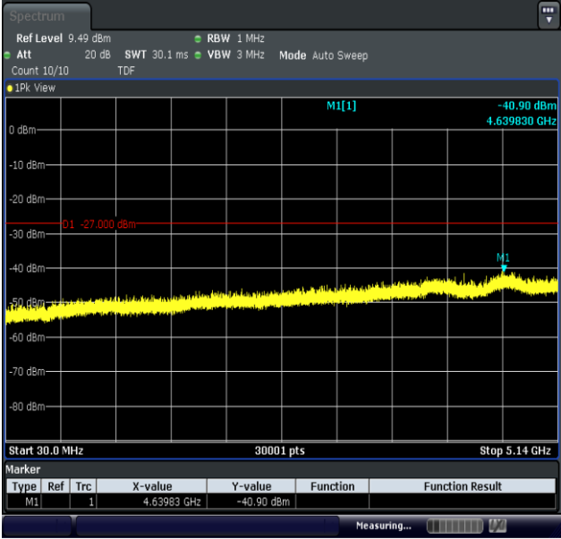
11AC40MIMO-Ant2-5230-30~5140-PASS
