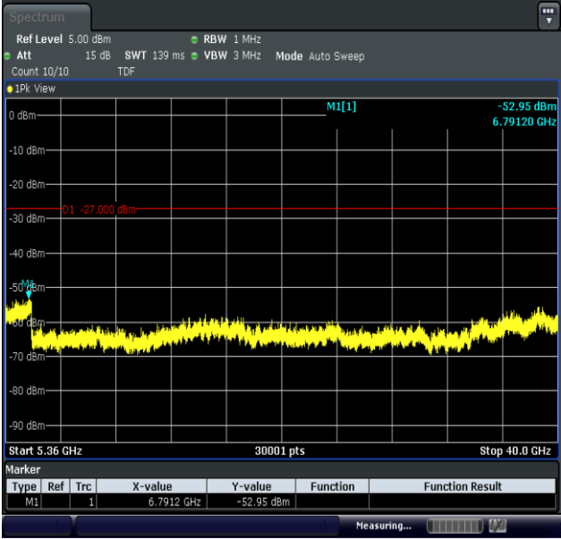
11AC80MIMO-Ant1-5210-5360~40000-PASS
