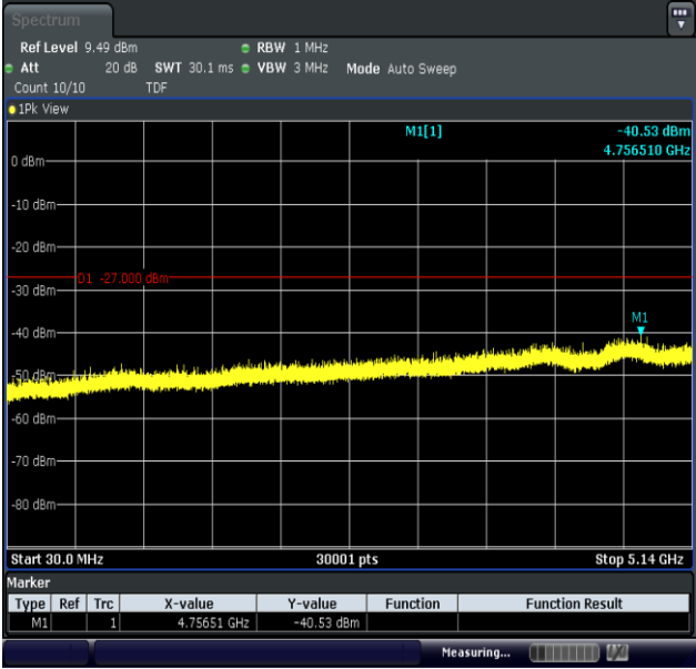
11AC20MIMO-Ant2-5180-30~5140-PASS
