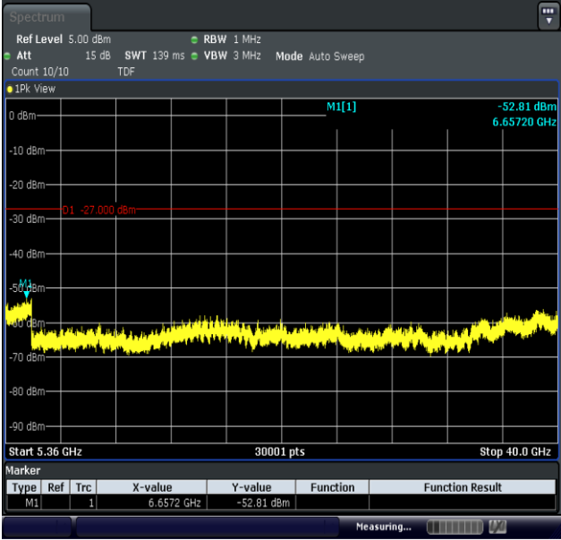
11AC20MIMO-Ant1-5180-5360~40000-PASS
