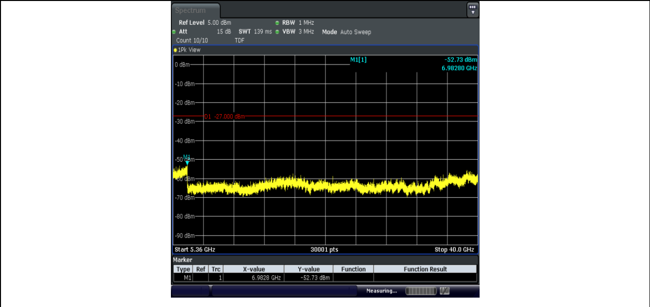
11AX80MIMO-Ant1-5210-5360~40000-PASS
