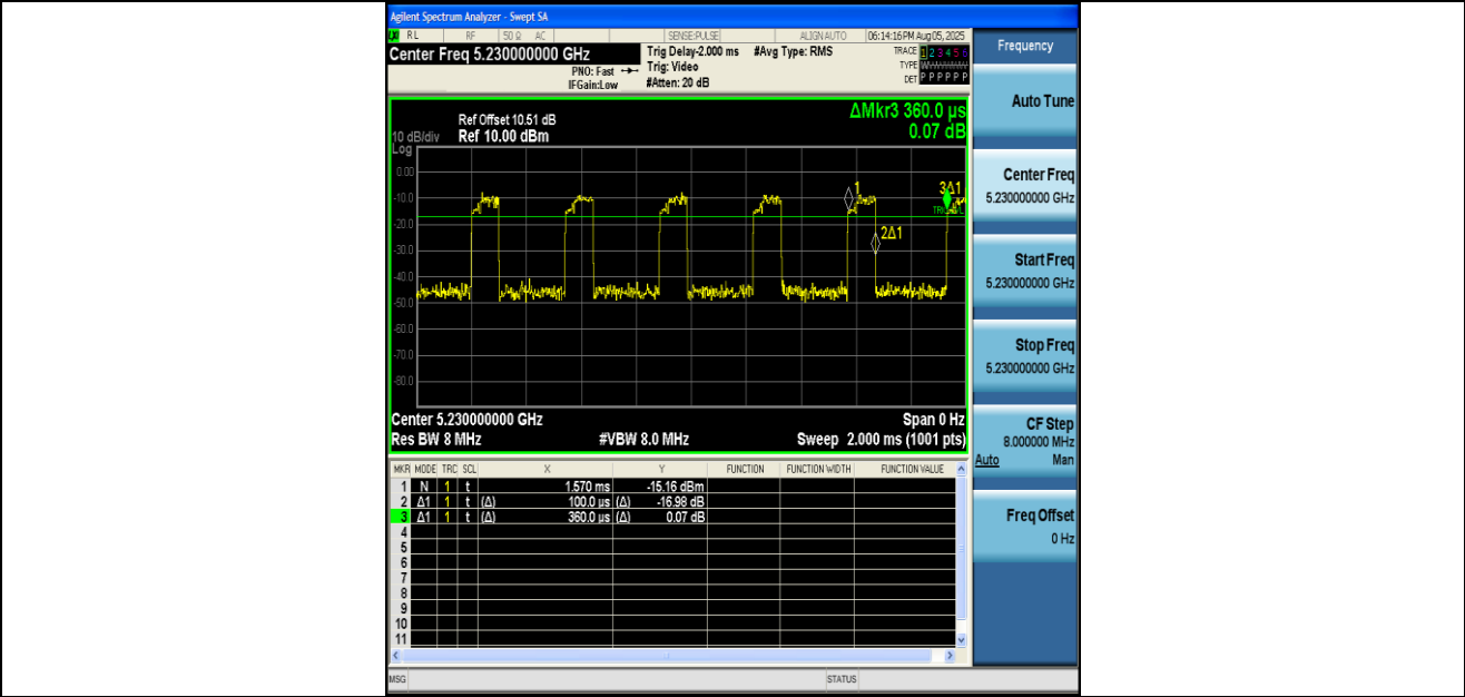
NTNV-11N40MIMO-Ant2-5230
