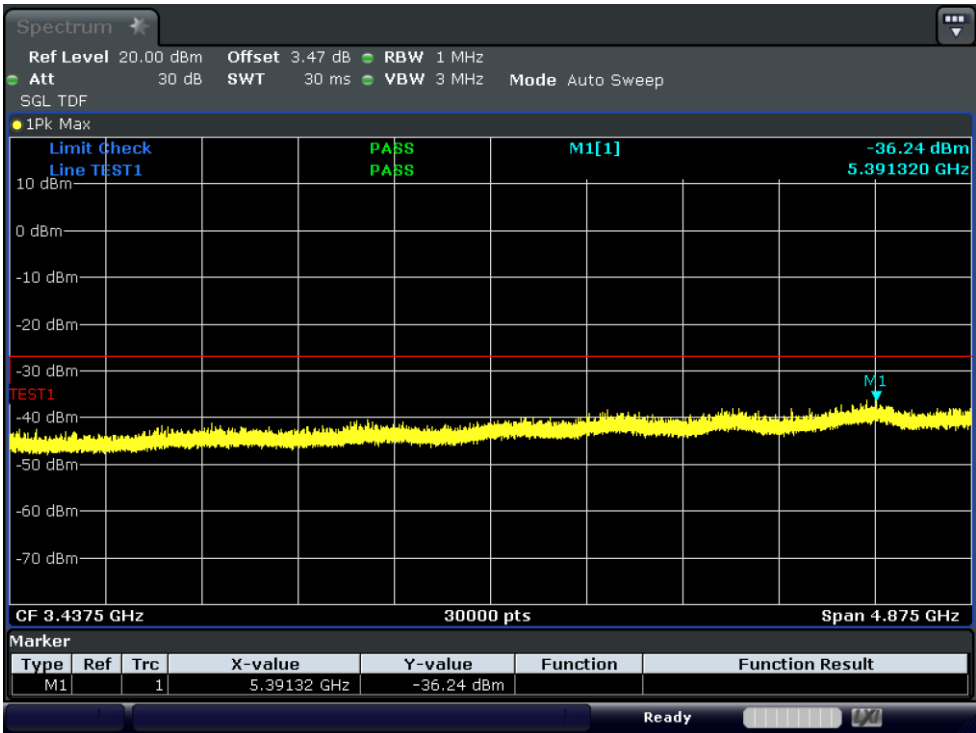
Test_Graph_11ax40_ANT1_6445_HE0_TX1
