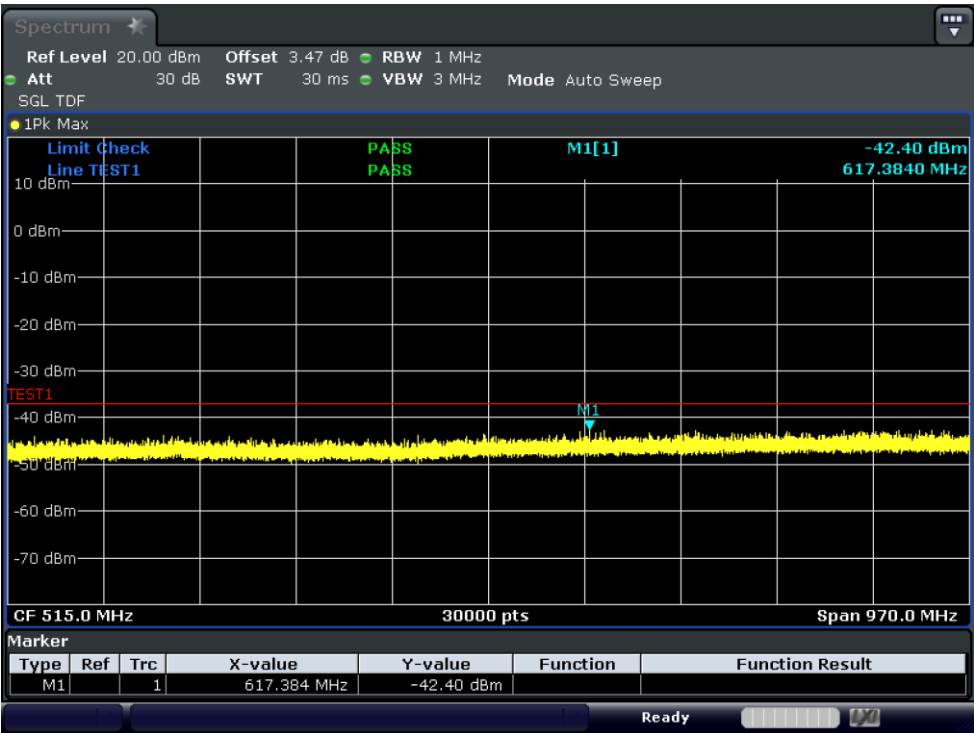
Test_Graph_11ax40_ANT1_5965_HE0_TX1
