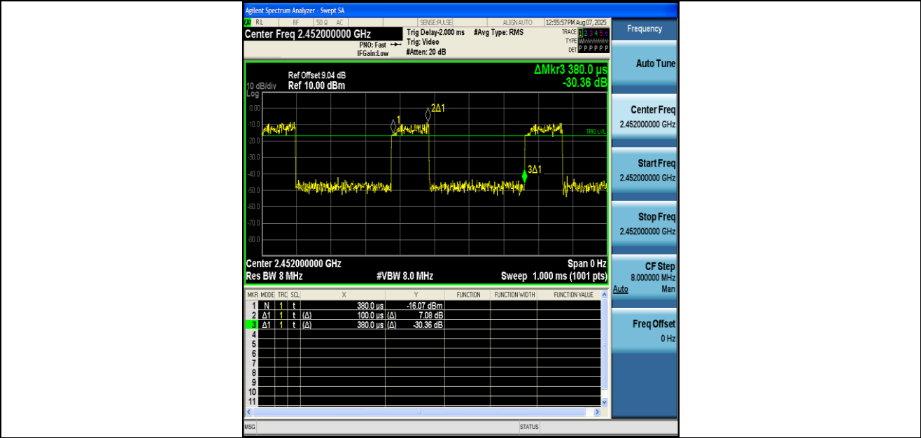
NTNV-11AX40MIMO-Ant2-2452
