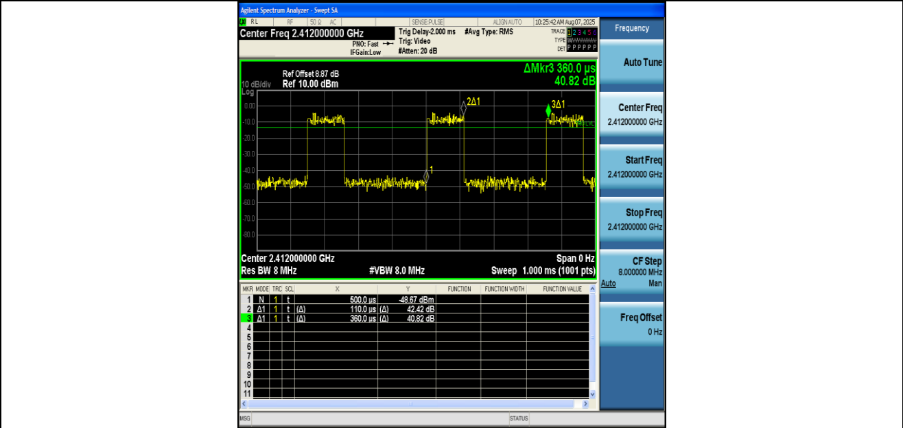
NTNV-11AX20MIMO-Ant2-2412
