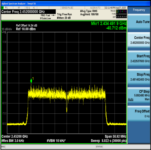
11AX40MIMO-Ant2-2452-PASS
