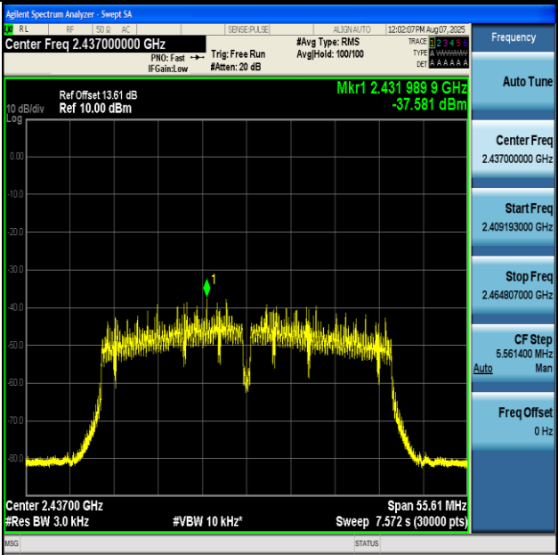
11N40MIMO-Ant1-2437-PASS
