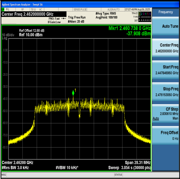
11N20MIMO-Ant1-2462-PASS
