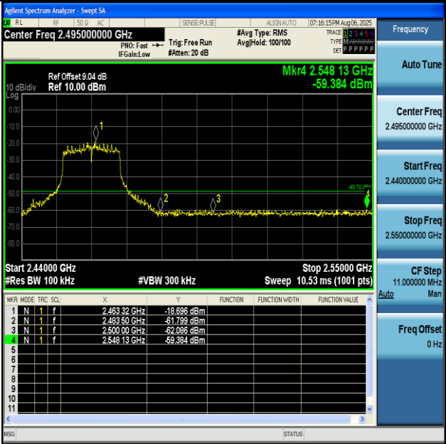
11N20MIMO-Ant2-2462-PASS
