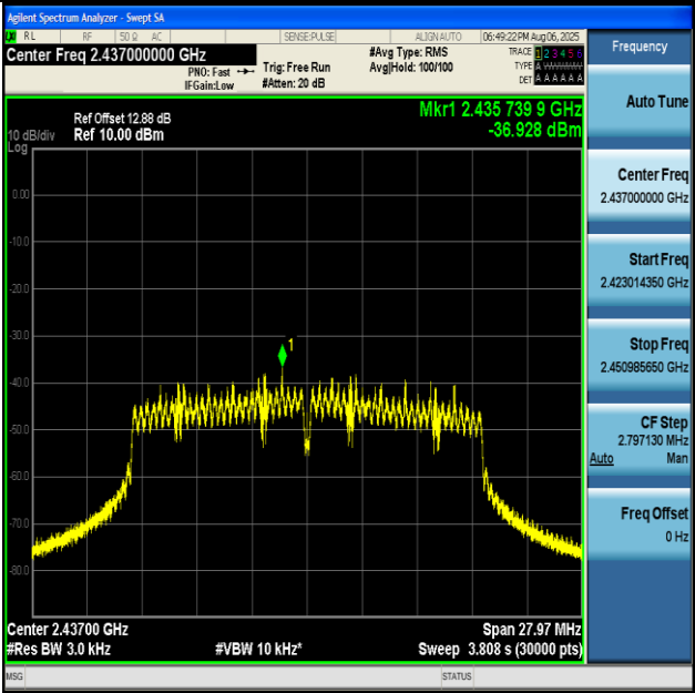
11N20MIMO-Ant1-2437-PASS
