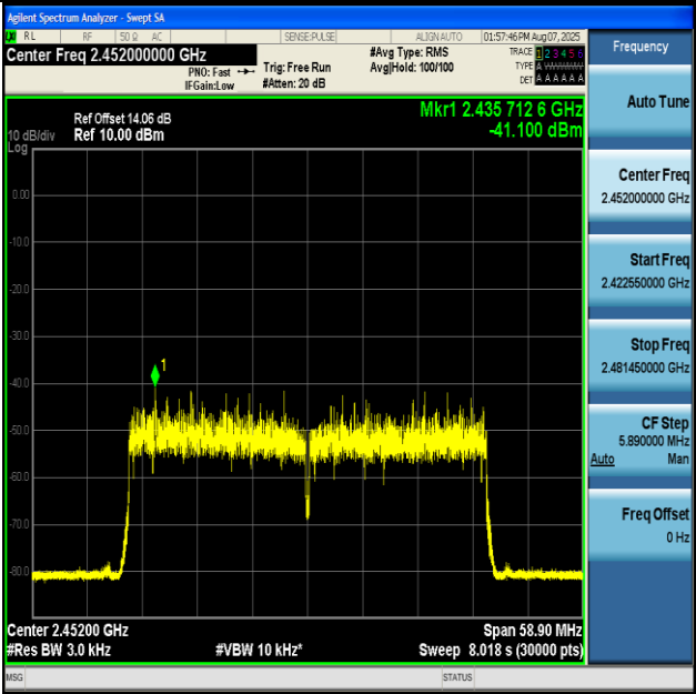
11AX40MIMO-Ant1-2452-PASS
