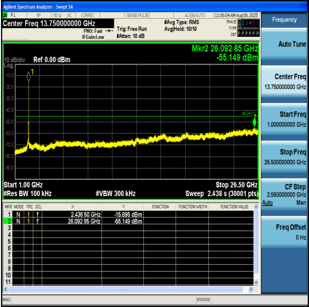
11G-Ant1-2437-1000~26500-PASS
