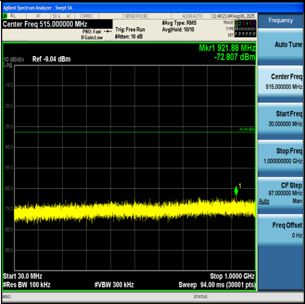
11B-Ant2-2437-30~1000-PASS
