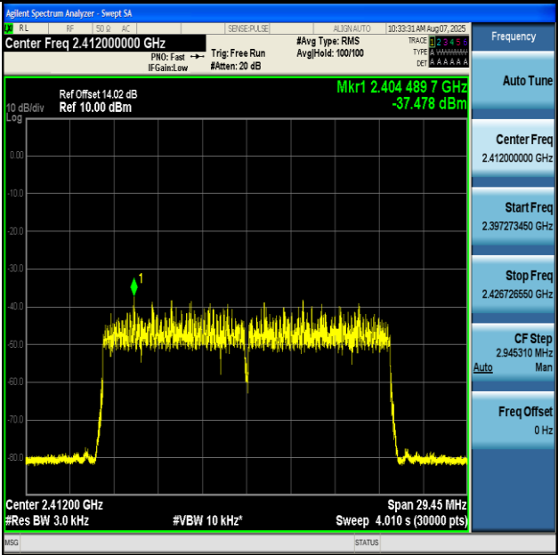
11AX20MIMO-Ant2-2412-PASS
