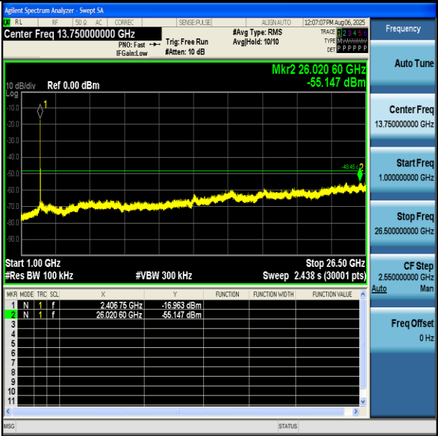
11G-Ant2-2412-1000~26500-PASS
