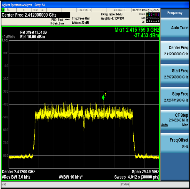
11AX20MIMO-Ant1-2412-PASS
