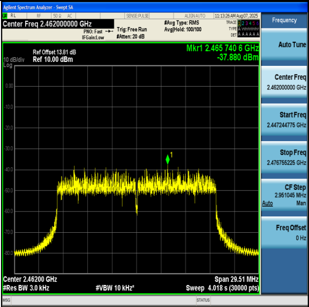
11AX20MIMO-Ant2-2462-PASS
