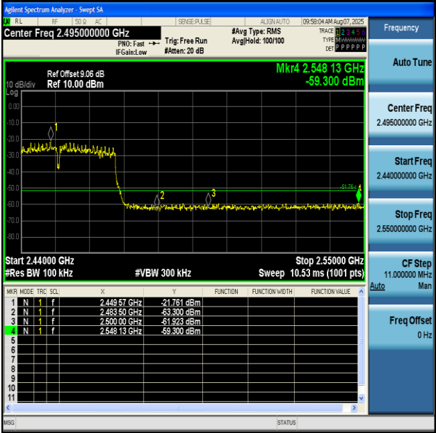
11N40MIMO-Ant1-2452-PASS
