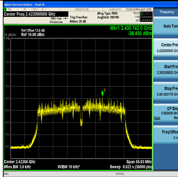
11AX40MIMO-Ant1-2422-PASS
