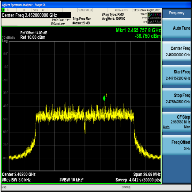
11AX20MIMO-Ant1-2462-PASS
