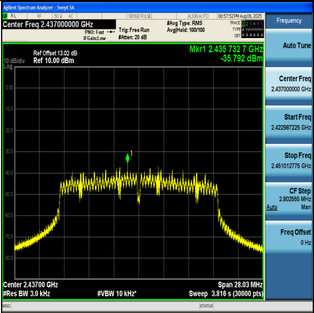
11N20MIMO-Ant2-2437-PASS
