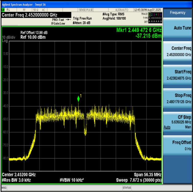
11N40MIMO-Ant2-2452-PASS
