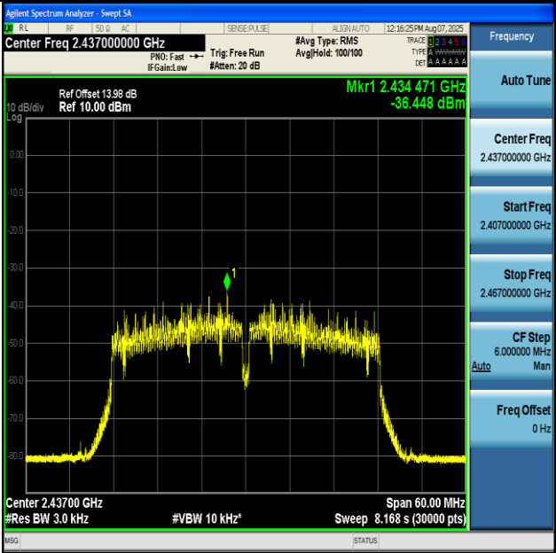
11N40MIMO-Ant2-2437-PASS
