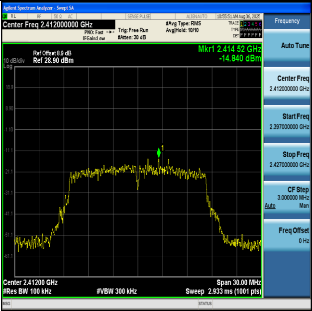
11G-Ant1-2412-0~Reference-PASS
