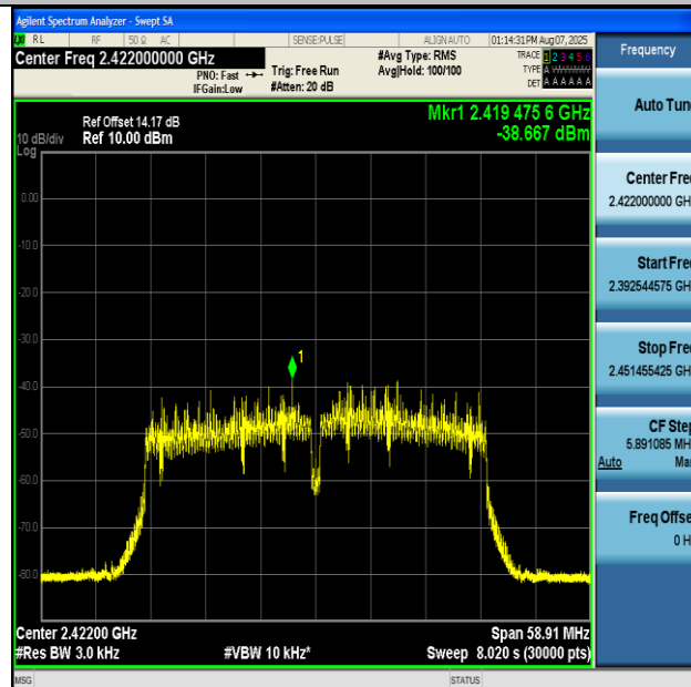
11AX40MIMO-Ant2-2422-PASS
