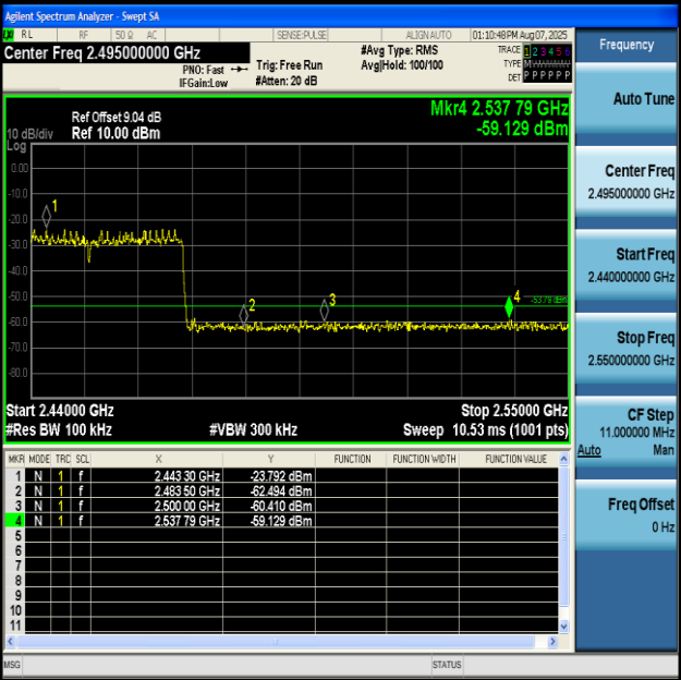
11AX40MIMO-Ant2-2452-PASS
