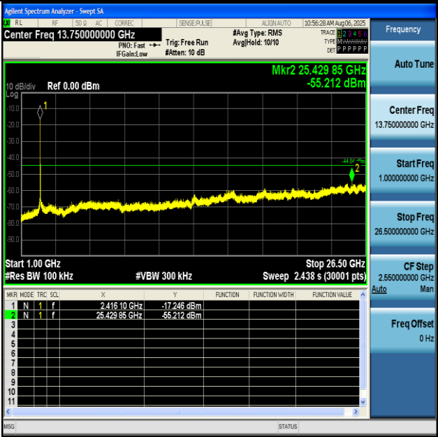
11G-Ant1-2412-1000~26500-PASS
