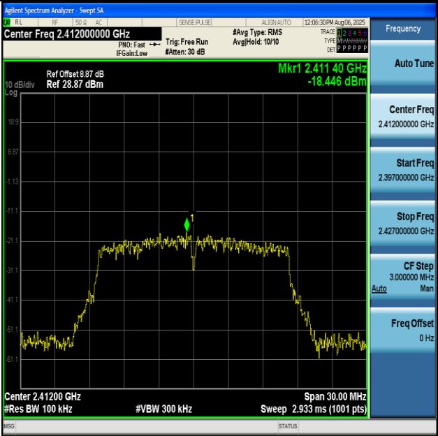
11G-Ant2-2412-0~Reference-PASS
