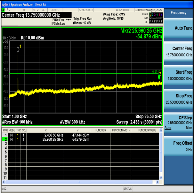
11G-Ant2-2437-1000~26500-PASS
