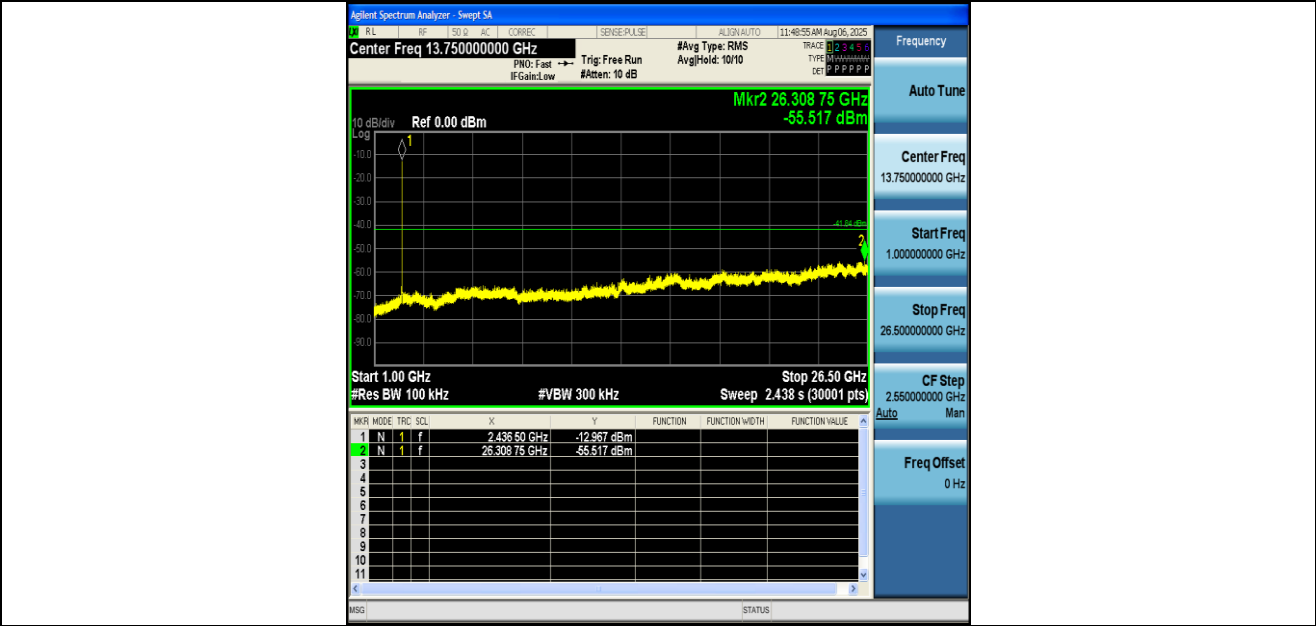
11B-Ant2-2437-1000~26500-PASS
