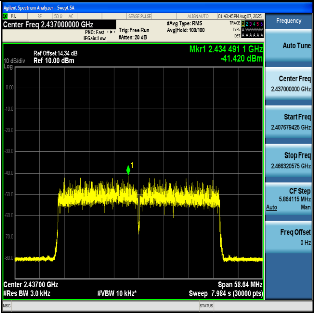
11AX40MIMO-Ant2-2437-PASS
