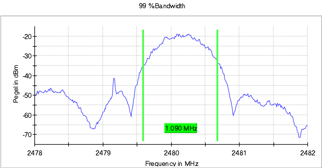
Transmission on 2480 MHz; + 85°C, 5 V DC
