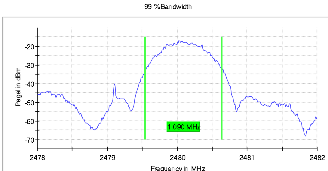
Transmission on 2480 MHz; - 40°C, 5 V DC
