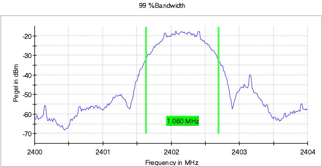
Transmission on 2402 MHz; + 85°C, 5 V DC
