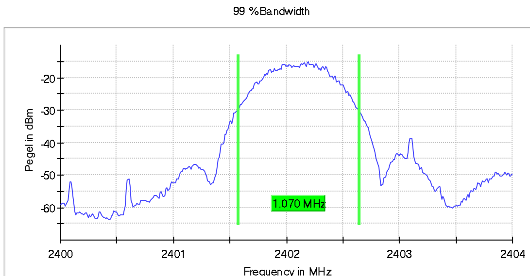
Transmission on 2402 MHz; - 40°C, 5 V DC
