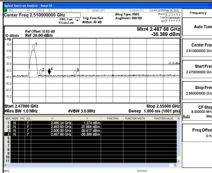
BLE_1M_Ant_High_2480_Peak
