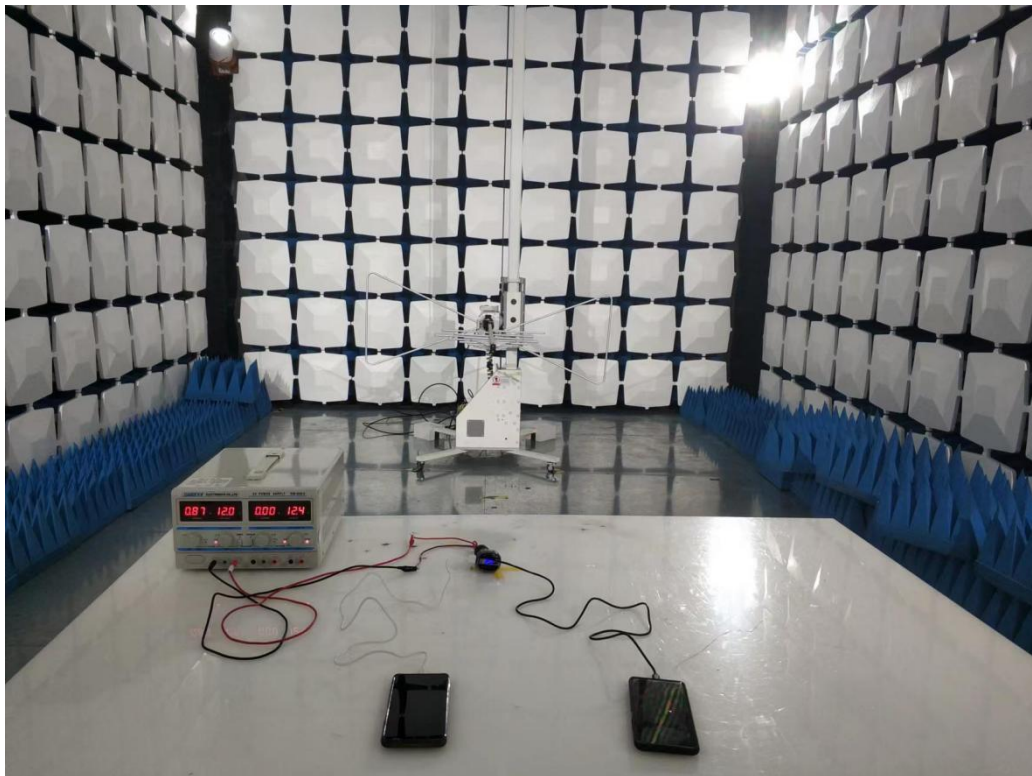
Blow 1GHz for radiated emission test setup
