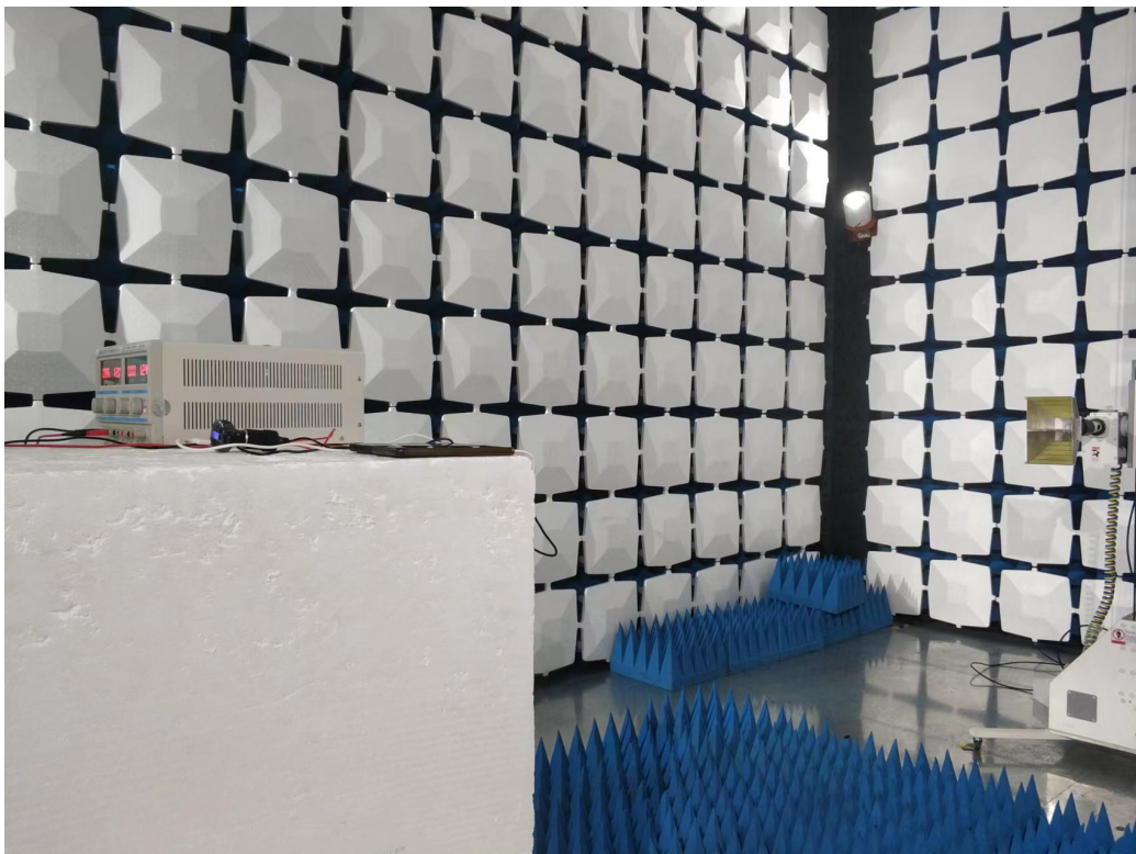
Above 1GHz for radiated emission test setup
