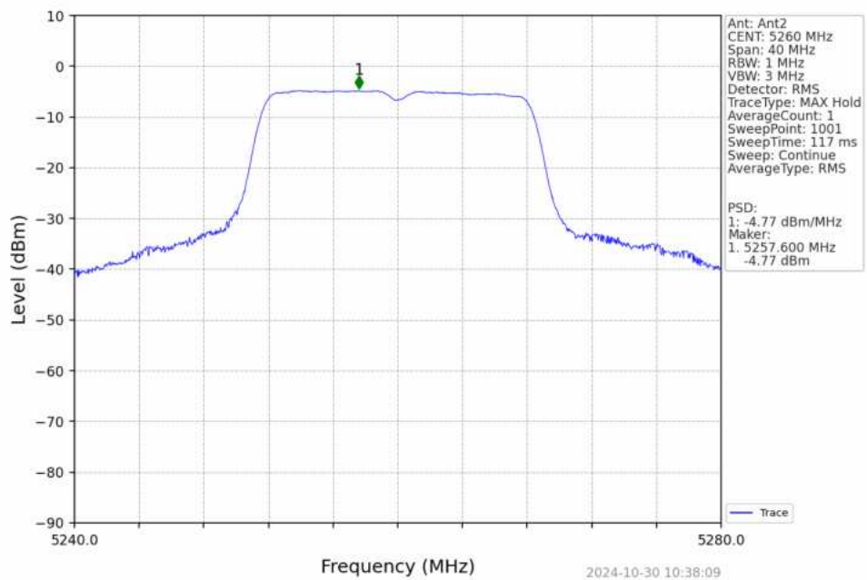
802.11a_LCH_5260MHz_Ant2_NTNV
