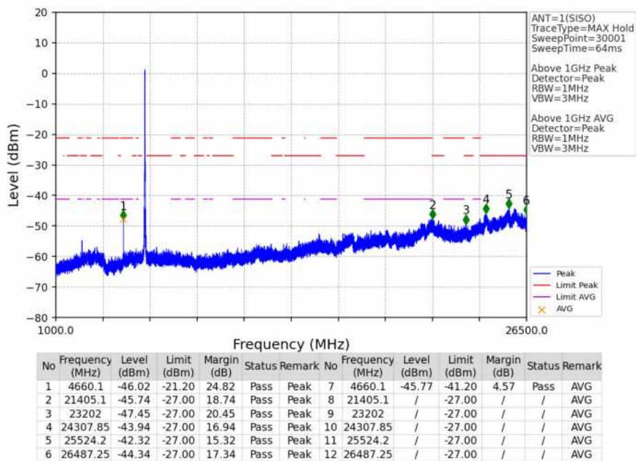
802.11a_HCH_5825MHz_Ant1_NTNV
