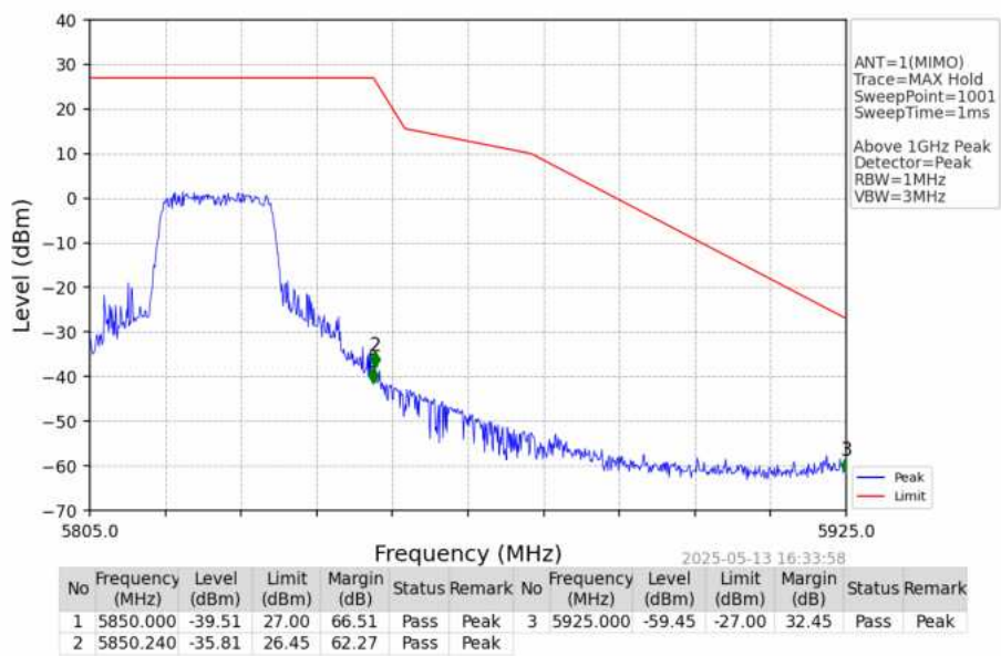
802.11ac(VHT20)_HCH_5825MHz_Ant1_NTNV
