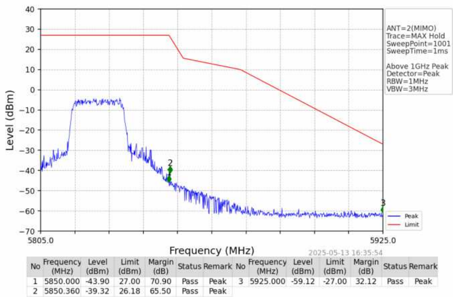
802.11ac(VHT20)_HCH_5825MHz_Ant2_NTNV
