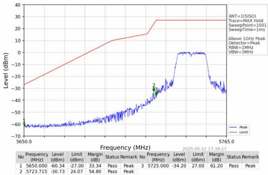
802.11a_LCH_5745MHz_Ant1_NTNV
