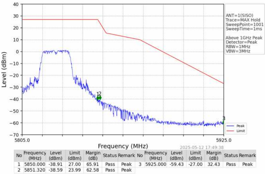
802.11a_HCH_5825MHz_Ant1_NTNV
