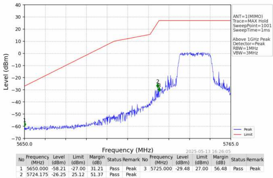
802.11ac(VHT20)_LCH_5745MHz_Ant1_NTNV
