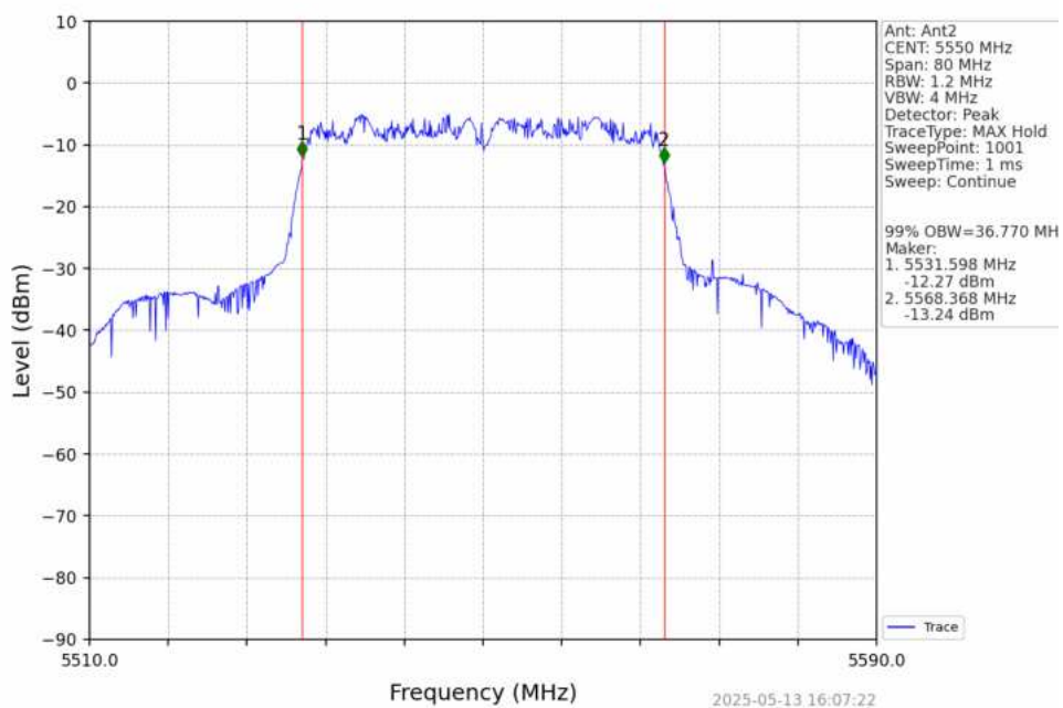
802.11ac(VHT40)_MCH_5550MHz_Ant2_NTNV
