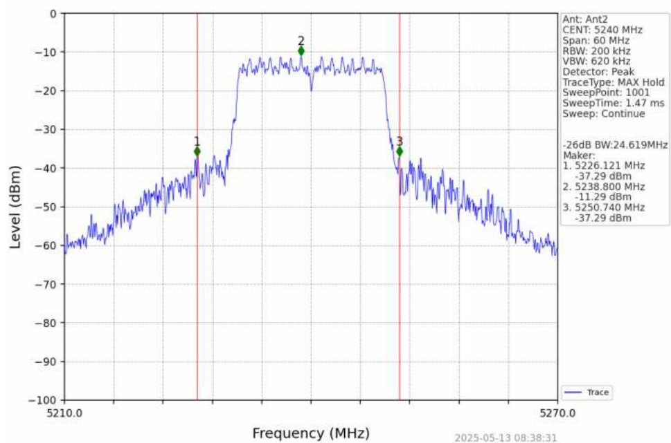
802.11n(HT20)_HCH_5240MHz_Ant2_NTNV
