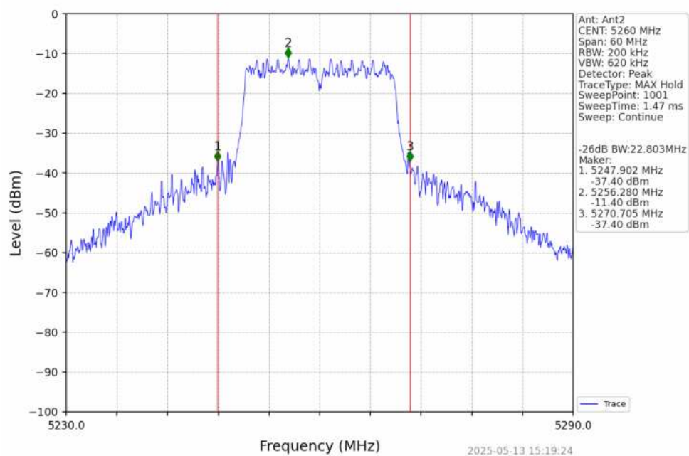
802.11ac(VHT20)_LCH_5260MHz_Ant2_NTNV
