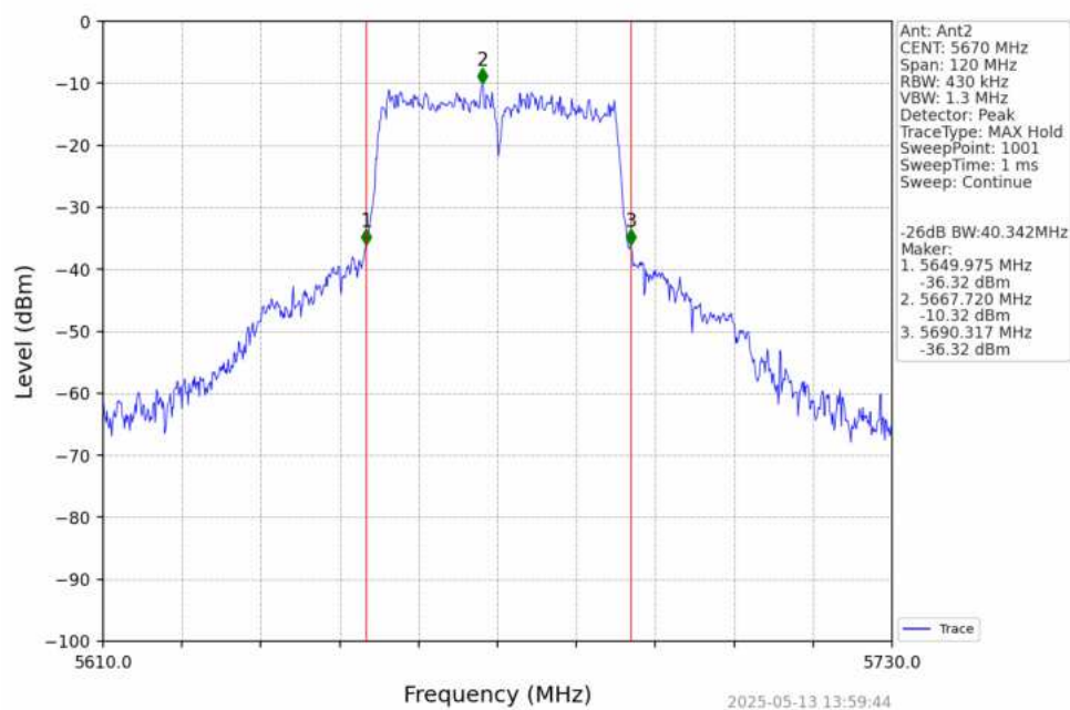
802.11n(HT40)_HCH_5670MHz_Ant2_NTNV
