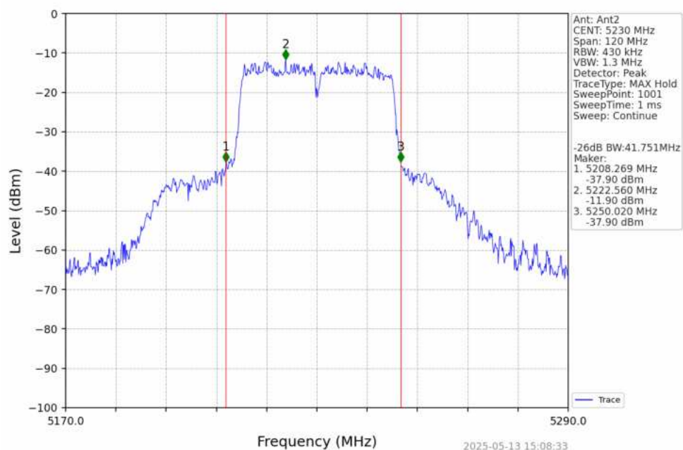
802.11ac(VHT40)_HCH_5230MHz_Ant2_NTNV
