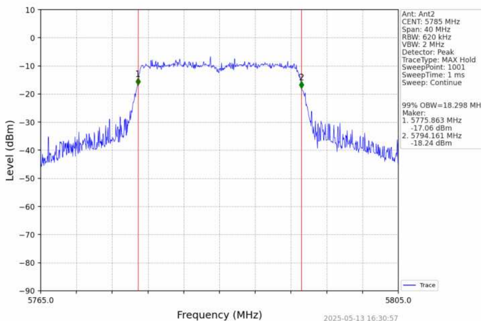
802.11ac(VHT20)_MCH_5785MHz_Ant2_NTNV
