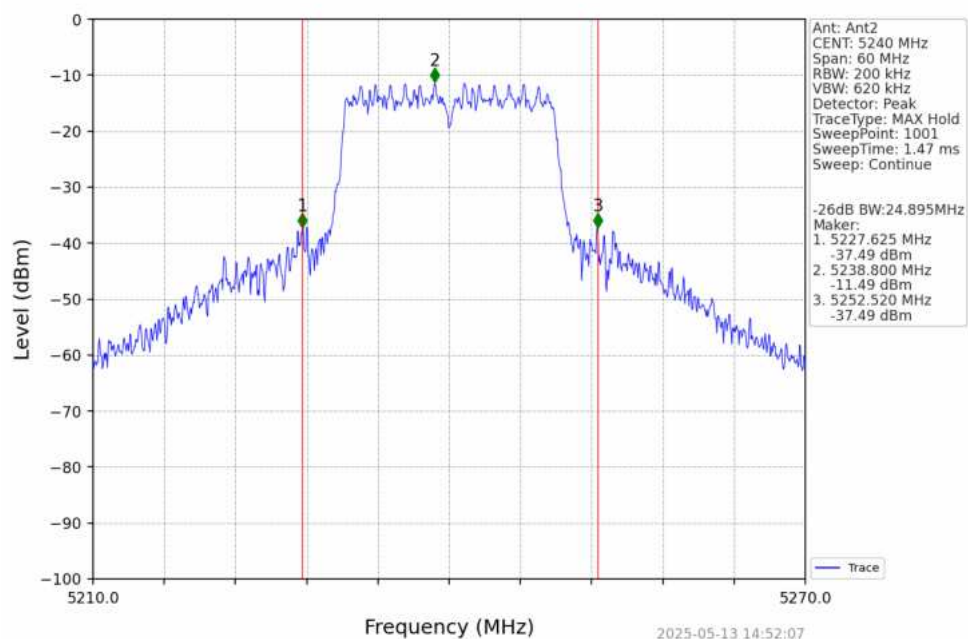
802.11ac(VHT20)_HCH_5240MHz_Ant2_NTNV
