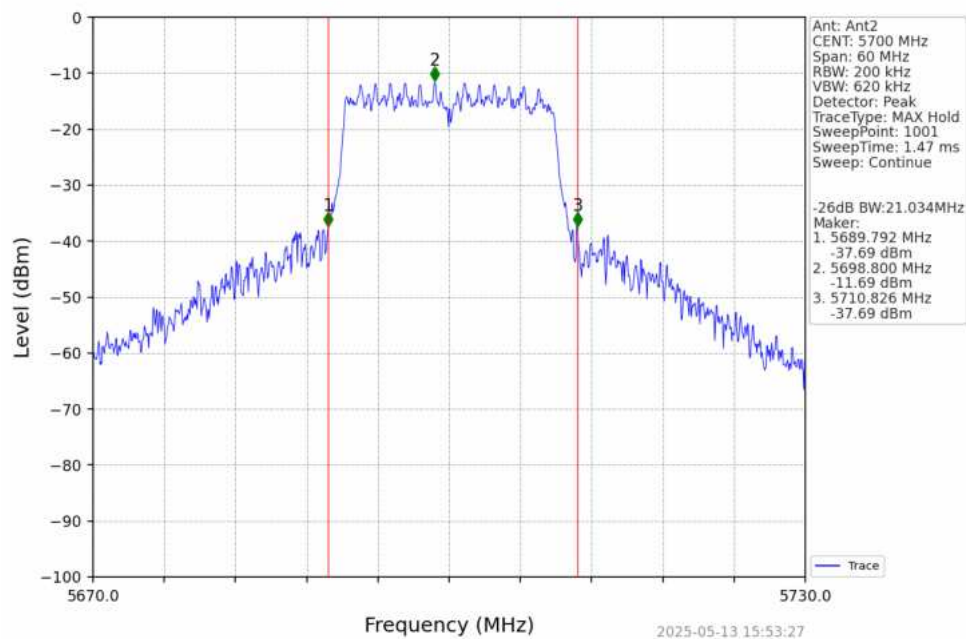
802.11ac(VHT20)_HCH_5700MHz_Ant2_NTNV
