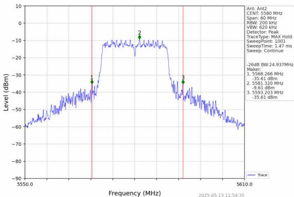
802.11n(HT20)_MCH_5580MHz_Ant2_NTNV
