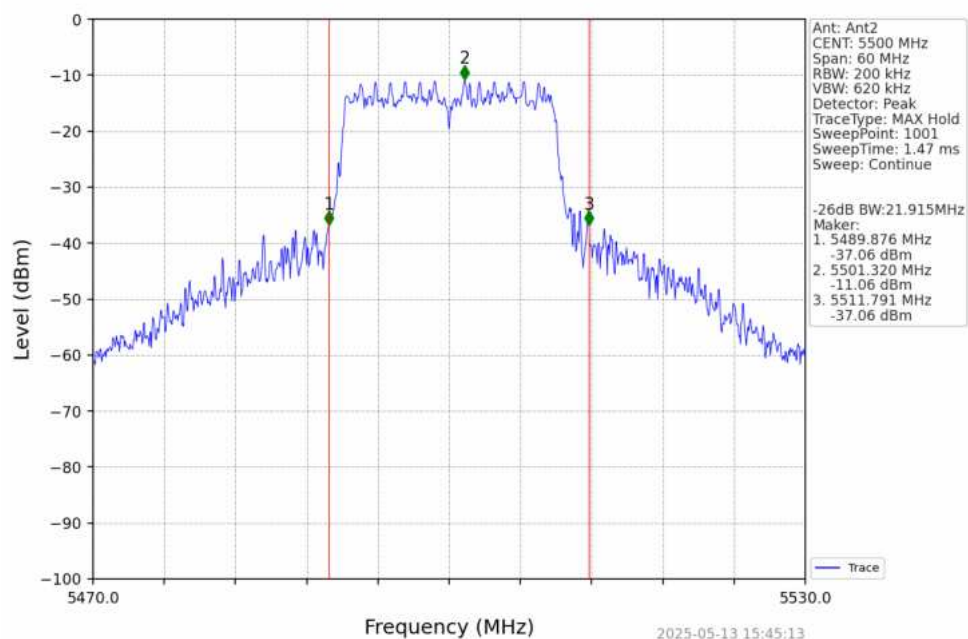
802.11ac(VHT20)_LCH_5500MHz_Ant2_NTNV
