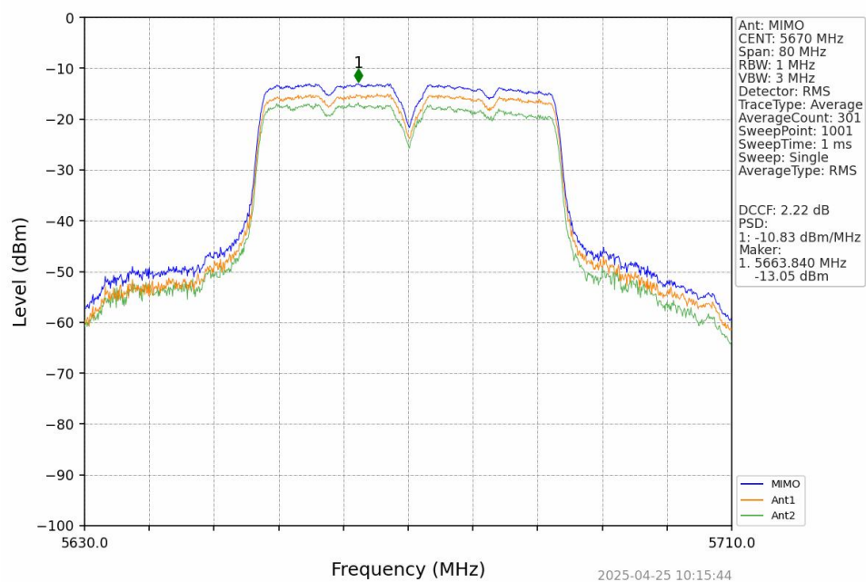
802.11ac(VHT40)_HCH_5670MHz_MIMO_NTNV
