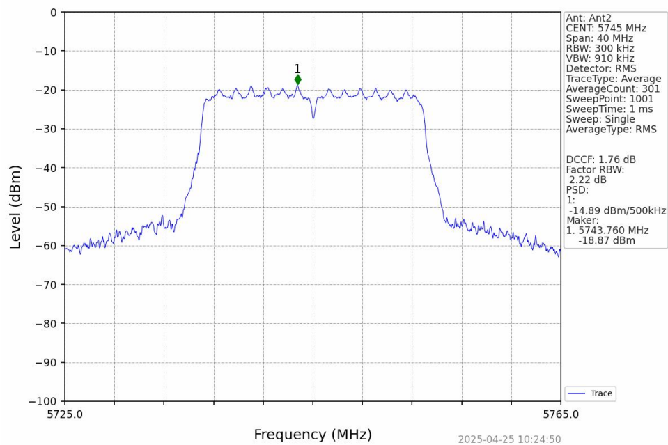
802.11ac(VHT20)_LCH_5745MHz_MIMO_NTNV
