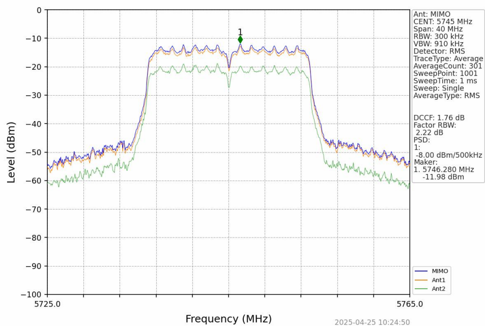
802.11ac(VHT20)_LCH_5745MHz_MIMO_NTNV
