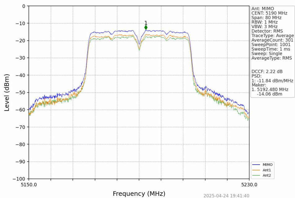
802.11ac(VHT40)_LCH_5190MHz_MIMO_NTNV
